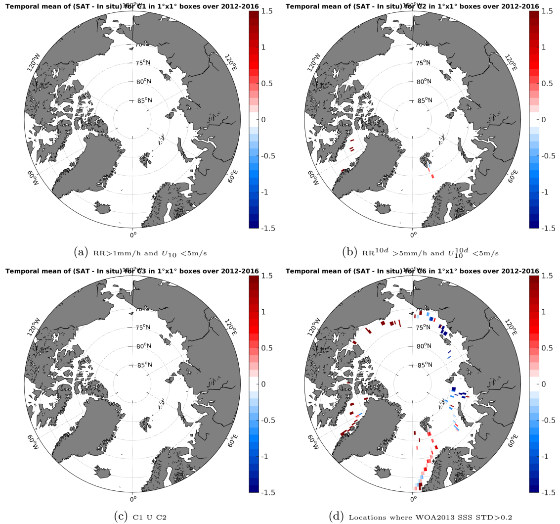
Figure 12: Temporal mean gridded over spatial boxes of size 1^\circ \times 1^\circ of \Delta SSS (SMOS-L3-CATDS-CECOS-LOCEAN-V2-9DAYS-25KM - TSG-GOSUD-Sailing-ship) for 4 different subdatasets corresponding to: RR > 1\text{mm/h} and U_{10} < 5\text{m/s} (a), RR^{10d} > 5\text{mm/h} and U_{10}^{10d} < 5\text{m/s} (b), C1 U C2 (c), Locations where WOA2013 SSS STD > 0.2 (d).
