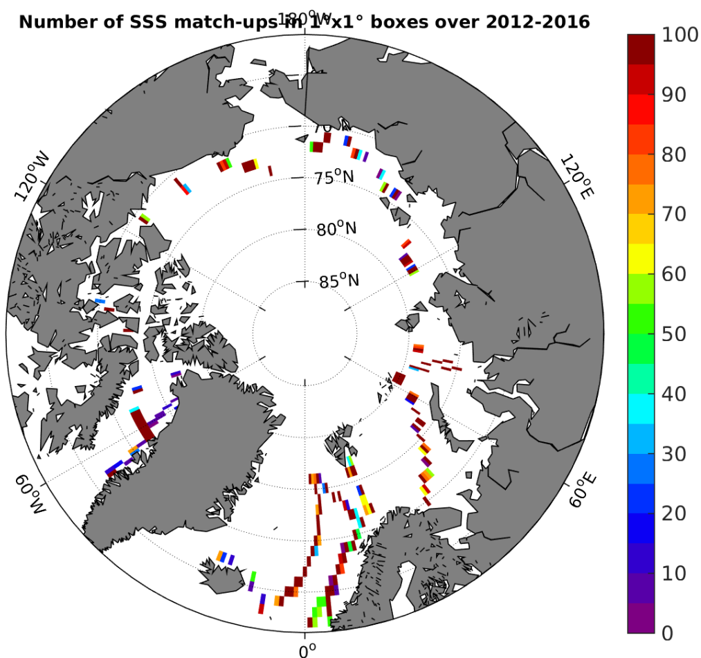
Figure 4: Number of SSS match-ups between TSG-GOSUD-Sailing-ship SSS and the SMOS-L3-CATDS-CECOS-LOCEAN-V2-9DAYS-25KM SSS product for the Arctic Ocean Pi-MEP region over 1°x1° boxes and for the full satellite product period.
