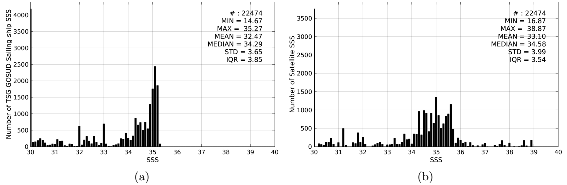
Figure 2: Histograms of SSS from TSG-GOSUD-Sailing-ship (a) and SMOS-L3-CATDS-CECOS-LOCEAN-V2-9DAYS-25KM (b) considering all match-up pairs per bins of 0.1 over the Arctic Ocean Pi-MEP region and for the full satellite product period.
