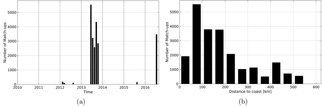
Figure 1: Number of match-ups between TSG-GOSUD-Sailing-ship and SMOS-L3-CATDS-CECOS-LOCEAN-V2-9DAYS-25KM SSS as a function of time (a) and as function of the distance to coast (b) over the Arctic Ocean Pi-MEP region and for the full satellite product period.
