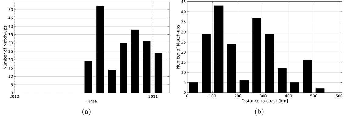
Figure 1: Number of match-ups between Sea mammals and SMOS-L3-CATDS-CECOS-LOCEAN-V2-9DAYS-25KM SSS as a function of time (a) and as function of the distance to coast (b) over the Arctic Ocean Pi-MEP region and for the full satellite product period.
