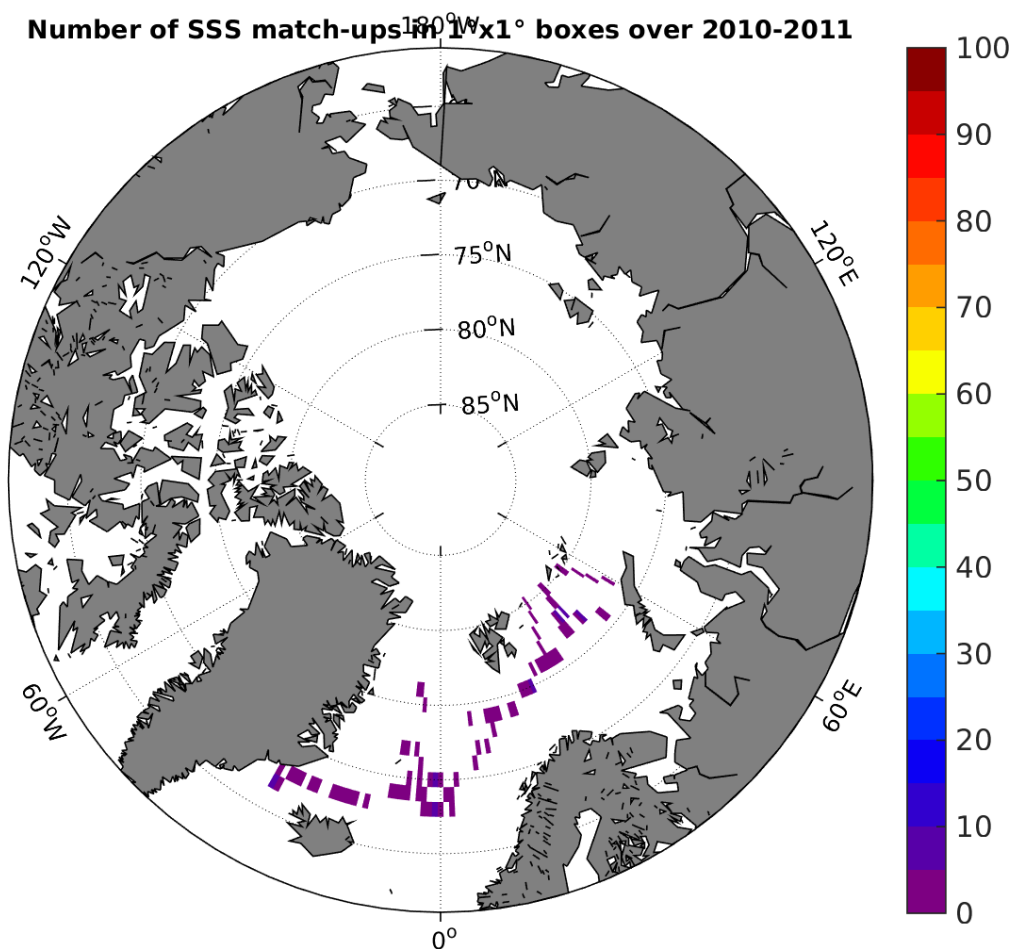
Figure 4: Number of SSS match-ups between Sea mammals SSS and the SMOS-L3-CATDS-CECOS-LOCEAN-V2-9DAYS-25KM SSS product for the Arctic Ocean Pi-MEP region over 1°x1° boxes and for the full satellite product period.
