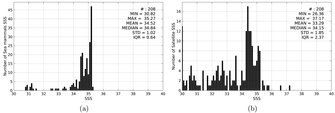
Figure 2: Histograms of SSS from Sea mammals (a) and SMOS-L3-CATDS-CECOS-LOCEAN-V2-9DAYS-25KM (b) considering all match-up pairs per bins of 0.1 over the Arctic Ocean Pi-MEP region and for the full satellite product period.
