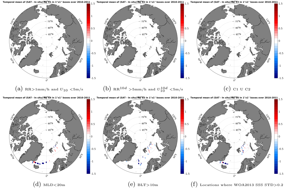
Figure 12: Temporal mean gridded over spatial boxes of size 1^\circ \times 1^\circ of \Delta SSS (SMOS-L3-CATDS-CECOS-LOCEAN-V2-9DAYS-25KM - Sea mammals) for 6 different subdatasets corresponding to: RR>1mm/h and U_{10} < 5\text{m/s} (a), RR^{10d} > 5\text{mm/h} and U_{10}^{10d} < 5\text{m/s} (b), C1 U C2 (c), MLD<20m (d), BLT>10m (e), Locations where WOA2013 SSS STD>0.2 (f).
