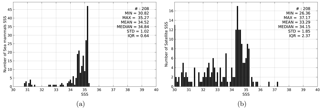
Figure 2: Histograms of SSS from Sea mammals (a) and SMOS-L3-CATDS-CECOS-LOCEAN-V2-9DAYS-25KM (b) considering all match-up pairs per bins of 0.1 over the Arctic Ocean Pi-MEP region and for the full satellite product period.
