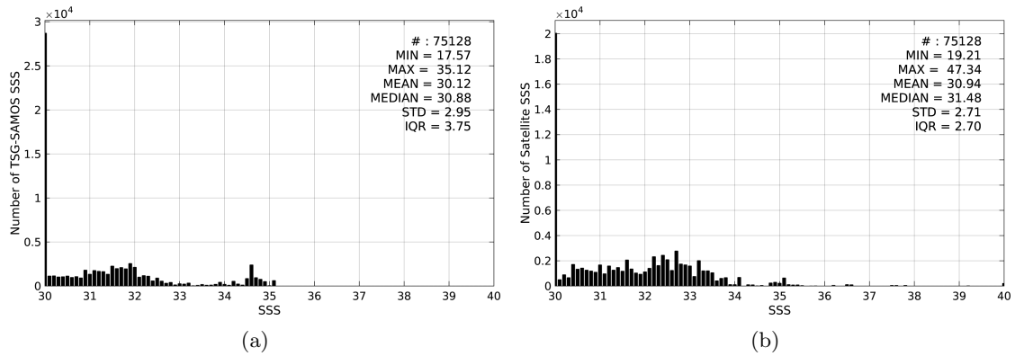
Figure 2: Histograms of SSS from TSG-SAMOS (a) and SMOS-L3-CATDS-CECOS-LOCEAN-V2-18DAYS-25KM (b) considering all match-up pairs per bins of 0.1 over the Arctic Ocean Pi-MEP region and for the full satellite product period.
