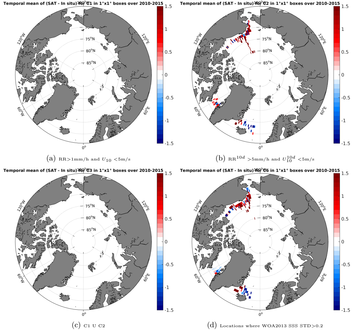
Figure 12: Temporal mean gridded over spatial boxes of size 1^\circ \times 1^\circ of \Delta SSS (SMOS-L3-CATDS-CECOS-LOCEAN-V2-18DAYS-25KM - TSG-SAMOS) for 4 different subdatasets corresponding to: RR > 1mm/h and U_{10} < 5\text{m/s} (a), RR^{10d} > 5\text{mm/h} and U_{10}^{10d} < 5\text{m/s} (b), C1 U C2 (c), Locations where WOA2013 SSS STD > 0.2 (d).
