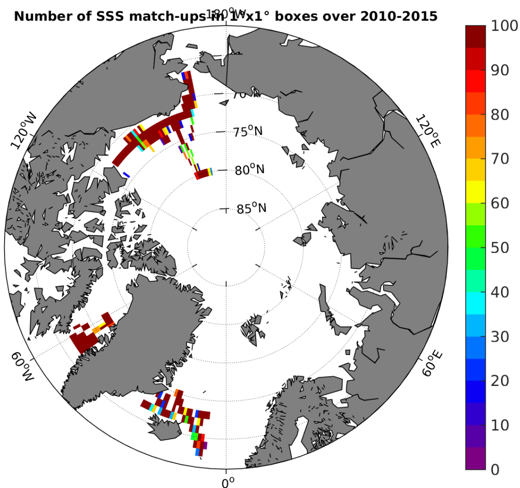
Figure 4: Number of SSS match-ups between TSG-SAMOS SSS and the SMOS-L3-CATDS-CECOS-LOCEAN-V2-18DAYS-25KM SSS product for the Arctic Ocean Pi-MEP region over 1^\circ \times 1^\circ boxes and for the full satellite product period.
