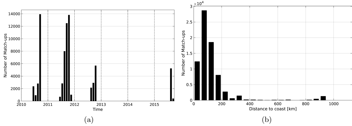
Figure 1: Number of match-ups between TSG-SAMOS and SMOS-L3-CATDS-CECOS-LOCEAN-V2-18DAYS-25KM SSS as a function of time (a) and as function of the distance to coast (b) over the Arctic Ocean Pi-MEP region and for the full satellite product period.
