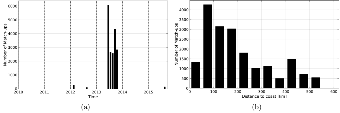
Figure 1: Number of match-ups between TSG-GOSUD-Sailing-ship and SMOS-L3-CATDS-CECOS-LOCEAN-V2-18DAYS-25KM SSS as a function of time (a) and as function of the distance to coast (b) over the Arctic Ocean Pi-MEP region and for the full satellite product period.
