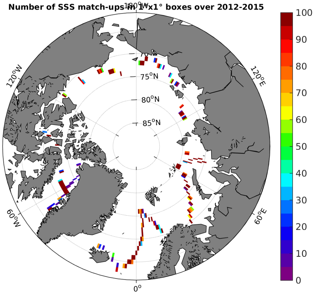
Figure 4: Number of SSS match-ups between TSG-GOSUD-Sailing-ship SSS and the SMOS-L3-CATDS-CECOS-LOCEAN-V2-18DAYS-25KM SSS product for the Arctic Ocean Pi-MEP region over 1°x1° boxes and for the full satellite product period.
