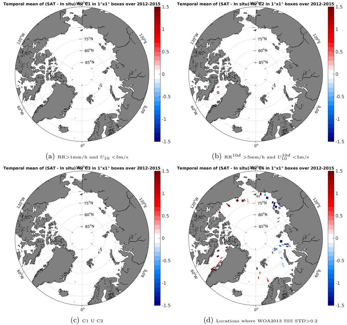
Figure 12: Temporal mean gridded over spatial boxes of size 1^\circ \times 1^\circ of \Delta SSS (SMOS-L3-CATDS-CECOS-LOCEAN-V2-18DAYS-25KM - TSG-GOSUD-Sailing-ship) for 4 different subdatasets corresponding to: RR > 1\text{mm/h} and U_{10} < 5\text{m/s} (a), RR^{10d} > 5\text{mm/h} and U_{10}^{10d} < 5\text{m/s} (b), C1 U C2 (c), Locations where WOA2013 SSS STD > 0.2 (d).
