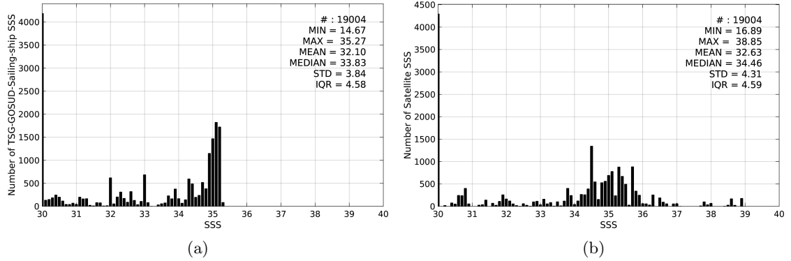
Figure 2: Histograms of SSS from TSG-GOSUD-Sailing-ship (a) and SMOS-L3-CATDS-CECOS-LOCEAN-V2-18DAYS-25KM (b) considering all match-up pairs per bins of 0.1 over the Arctic Ocean Pi-MEP region and for the full satellite product period.
