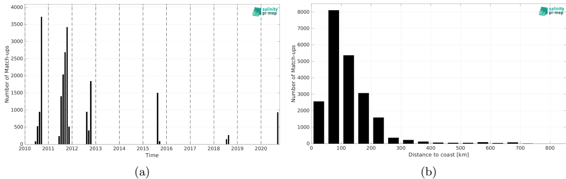
Figure 2: Number of match-ups between TSG (SAMOS) and SMOS SSS L3 Arctic v2 - 9 Days (CATDS-CEC-LOCEAN) SSS as a function of time (a) and as function of the distance to coast (b) over the Arctic Ocean Pi-MEP region and for the full satellite product period.
