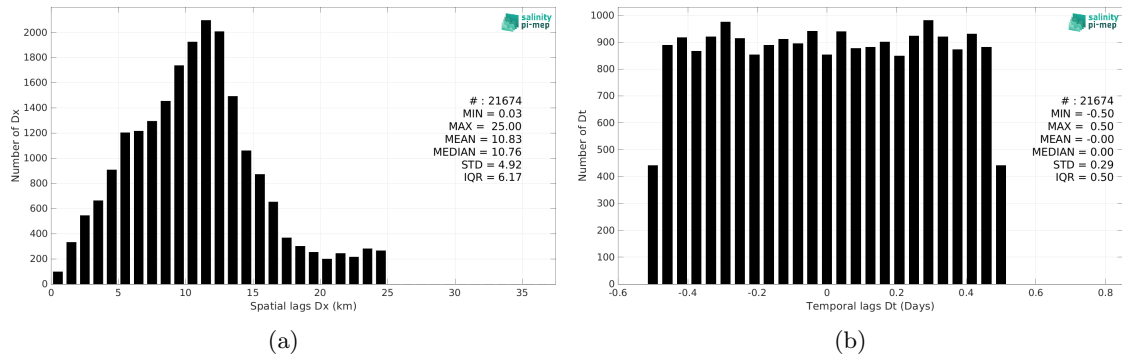
Figure 6: Histograms of the spatial (a) and temporal (b) lags between the location/time of the TSG (SAMOS) measurement and the date of the corresponding SMOS SSS L3 Arctic v2 - 9 Days (CATDS-CEC-LOCEAN) SSS pixel.
