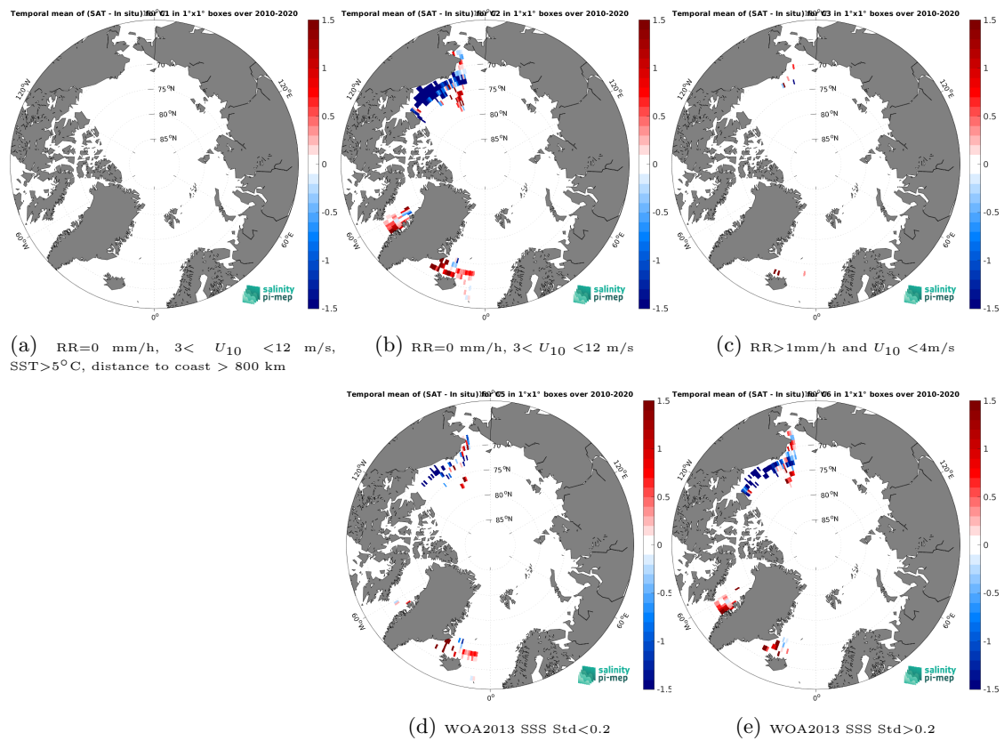
Figure 14: Temporal mean gridded over spatial boxes of size 1^\circ \times 1^\circ of \Delta\text{SSS} (SMOS SSS L3 Arctic v2 - 9 Days (CATDS-CEC-LOCEAN) - TSG (SAMOS)) for 5 different subdatasets corresponding to: RR=0 mm/h, 3 < U_{10} < 12 m/s, SST > 5°C, distance to coast > 800 km (a), RR=0 mm/h, 3 < U_{10} < 12 m/s (b), RR > 1mm/h and U_{10} < 4 m/s (c), WOA2013 SSS Std < 0.2 (d), WOA2013 SSS Std > 0.2 (e).
