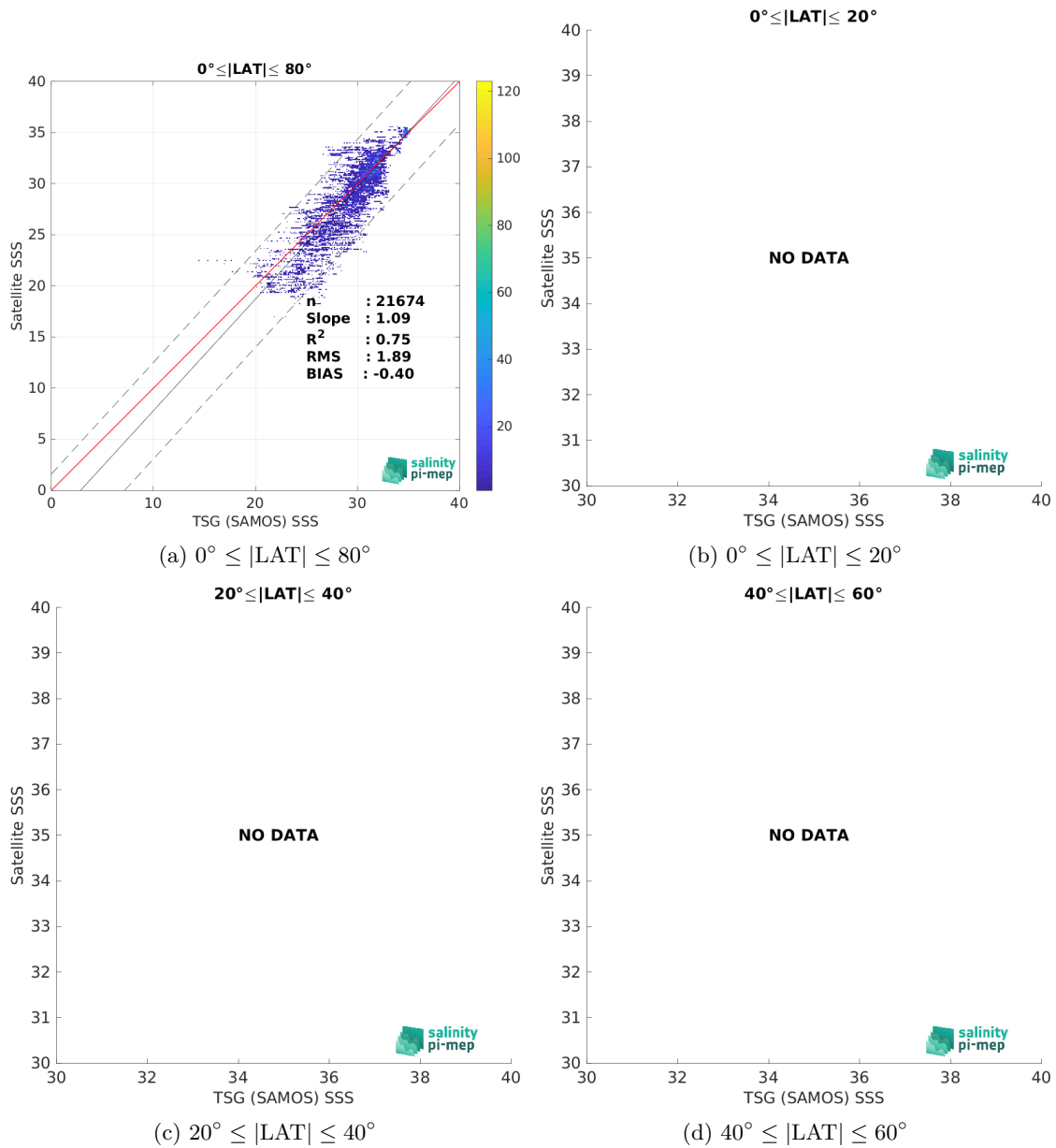
Figure 10: Contour maps of the concentration of SMOS SSS L3 Arctic v2 - 9 Days (CATDS-CEC-LOCEAN) SSS (y-axis) versus TSG (SAMOS) SSS (x-axis) at match-up pairs for different latitude bands. For each plot, the red line shows x=y . The black thin and dashed lines indicate a linear fit through the data cloud and the \pm 95\% confidence levels, respectively. The number match-up pairs n , the slope and R^2 coefficient of the linear fit, the root mean square (RMS) and the mean bias between satellite and in situ data are indicated for each latitude band in each plots.
