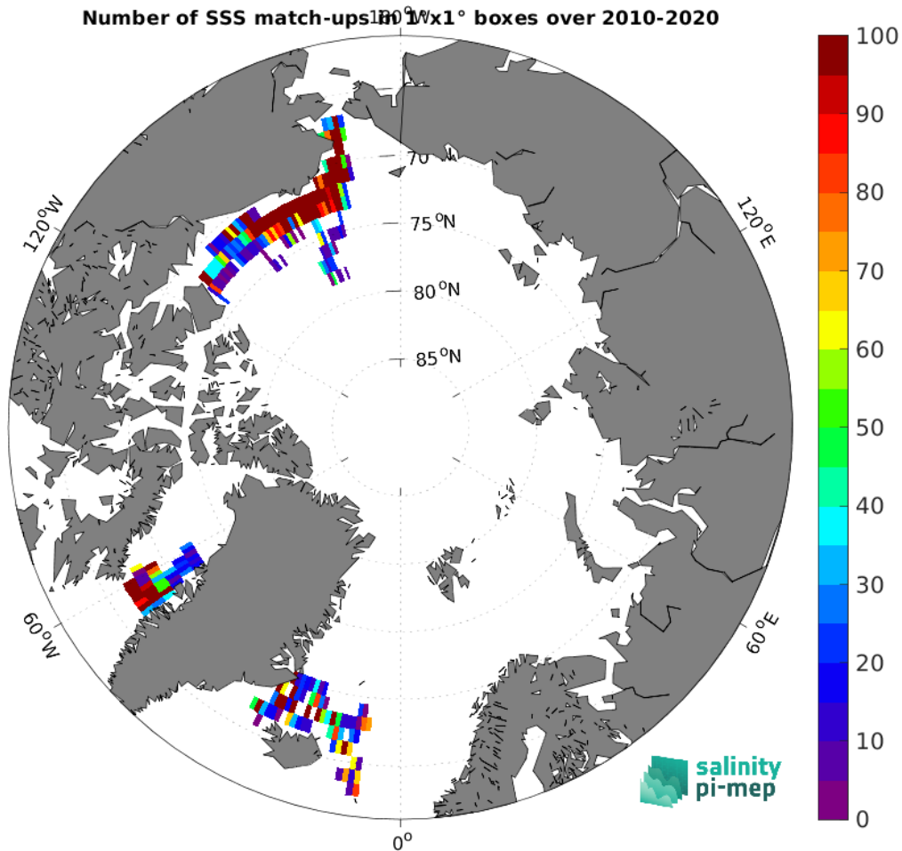
Figure 5: Number of SSS match-ups between TSG (SAMOS) SSS and the SMOS SSS L3 Arctic v2 - 9 Days (CATDS-CEC-LOCEAN) SSS product for the Arctic Ocean Pi-MEP region over 1^\circ \times 1^\circ boxes and for the full satellite product period.
