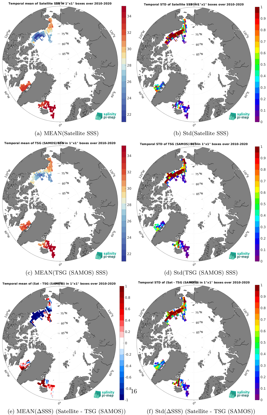
Figure 7: Temporal mean (left) and Std (right) of SSS from SMOS SSS L3 Arctic v2 - 9 Days (CATDS-CEC-LOCEAN) (top), TSG (SAMOS) (middle), and of \Delta SSS (Satellite - TSG (SAMOS)). Only match-up pairs are used to generate these maps.
