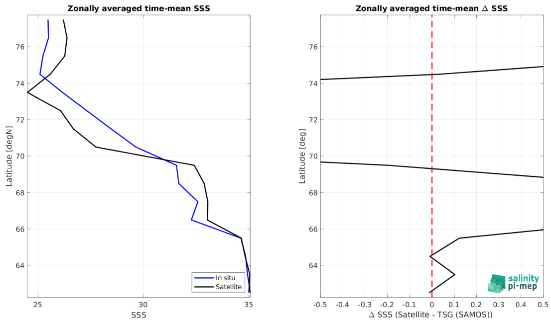
Figure 9: Left panel: Zonal mean SSS from SMOS SSS L3 Arctic v2 - 9 Days (CATDS-CEC-LOCEAN) satellite product (black) and from TSG (SAMOS) (blue). Right panel: Zonal mean of \Delta SSS (Satellite - TSG (SAMOS)) for all the collected Pi-MEP match-up pairs estimated over the full satellite product period.
