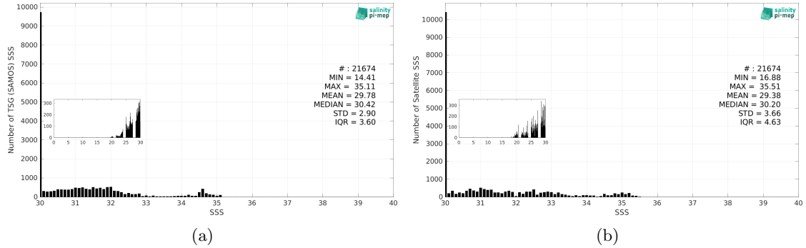
Figure 3: Histograms of SSS from TSG (SAMOS) (a) and SMOS SSS L3 Arctic v2 - 9 Days (CATDS-CEC-LOCEAN) (b) considering all match-up pairs per bins of 0.1 over the Arctic Ocean Pi-MEP region and for the full satellite product period.
