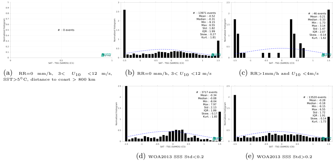
Figure 15: Normalized histogram of \Delta SSS (SMOS SSS L3 Arctic v2 - 9 Days (CATDS-CEC-LOCEAN) - TSG (SAMOS)) for 5 different subdatasets corresponding to: RR=0 mm/h, 3 < U_{10} < 12 m/s, SST > 5°C, distance to coast > 800 km (a), RR=0 mm/h, 3 < U_{10} < 12 m/s (b), RR > 1mm/h and U_{10} < 4 m/s (c), WOA2013 SSS Std < 0.2 (d), WOA2013 SSS Std > 0.2 (e).
