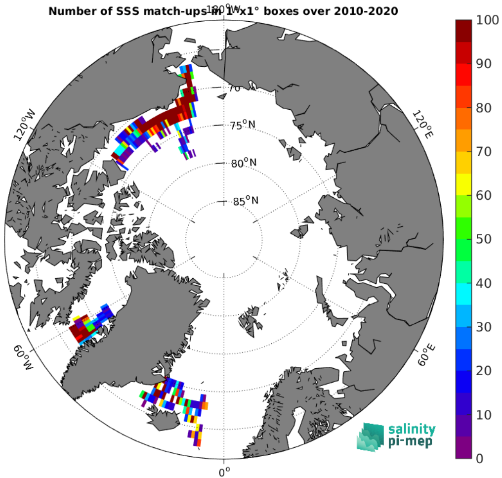
Figure 4: Number of SSS match-ups between TSG (SAMOS) SSS and the SMOS SSS L3 Arctic v2 - 9 Days (CATDS-CEC-LOCEAN) SSS product for the Arctic Ocean Pi-MEP region over 1^\circ \times 1^\circ boxes and for the full satellite product period.
