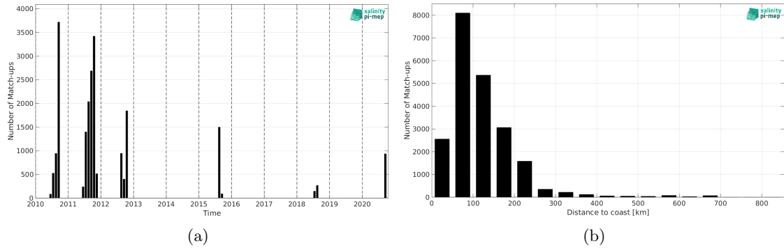
Figure 1: Number of match-ups between TSG (SAMOS) and SMOS SSS L3 Arctic v2 - 9 Days (CATDS-CEC-LOCEAN) SSS as a function of time (a) and as function of the distance to coast (b) over the Arctic Ocean Pi-MEP region and for the full satellite product period.
