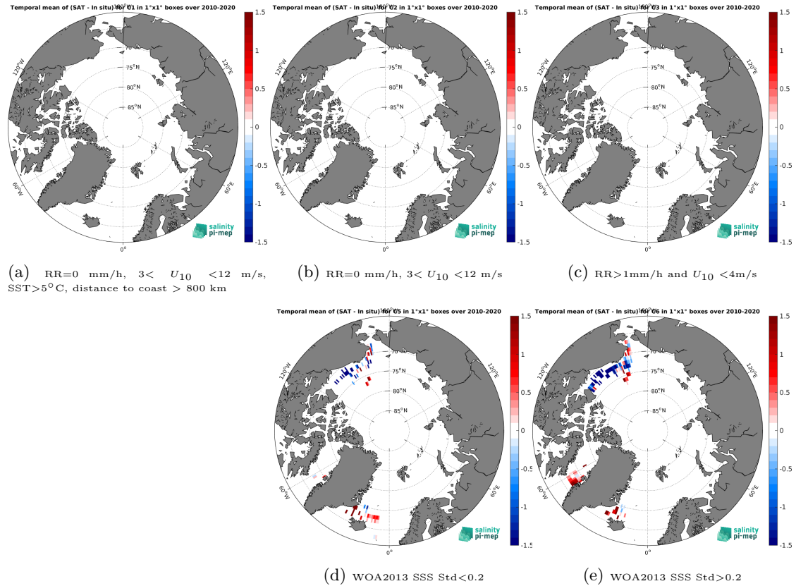
Figure 12: Temporal mean gridded over spatial boxes of size 1^{\circ}\times 1^{\circ} of \Delta\text{SSS} (SMOS SSS L3 Arctic v2 - 9 Days (CATDS-CEC-LOCEAN) - TSG (SAMOS)) for 5 different subdatasets corresponding to:RR=0 mm/h, 3 < U_{10} < 12 m/s, SST >5^{\circ}\text{C} , distance to coast > 800 km (a), RR=0 mm/h, 3 < U_{10} < 12 m/s (b), RR >1 mm/h and U_{10} < 4 m/s (c), WOA2013 SSS Std <0.2 (d), WOA2013 SSS Std >0.2 (e).
