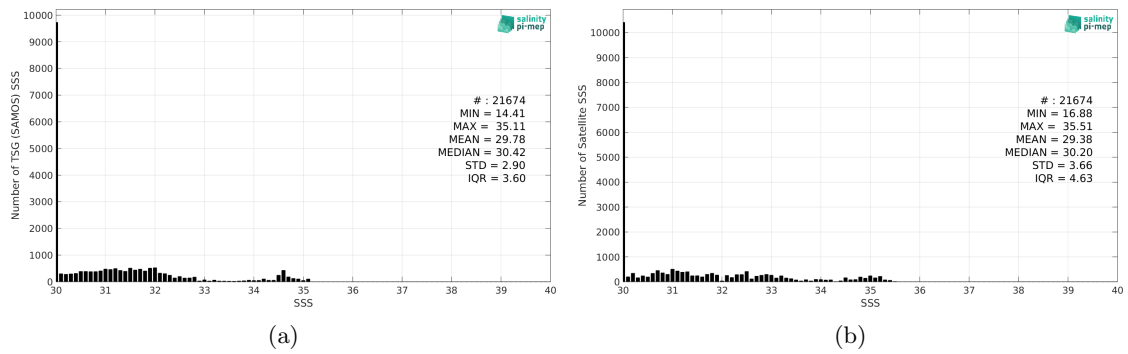
Figure 2: Histograms of SSS from TSG (SAMOS) (a) and SMOS SSS L3 Arctic v2 - 9 Days (CATDS-CEC-LOCEAN) (b) considering all match-up pairs per bins of 0.1 over the Arctic Ocean Pi-MEP region and for the full satellite product period.
