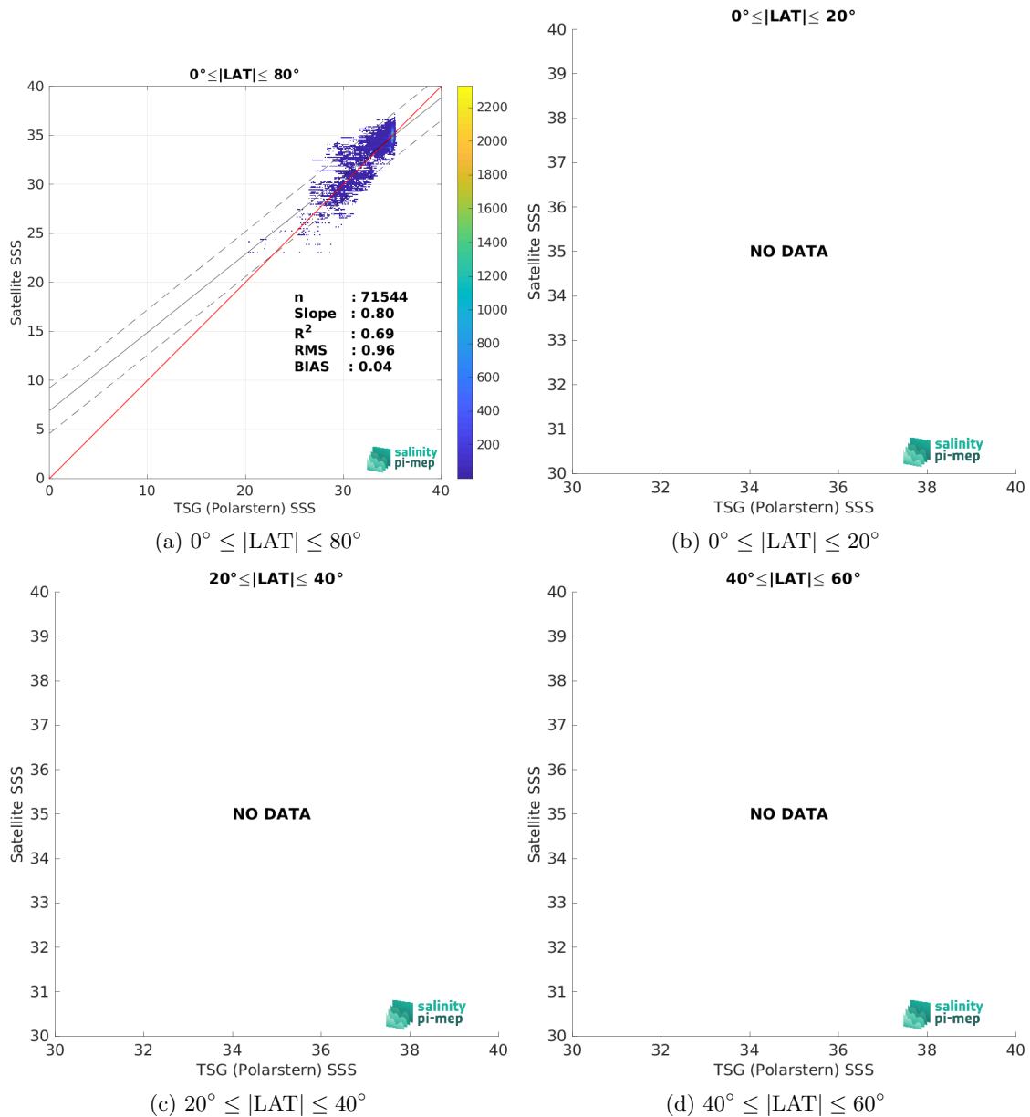
Figure 10: Contour maps of the concentration of SMOS SSS L3 Arctic v2 - 9 Days (CATDS-CEC-LOCEAN) SSS (y-axis) versus TSG (Polarstern) SSS (x-axis) at match-up pairs for different latitude bands. For each plot, the red line shows x=y . The black thin and dashed lines indicate a linear fit through the data cloud and the \pm 95\% confidence levels, respectively. The number match-up pairs n , the slope and R^2 coefficient of the linear fit, the root mean square (RMS) and the mean bias between satellite and in situ data are indicated for each latitude band in each plots.
