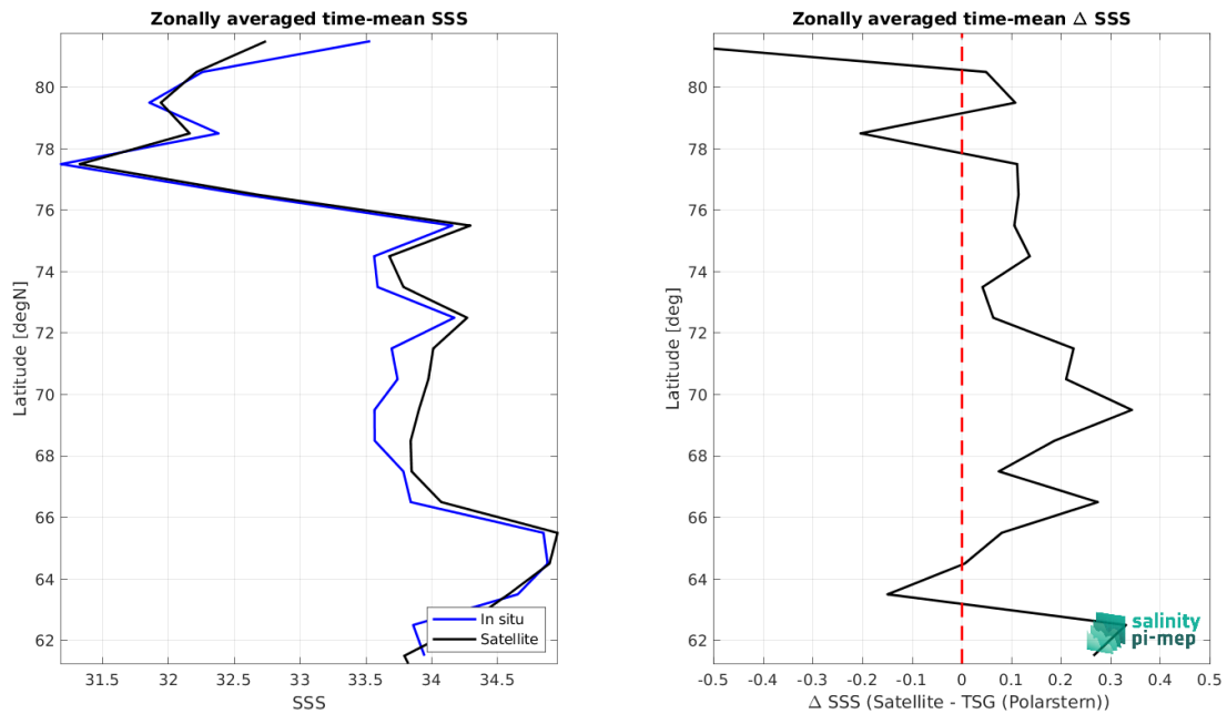
Figure 9: Left panel: Zonal mean SSS from SMOS SSS L3 Arctic v2 - 9 Days (CATDS-CEC-LOCEAN) satellite product (black) and from TSG (Polarstern) (blue). Right panel: Zonal mean of \Delta SSS (Satellite - TSG (Polarstern)) for all the collected Pi-MEP match-up pairs estimated over the full satellite product period.
