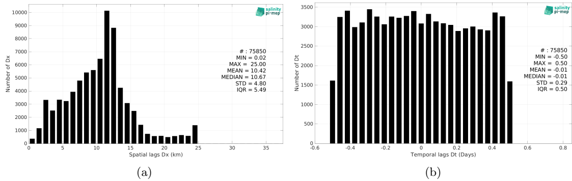
Figure 6: Histograms of the spatial (a) and temporal (b) lags between the location/time of the TSG (Polarstern) measurement and the date of the corresponding SMOS SSS L3 Arctic v2 - 9 Days (CATDS-CEC-LOCEAN) SSS pixel.
