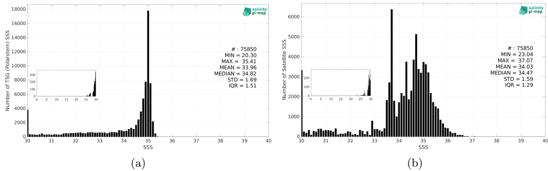
Figure 3: Histograms of SSS from TSG (Polarstern) (a) and SMOS SSS L3 Arctic v2 - 9 Days (CATDS-CEC-LOCEAN) (b) considering all match-up pairs per bins of 0.1 over the Arctic Ocean Pi-MEP region and for the full satellite product period.
