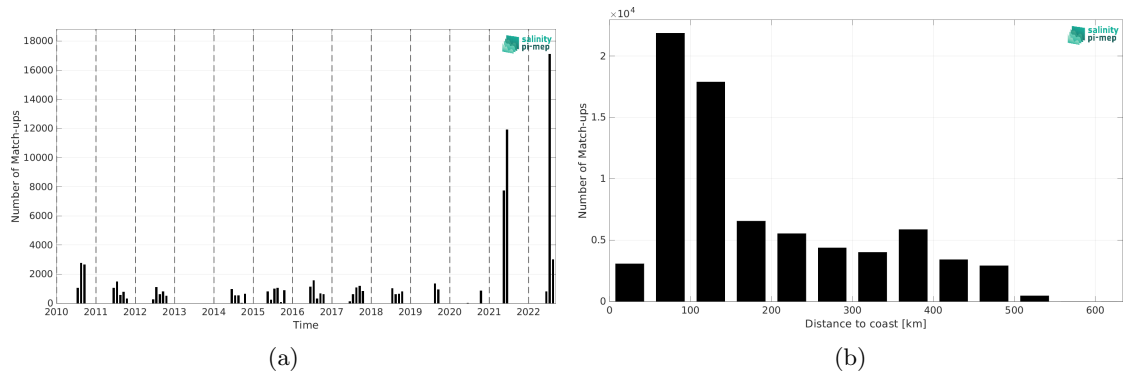
Figure 2: Number of match-ups between TSG (Polarstern) and SMOS SSS L3 Arctic v2 - 9 Days (CATDS-CEC-LOCEAN) SSS as a function of time (a) and as function of the distance to coast (b) over the Arctic Ocean Pi-MEP region and for the full satellite product period.
