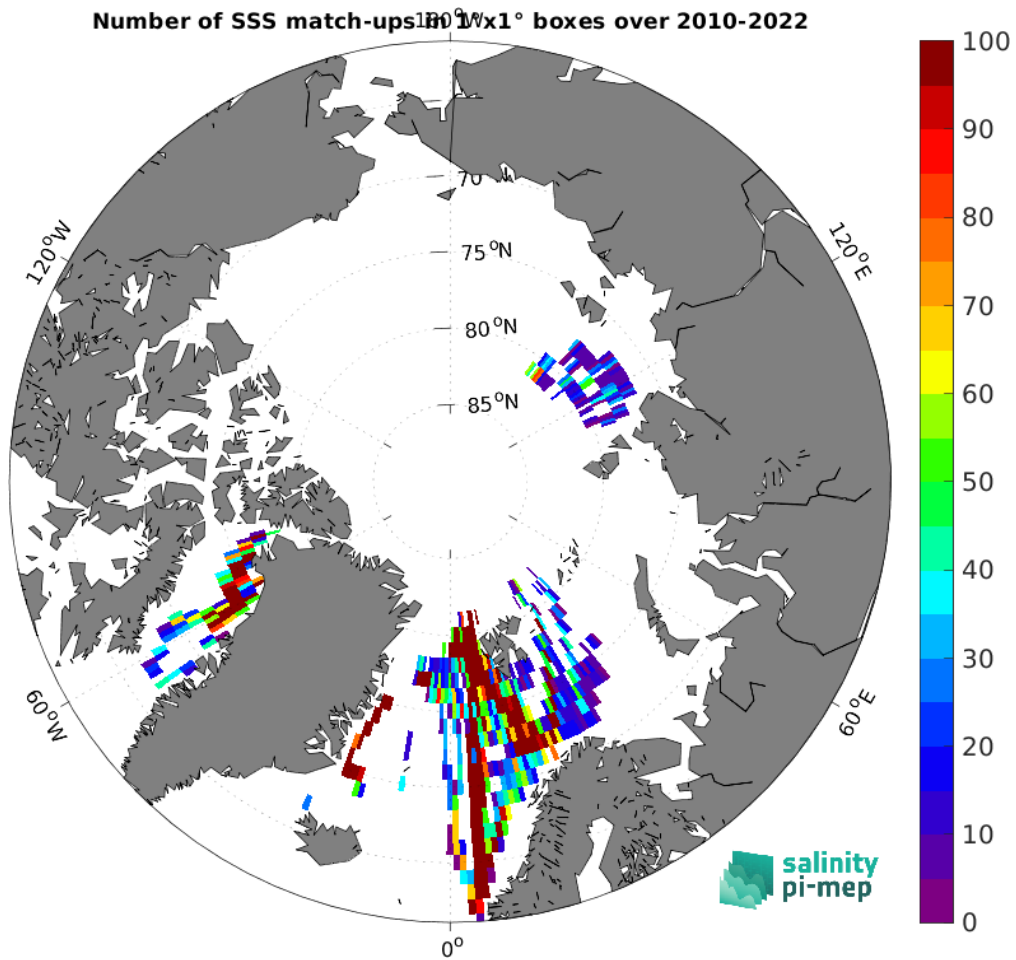
Figure 5: Number of SSS match-ups between TSG (Polarstern) SSS and the SMOS SSS L3 Arctic v2 - 9 Days (CATDS-CEC-LOCEAN) SSS product for the Arctic Ocean Pi-MEP region over 1^{\circ} \times 1^{\circ} boxes and for the full satellite product period.
