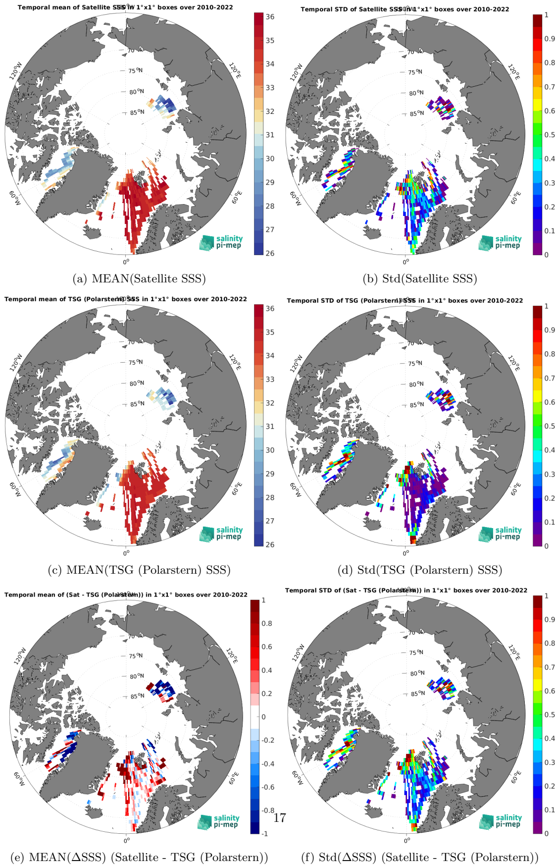
Figure 7: Temporal mean (left) and Std (right) of SSS from SMOS SSS L3 Arctic v2 - 9 Days (CATDS-CEC-LOCEAN) (top), TSG (Polarstern) (middle), and of \Delta SSS (Satellite - TSG (Polarstern)). Only match-up pairs are used to generate these maps.
