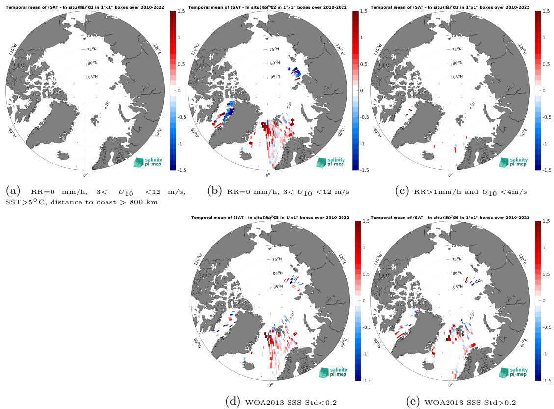
Figure 14: Temporal mean gridded over spatial boxes of size 1^\circ \times 1^\circ of \Delta SSS (SMOS SSS L3 Arctic v2 - 9 Days (CATDS-CEC-LOCEAN) - TSG (Polarstern)) for 5 different subdatasets corresponding to: RR=0 mm/h, 3 < U_{10} < 12 m/s, SST > 5°C, distance to coast > 800 km (a), RR=0 mm/h, 3 < U_{10} < 12 m/s (b), RR > 1mm/h and U_{10} < 4 m/s (c), WOA2013 SSS Std < 0.2 (d), WOA2013 SSS Std > 0.2 (e).
