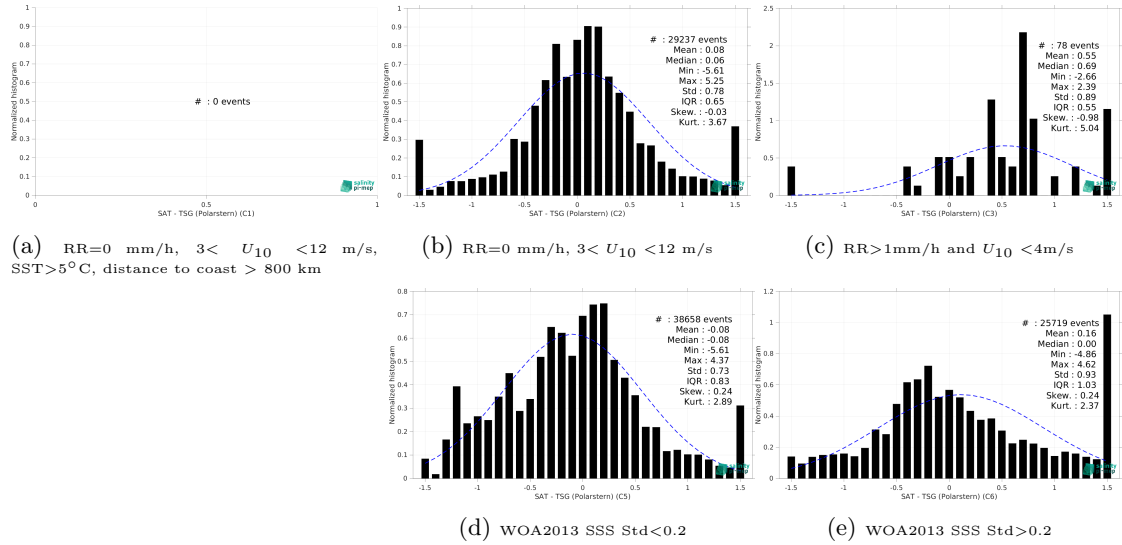
Figure 15: Normalized histogram of \Delta SSS (SMOS SSS L3 Arctic v2 - 9 Days (CATDS-CEC-LOCEAN) - TSG (Polarstern)) for 5 different subdatasets corresponding to: RR=0 mm/h, 3 < U_{10} < 12 m/s, SST > 5°C, distance to coast > 800 km (a), RR=0 mm/h, 3 < U_{10} < 12 m/s (b), RR > 1mm/h and U_{10} < 4 m/s (c), WOA2013 SSS Std < 0.2 (d), WOA2013 SSS Std > 0.2 (e).
