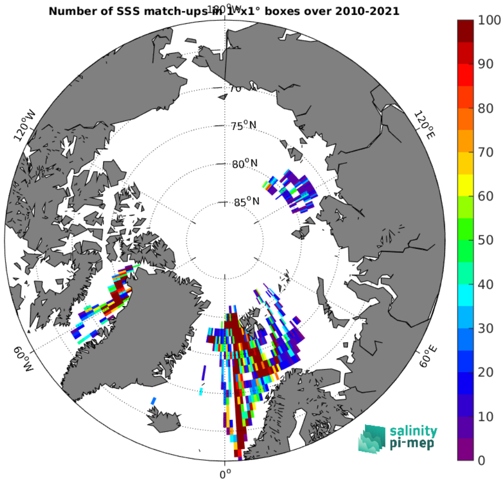
Figure 4: Number of SSS match-ups between TSG (Polarstern) SSS and the SMOS SSS L3 Arctic v2 - 9 Days (CATDS-CEC-LOCEAN) SSS product for the Arctic Ocean Pi-MEP region over 1^\circ \times 1^\circ boxes and for the full satellite product period.
