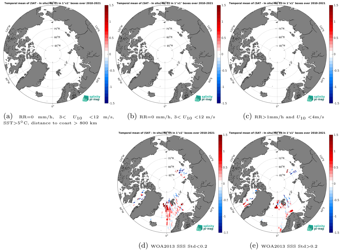
Figure 12: Temporal mean gridded over spatial boxes of size 1^{\circ}\times 1^{\circ} of \Delta\text{SSS} (SMOS SSS L3 Arctic v2 - 9 Days (CATDS-CEC-LOCEAN) - TSG (Polarstern)) for 5 different subdatasets corresponding to:RR=0 mm/h, 3 < U_{10} < 12 m/s, SST >5^{\circ}\text{C} , distance to coast > 800 km (a), RR=0 mm/h, 3 < U_{10} < 12 m/s (b), RR >1 mm/h and U_{10} < 4 m/s (c), WOA2013 SSS Std <0.2 (d), WOA2013 SSS Std >0.2 (e).
