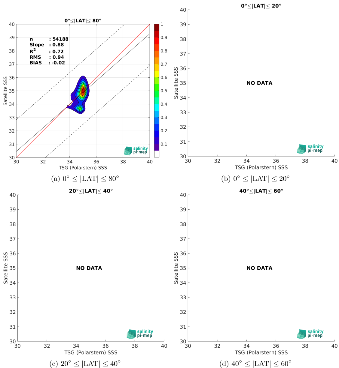
Figure 9: Contour maps of the concentration of SMOS SSS L3 Arctic v2 - 9 Days (CATDS-CEC-LOCEAN) SSS (y-axis) versus TSG (Polarstern) SSS (x-axis) at match-up pairs for different latitude bands. For each plot, the red line shows x=y . The black thin and dashed lines indicate a linear fit through the data cloud and the \pm 95\% confidence levels, respectively. The number match-up pairs n , the slope and R^2 coefficient of the linear fit, the root mean square (RMS) and the mean bias between satellite and in situ data are indicated for each latitude band in each plots.
