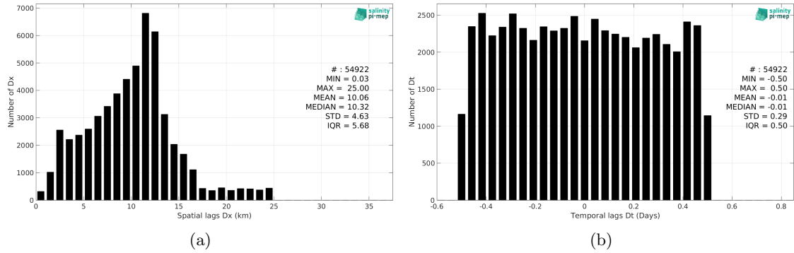
Figure 5: Histograms of the spatial (a) and temporal (b) lags between the location/time of the TSG (Polarstern) measurement and the date of the corresponding SMOS SSS L3 Arctic v2 - 9 Days (CATDS-CEC-LOCEAN) SSS pixel.
