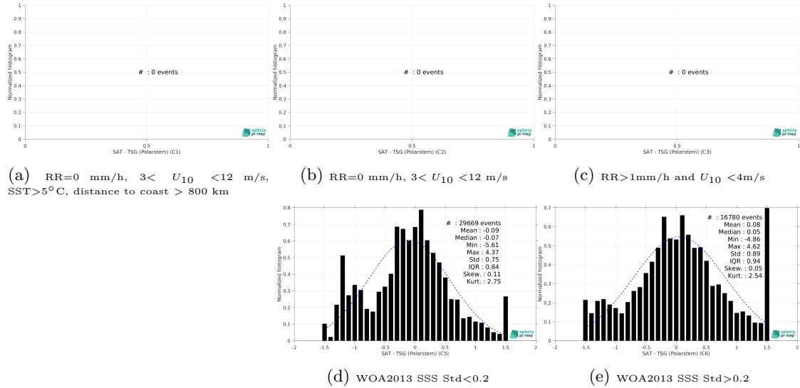
Figure 13: Normalized histogram of \Delta SSS (SMOS SSS L3 Arctic v2 - 9 Days (CATDS-CEC-LOCEAN) - TSG (Polarstern)) for 5 different subdatasets corresponding to: RR=0 mm/h, 3 < U_{10} < 12 m/s, SST>5°C, distance to coast > 800 km (a), RR=0 mm/h, 3 < U_{10} < 12 m/s (b), RR>1mm/h and U_{10} < 4 m/s (c), WOA2013 SSS Std<0.2 (d), WOA2013 SSS Std>0.2 (e).
