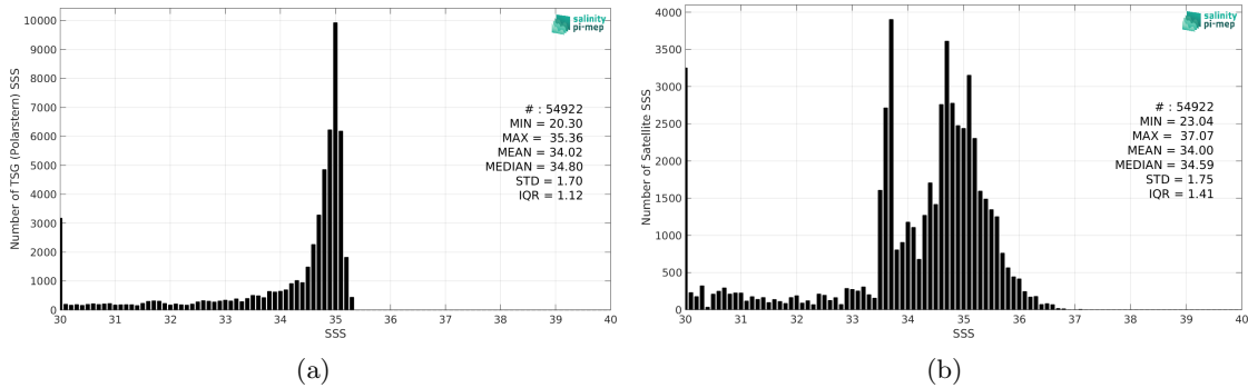
Figure 2: Histograms of SSS from TSG (Polarstern) (a) and SMOS SSS L3 Arctic v2 - 9 Days (CATDS-CEC-LOCEAN) (b) considering all match-up pairs per bins of 0.1 over the Arctic Ocean Pi-MEP region and for the full satellite product period.
