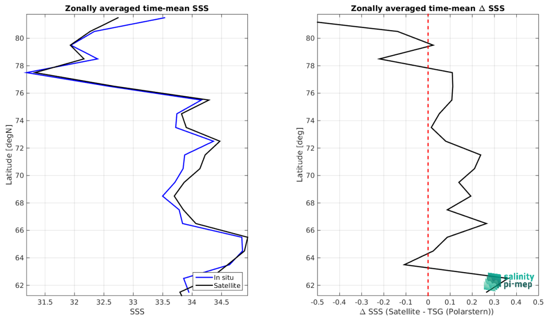
Figure 8: Left panel: Zonal mean SSS from SMOS SSS L3 Arctic v2 - 9 Days (CATDS-CEC-LOCEAN) satellite product (black) and from TSG (Polarstern) (blue). Right panel: Zonal mean of \Delta SSS (Satellite - TSG (Polarstern)) for all the collected Pi-MEP match-up pairs estimated over the full satellite product period.
