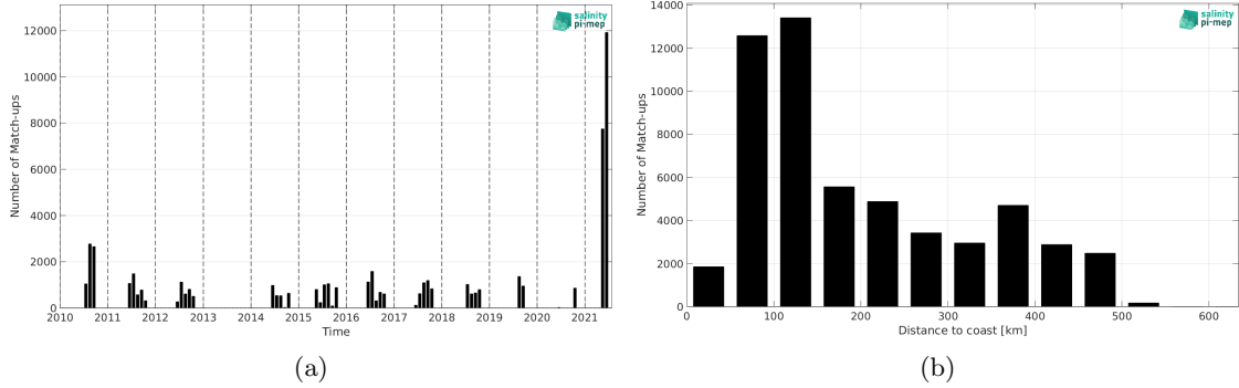
Figure 1: Number of match-ups between TSG (Polarstern) and SMOS SSS L3 Arctic v2 - 9 Days (CATDS-CEC-LOCEAN) SSS as a function of time (a) and as function of the distance to coast (b) over the Arctic Ocean Pi-MEP region and for the full satellite product period.
