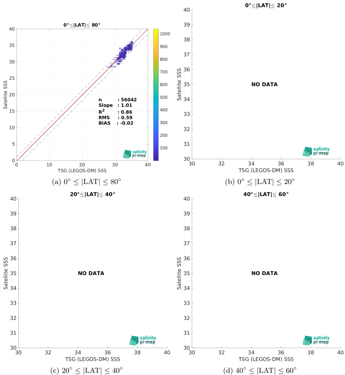
Figure 10: Contour maps of the concentration of SMOS SSS L3 Arctic v2 - 9 Days (CATDS-CEC-LOCEAN) SSS (y-axis) versus TSG (LEGOS-DM) SSS (x-axis) at match-up pairs for different latitude bands. For each plot, the red line shows x=y . The black thin and dashed lines indicate a linear fit through the data cloud and the \pm 95\% confidence levels, respectively. The number match-up pairs n , the slope and R^2 coefficient of the linear fit, the root mean square (RMS) and the mean bias between satellite and in situ data are indicated for each latitude band in each plots.
