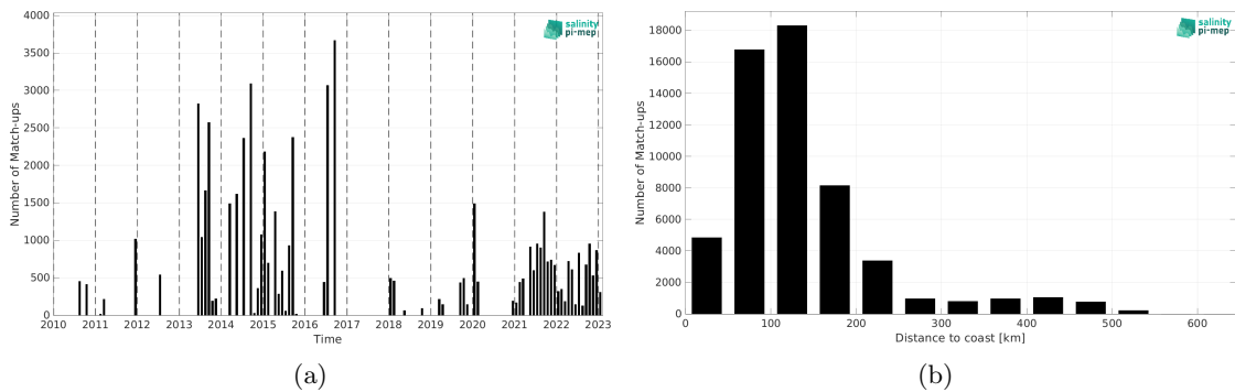
Figure 2: Number of match-ups between TSG (LEGOS-DM) and SMOS SSS L3 Arctic v2 - 9 Days (CATDS-CEC-LOCEAN) SSS as a function of time (a) and as function of the distance to coast (b) over the Arctic Ocean Pi-MEP region and for the full satellite product period.
