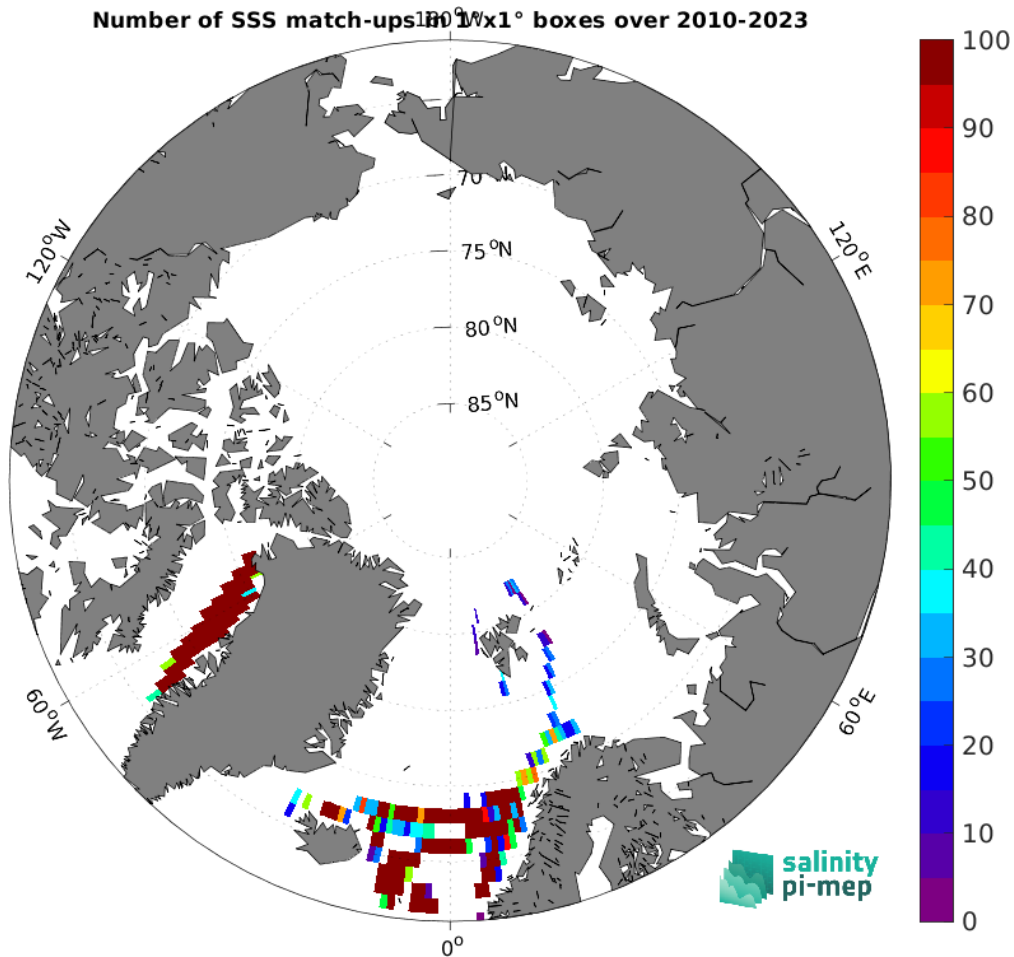
Figure 5: Number of SSS match-ups between TSG (LEGOS-DM) SSS and the SMOS SSS L3 Arctic v2 - 9 Days (CATDS-CEC-LOCEAN) SSS product for the Arctic Ocean Pi-MEP region over 1^\circ \times 1^\circ boxes and for the full satellite product period.
