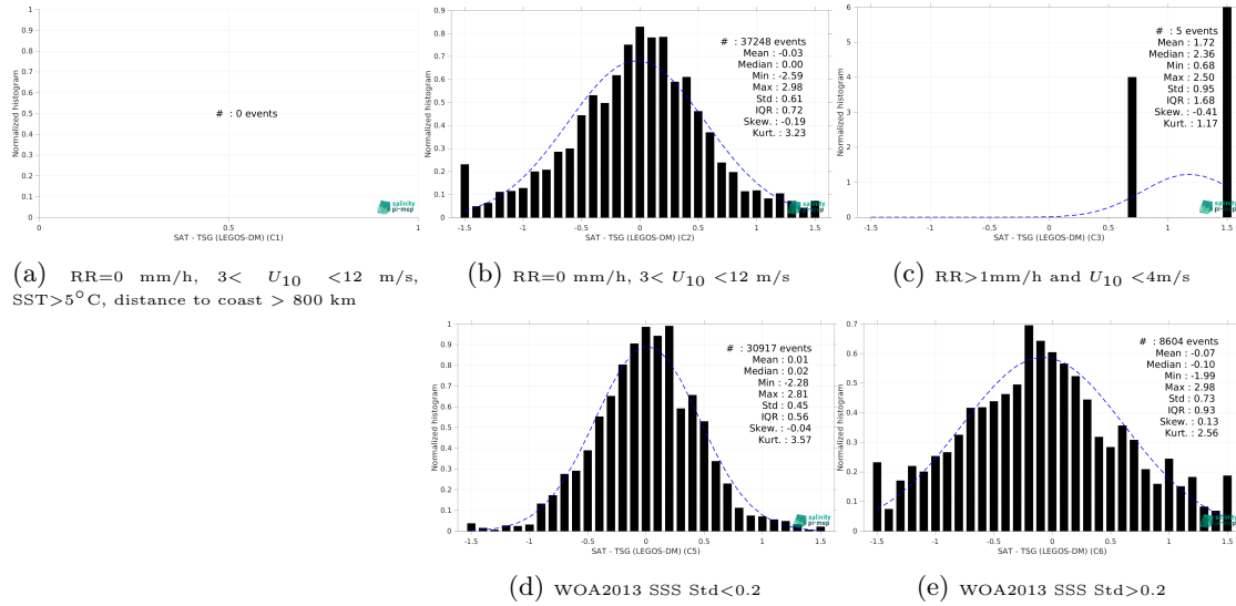
Figure 15: Normalized histogram of \Delta\text{SSS} (SMOS SSS L3 Arctic v2 - 9 Days (CATDS-CEC-LOCEAN) - TSG (LEGOS-DM)) for 5 different subdatasets corresponding to: RR=0 mm/h, 3 < U_{10} < 12 m/s, SST > 5^\circ\text{C} , distance to coast > 800 km (a), RR=0 mm/h, 3 < U_{10} < 12 m/s (b), RR > 1\text{mm/h} and U_{10} < 4\text{m/s} (c), WOA2013 SSS Std < 0.2 (d), WOA2013 SSS Std > 0.2 (e).
