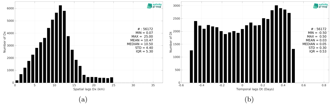
Figure 6: Histograms of the spatial (a) and temporal (b) lags between the location/time of the TSG (LEGOS-DM) measurement and the date of the corresponding SMOS SSS L3 Arctic v2 - 9 Days (CATDS-CEC-LOCEAN) SSS pixel.
