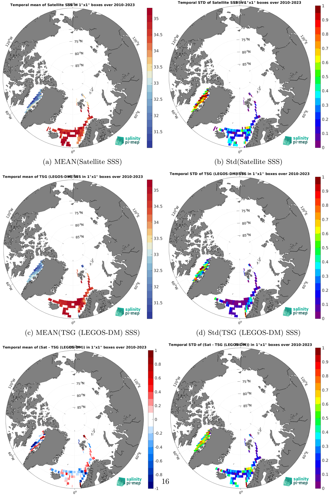
(e) MEAN( \Delta SSS) (Satellite - TSG (LEGOS-DM)) (f) Std( \Delta SSS) (Satellite - TSG (LEGOS-DM)) Figure 7: Temporal mean (left) and Std (right) of SSS from SMOS SSS L3 Arctic v2 - 9 Days (CATDS-CEC-LOCEAN) (top), TSG (LEGOS-DM) (middle), and of \Delta SSS (Satellite - TSG (LEGOS-DM)). Only match-up pairs are used to generate these maps.
