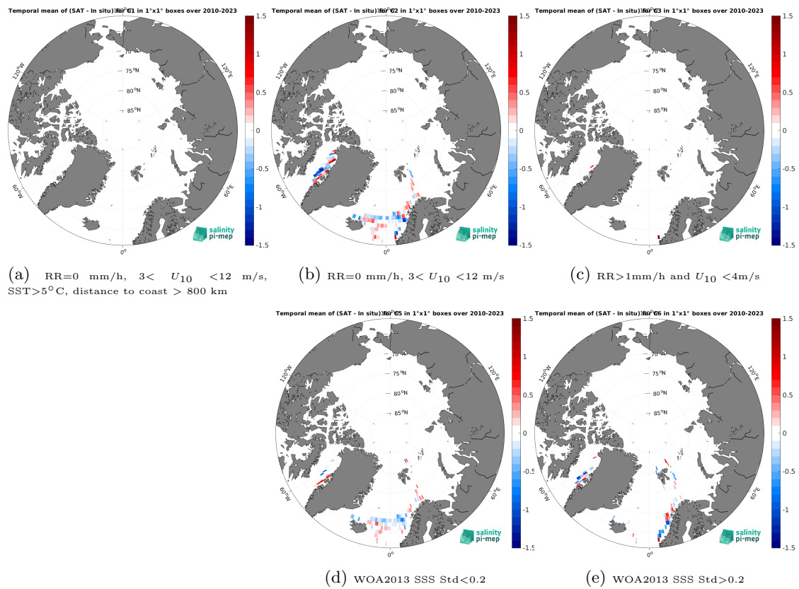
Figure 14: Temporal mean gridded over spatial boxes of size 1^\circ \times 1^\circ of \Delta\text{SSS} (SMOS SSS L3 Arctic v2 - 9 Days (CATDS-CEC-LOCEAN) - TSG (LEGOS-DM)) for 5 different subdatasets corresponding to:RR=0 mm/h, 3 < U_{10} < 12 m/s, SST >5^\circ\text{C} , distance to coast > 800 km (a), RR=0 mm/h, 3 < U_{10} < 12 m/s (b), RR >1 mm/h and U_{10} < 4 m/s (c), WOA2013 SSS Std <0.2 (d), WOA2013 SSS Std >0.2 (e).
