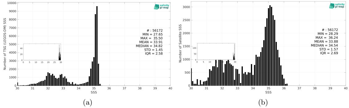
Figure 3: Histograms of SSS from TSG (LEGOS-DM) (a) and SMOS SSS L3 Arctic v2 - 9 Days (CATDS-CEC-LOCEAN) (b) considering all match-up pairs per bins of 0.1 over the Arctic Ocean Pi-MEP region and for the full satellite product period.
