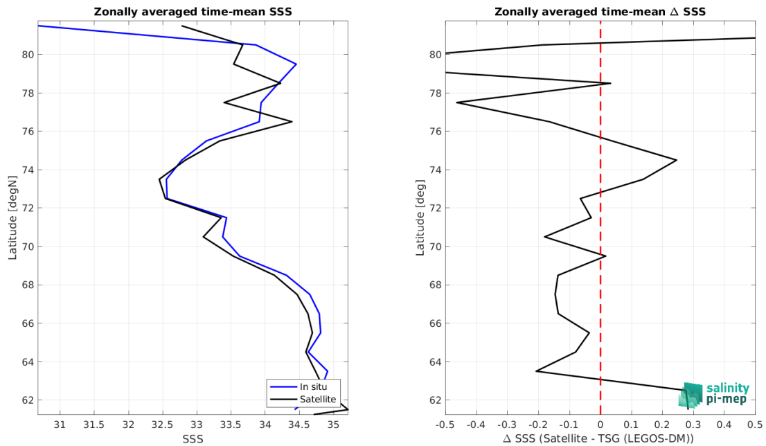
Figure 9: Left panel: Zonal mean SSS from SMOS SSS L3 Arctic v2 - 9 Days (CATDS-CEC-LOCEAN) satellite product (black) and from TSG (LEGOS-DM) (blue). Right panel: Zonal mean of \Delta SSS (Satellite - TSG (LEGOS-DM)) for all the collected Pi-MEP match-up pairs estimated over the full satellite product period.
