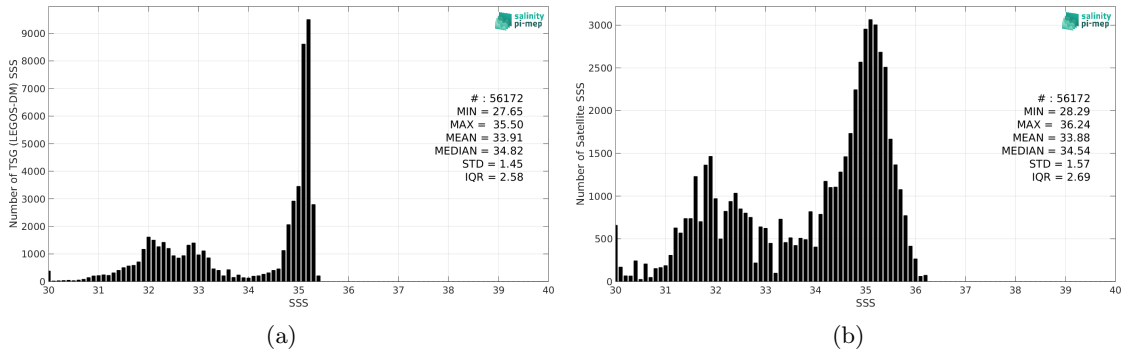
Figure 2: Histograms of SSS from TSG (LEGOS-DM) (a) and SMOS SSS L3 Arctic v2 - 9 Days (CATDS-CEC-LOCEAN) (b) considering all match-up pairs per bins of 0.1 over the Arctic Ocean Pi-MEP region and for the full satellite product period.
