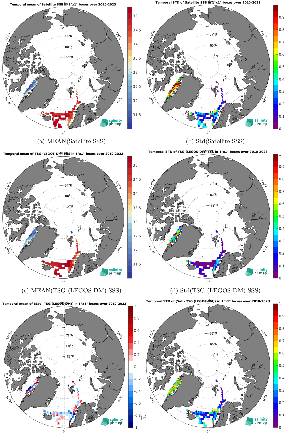
(e) MEAN( \Delta SSS) (Satellite - TSG (LEGOS-DM)) (f) Std( \Delta SSS) (Satellite - TSG (LEGOS-DM)) Figure 6: Temporal mean (left) and Std (right) of SSS from SMOS SSS L3 Arctic v2 - 9 Days (CATDS-CEC-LOCEAN) (top), TSG (LEGOS-DM) (middle), and of \Delta SSS (Satellite - TSG (LEGOS-DM)). Only match-up pairs are used to generate these maps.
