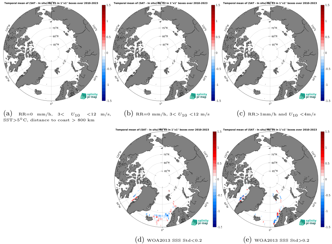
Figure 12: Temporal mean gridded over spatial boxes of size 1^{\circ}\times 1^{\circ} of \Delta\text{SSS} (SMOS SSS L3 Arctic v2 - 9 Days (CATDS-CEC-LOCEAN) - TSG (LEGOS-DM)) for 5 different subdatasets corresponding to:RR=0 mm/h, 3 < U_{10} < 12 m/s, SST >5^{\circ}\text{C} , distance to coast > 800 km (a), RR=0 mm/h, 3 < U_{10} < 12 m/s (b), RR >1 mm/h and U_{10} < 4 m/s (c), WOA2013 SSS Std <0.2 (d), WOA2013 SSS Std >0.2 (e).
