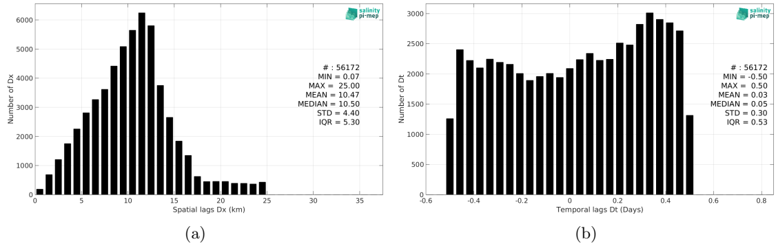
Figure 5: Histograms of the spatial (a) and temporal (b) lags between the location/time of the TSG (LEGOS-DM) measurement and the date of the corresponding SMOS SSS L3 Arctic v2 - 9 Days (CATDS-CEC-LOCEAN) SSS pixel.
