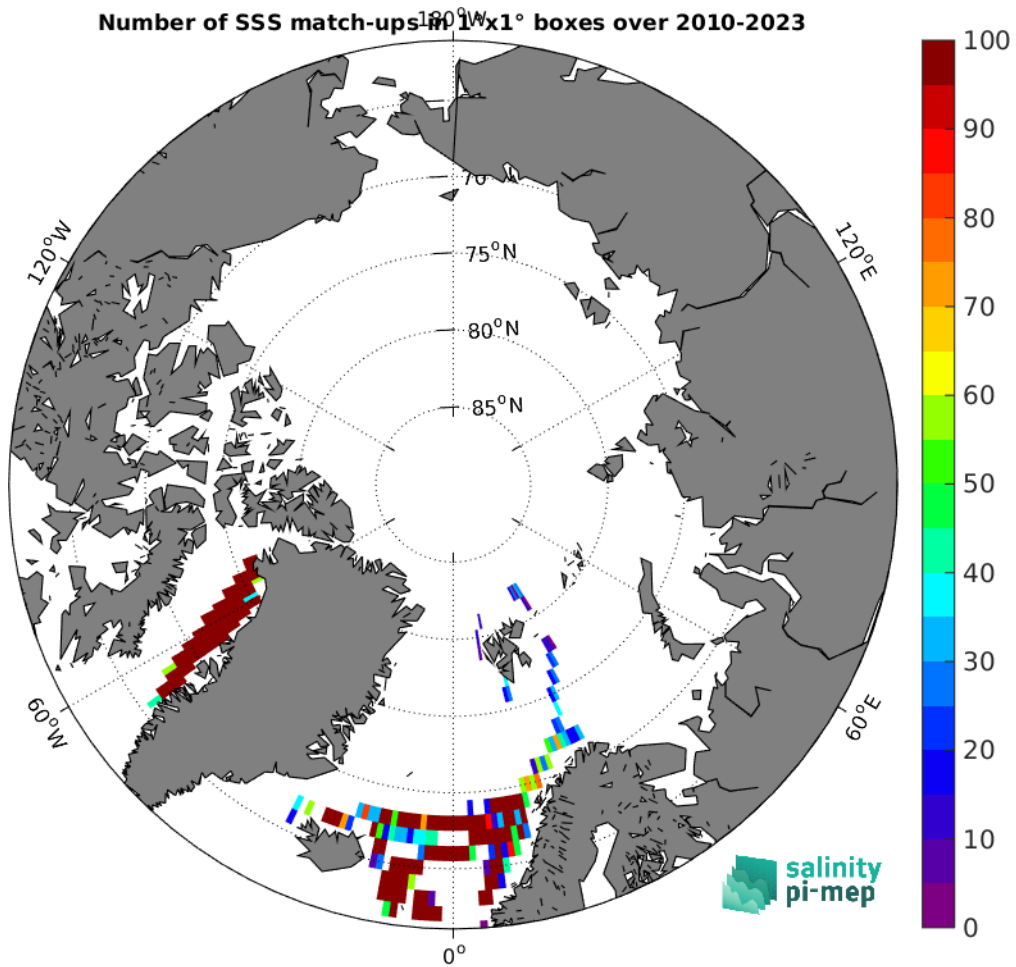
Figure 4: Number of SSS match-ups between TSG (LEGOS-DM) SSS and the SMOS SSS L3 Arctic v2 - 9 Days (CATDS-CEC-LOCEAN) SSS product for the Arctic Ocean Pi-MEP region over 1^\circ \times 1^\circ boxes and for the full satellite product period.
