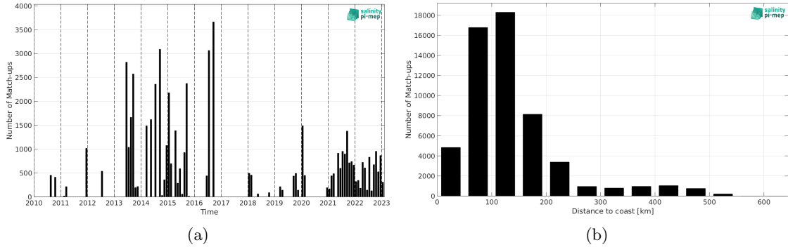
Figure 1: Number of match-ups between TSG (LEGOS-DM) and SMOS SSS L3 Arctic v2 - 9 Days (CATDS-CEC-LOCEAN) SSS as a function of time (a) and as function of the distance to coast (b) over the Arctic Ocean Pi-MEP region and for the full satellite product period.
