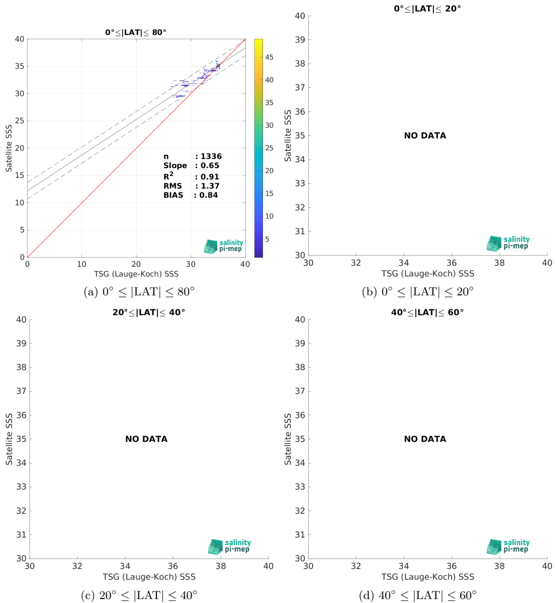
Figure 10: Contour maps of the concentration of SMOS SSS L3 Arctic v2 - 9 Days (CATDS-CEC-LOCEAN) SSS (y-axis) versus TSG (Lauge-Koch) SSS (x-axis) at match-up pairs for different latitude bands. For each plot, the red line shows x=y . The black thin and dashed lines indicate a linear fit through the data cloud and the \pm 95\% confidence levels, respectively. The number match-up pairs n , the slope and R^2 coefficient of the linear fit, the root mean square (RMS) and the mean bias between satellite and in situ data are indicated for each latitude band in each plots.
