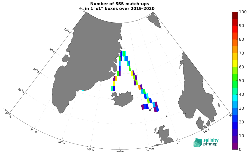
Figure 5: Number of SSS match-ups between TSG (Lauge-Koch) SSS and the SMOS SSS L3 Arctic v2 - 9 Days (CATDS-CEC-LOCEAN) SSS product for the Arctic Ocean Pi-MEP region over 1^\circ \times 1^\circ boxes and for the full satellite product period.
