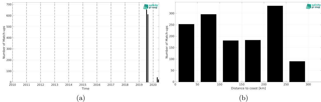
Figure 2: Number of match-ups between TSG (Lauge-Koch) and SMOS SSS L3 Arctic v2 - 9 Days (CATDS-CEC-LOCEAN) SSS as a function of time (a) and as function of the distance to coast (b) over the Arctic Ocean Pi-MEP region and for the full satellite product period.
