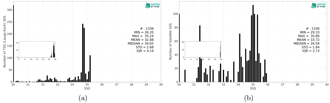
Figure 3: Histograms of SSS from TSG (Lauge-Koch) (a) and SMOS SSS L3 Arctic v2 - 9 Days (CATDS-CEC-LOCEAN) (b) considering all match-up pairs per bins of 0.1 over the Arctic Ocean Pi-MEP region and for the full satellite product period.
