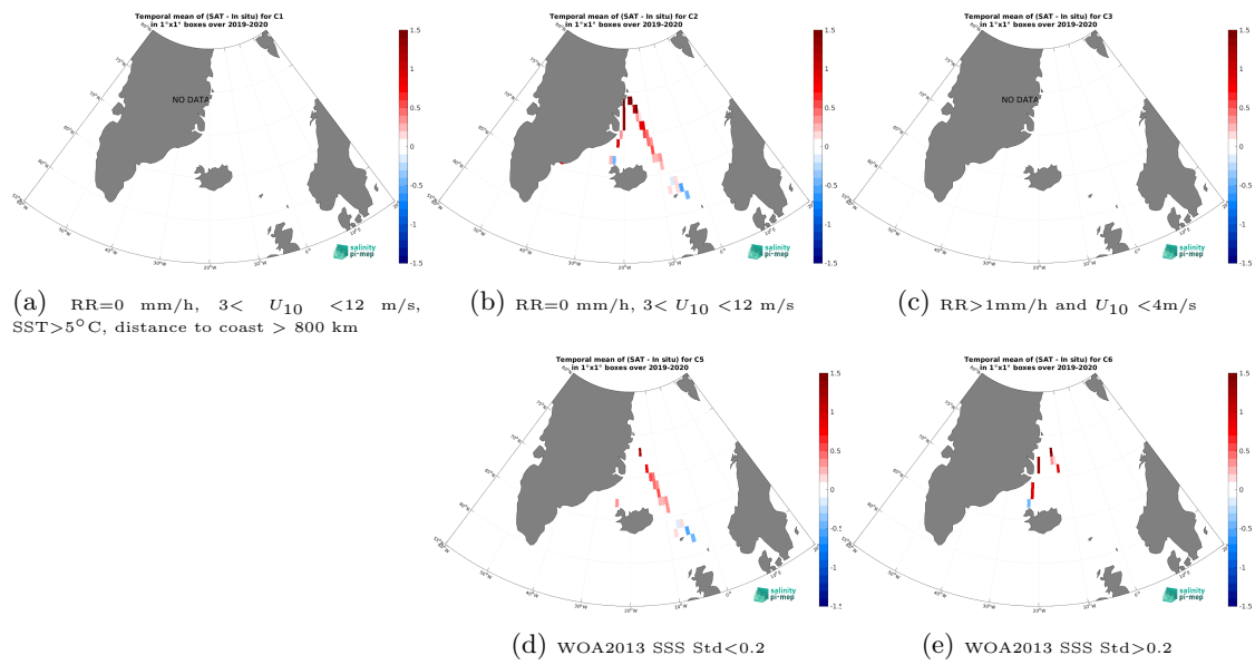
Figure 14: Temporal mean gridded over spatial boxes of size 1^\circ \times 1^\circ of \Delta SSS (SMOS SSS L3 Arctic v2 - 9 Days (CATDS-CEC-LOCEAN) - TSG (Lauge-Koch)) for 5 different subdatasets corresponding to: RR=0 mm/h, 3 < U_{10} < 12 m/s, SST > 5^\circ\text{C} , distance to coast > 800 km (a), RR=0 mm/h, 3 < U_{10} < 12 m/s (b), RR > 1 mm/h and U_{10} < 4 m/s (c), WOA2013 SSS Std < 0.2 (d), WOA2013 SSS Std > 0.2 (e).
