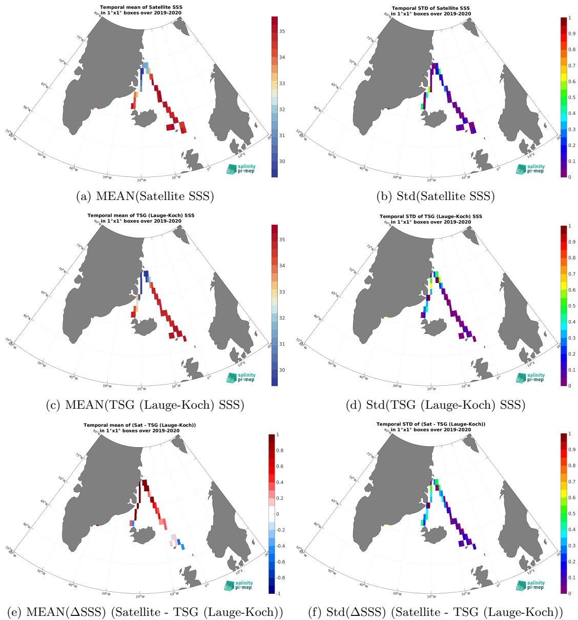
Figure 7: Temporal mean (left) and Std (right) of SSS from SMOS SSS L3 Arctic v2 - 9 Days (CATDS-CEC-LOCEAN) (top), TSG (Lauge-Koch) (middle), and of \Delta SSS (Satellite - TSG (Lauge-Koch)). Only match-up pairs are used to generate these maps.
