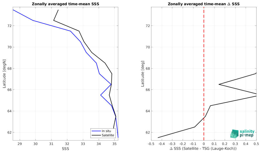
Figure 9: Left panel: Zonal mean SSS from SMOS SSS L3 Arctic v2 - 9 Days (CATDS-CEC-LOCEAN) satellite product (black) and from TSG (Lauge-Koch) (blue). Right panel: Zonal mean of \Delta SSS (Satellite - TSG (Lauge-Koch)) for all the collected Pi-MEP match-up pairs estimated over the full satellite product period.
