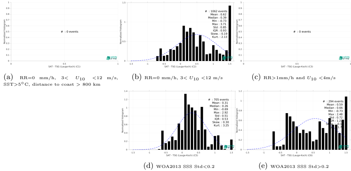
Figure 15: Normalized histogram of \Delta SSS (SMOS SSS L3 Arctic v2 - 9 Days (CATDS-CEC-LOCEAN) - TSG (Lauge-Koch)) for 5 different subdatasets corresponding to: RR=0 mm/h, 3 < U_{10} < 12 m/s, SST > 5°C, distance to coast > 800 km (a), RR=0 mm/h, 3 < U_{10} < 12 m/s (b), RR > 1mm/h and U_{10} < 4 m/s (c), WOA2013 SSS Std < 0.2 (d), WOA2013 SSS Std > 0.2 (e).
