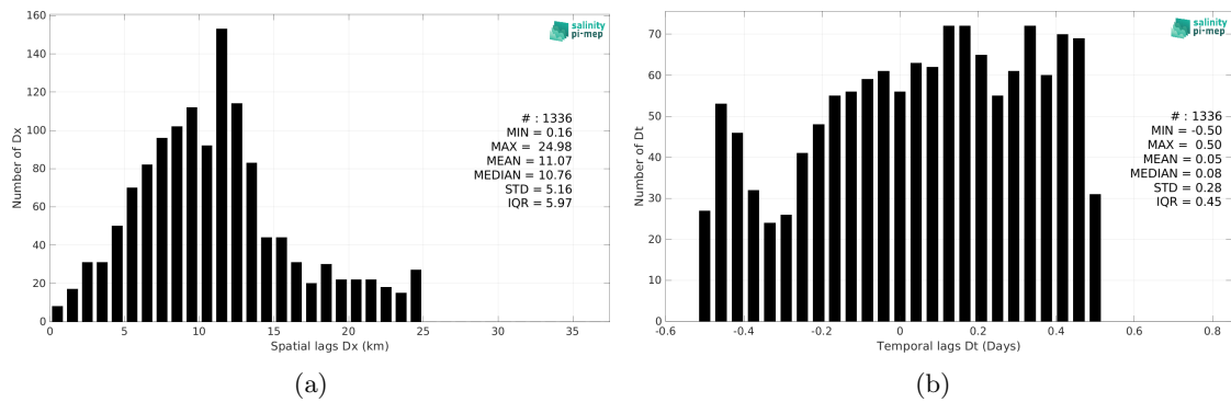
Figure 6: Histograms of the spatial (a) and temporal (b) lags between the location/time of the TSG (Lauge-Koch) measurement and the date of the corresponding SMOS SSS L3 Arctic v2 - 9 Days (CATDS-CEC-LOCEAN) SSS pixel.
