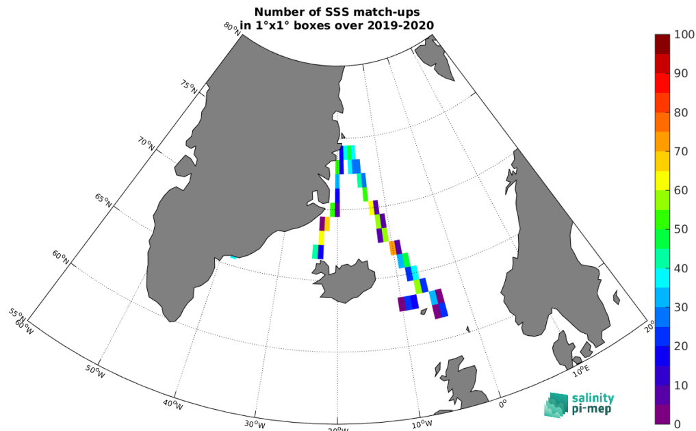
Figure 4: Number of SSS match-ups between TSG (Lauge-Koch) SSS and the SMOS SSS L3 Arctic v2 - 9 Days (CATDS-CEC-LOCEAN) SSS product for the Arctic Ocean Pi-MEP region over 1^\circ \times 1^\circ boxes and for the full satellite product period.
