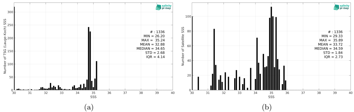
Figure 2: Histograms of SSS from TSG (Lauge-Koch) (a) and SMOS SSS L3 Arctic v2 - 9 Days (CATDS-CEC-LOCEAN) (b) considering all match-up pairs per bins of 0.1 over the Arctic Ocean Pi-MEP region and for the full satellite product period.
