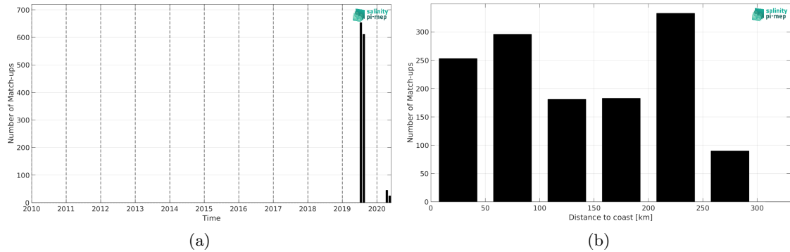
Figure 1: Number of match-ups between TSG (Lauge-Koch) and SMOS SSS L3 Arctic v2 - 9 Days (CATDS-CEC-LOCEAN) SSS as a function of time (a) and as function of the distance to coast (b) over the Arctic Ocean Pi-MEP region and for the full satellite product period.
