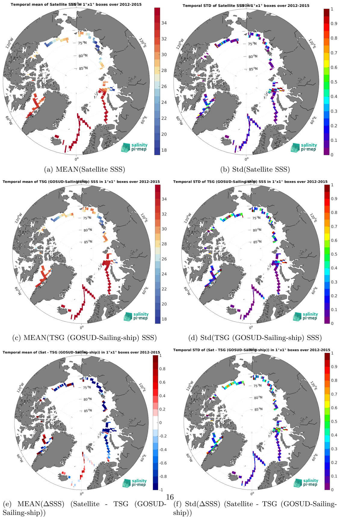
Figure 7: Temporal mean (left) and Std (right) of SSS from SMOS SSS L3 Arctic v2 - 9 Days (CATDS-CEC-LOCEAN) (top), TSG (GOSUD-Sailing-ship) (middle), and of \Delta SSS (Satellite - TSG (GOSUD-Sailing-ship)). Only match-up pairs are used to generate these maps.
