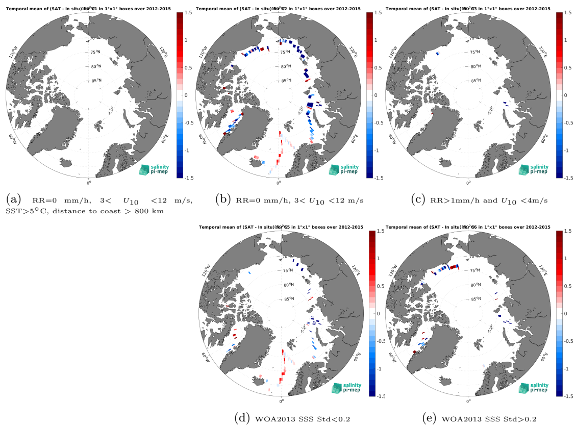
Figure 14: Temporal mean gridded over spatial boxes of size 1^\circ \times 1^\circ of \Delta\text{SSS} (SMOS SSS L3 Arctic v2 - 9 Days (CATDS-CEC-LOCEAN) - TSG (GOSUD-Sailing-ship)) for 5 different subdatasets corresponding to: RR=0 mm/h, 3 < U_{10} < 12 m/s, SST > 5°C, distance to coast > 800 km (a), RR=0 mm/h, 3 < U_{10} < 12 m/s (b), RR > 1mm/h and U_{10} < 4 m/s (c), WOA2013 SSS Std < 0.2 (d), WOA2013 SSS Std > 0.2 (e).
