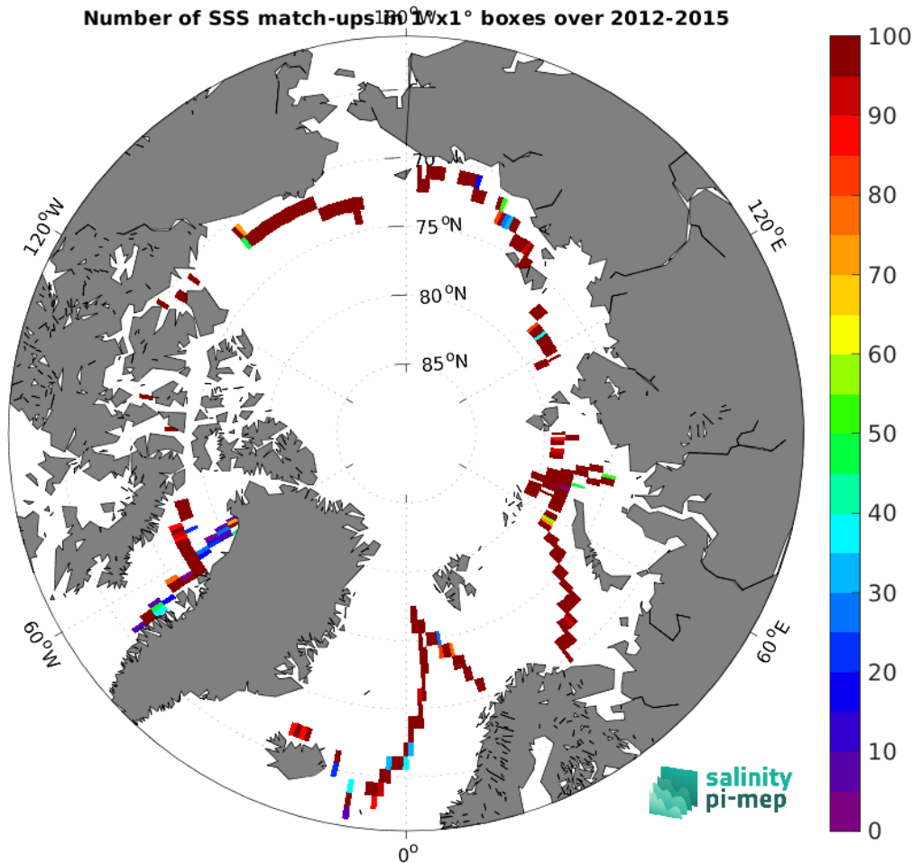
Figure 5: Number of SSS match-ups between TSG (GOSUD-Sailing-ship) SSS and the SMOS SSS L3 Arctic v2 - 9 Days (CATDS-CEC-LOCEAN) SSS product for the Arctic Ocean Pi-MEP region over 1^\circ \times 1^\circ boxes and for the full satellite product period.
