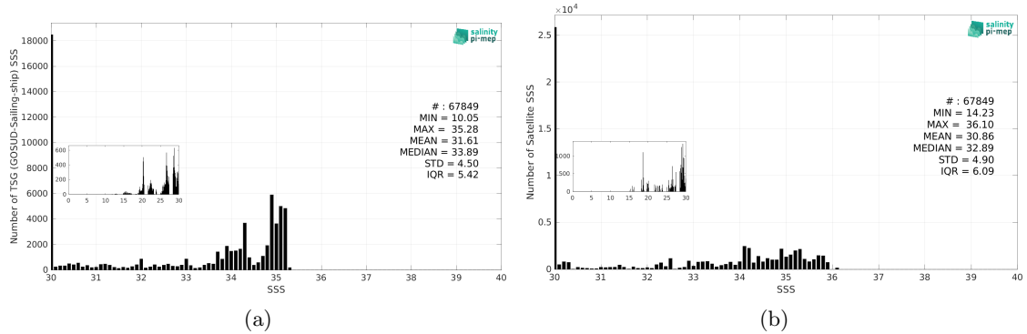
Figure 3: Histograms of SSS from TSG (GOSUD-Sailing-ship) (a) and SMOS SSS L3 Arctic v2 - 9 Days (CATDS-CEC-LOCEAN) (b) considering all match-up pairs per bins of 0.1 over the Arctic Ocean Pi-MEP region and for the full satellite product period.
