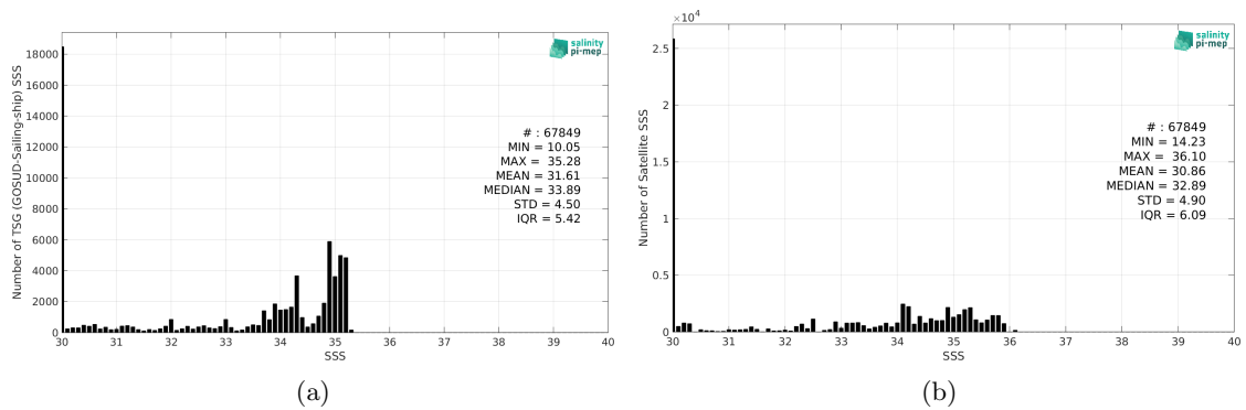
Figure 2: Histograms of SSS from TSG (GOSUD-Sailing-ship) (a) and SMOS SSS L3 Arctic v2 - 9 Days (CATDS-CEC-LOCEAN) (b) considering all match-up pairs per bins of 0.1 over the Arctic Ocean Pi-MEP region and for the full satellite product period.
