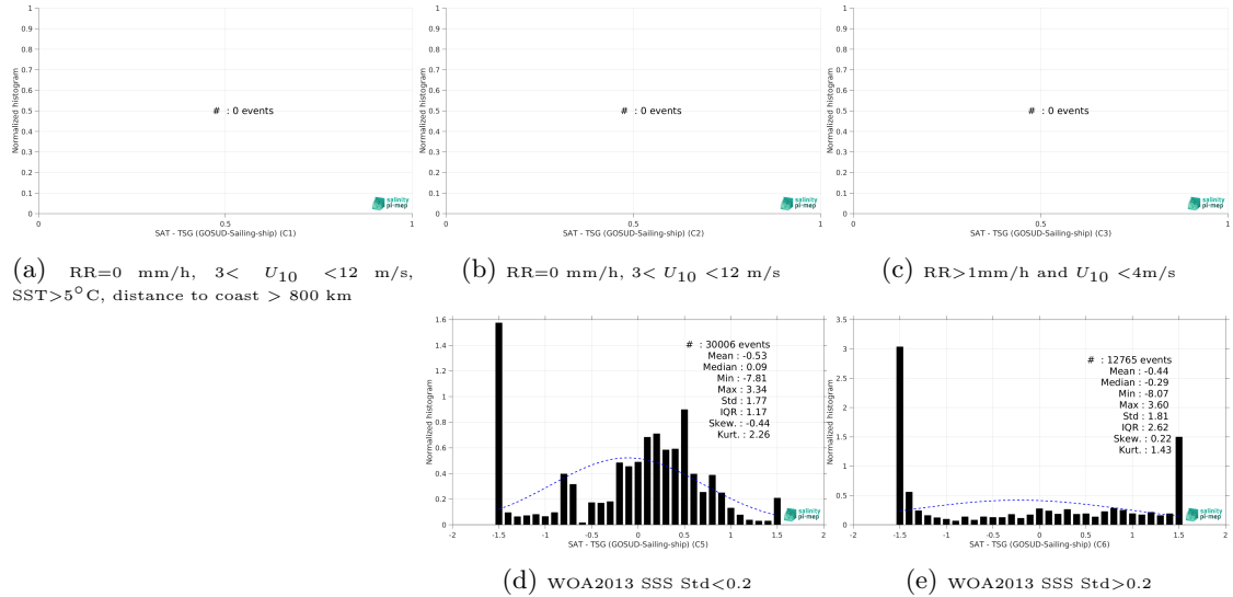
Figure 13: Normalized histogram of \Delta SSS (SMOS SSS L3 Arctic v2 - 9 Days (CATDS-CEC-LOCEAN) - TSG (GOSUD-Sailing-ship)) for 5 different subdatasets corresponding to: RR=0 mm/h, 3 < U_{10} < 12 m/s, SST > 5°C, distance to coast > 800 km (a), RR=0 mm/h, 3 < U_{10} < 12 m/s (b), RR > 1mm/h and U_{10} < 4 m/s (c), WOA2013 SSS Std < 0.2 (d), WOA2013 SSS Std > 0.2 (e).
