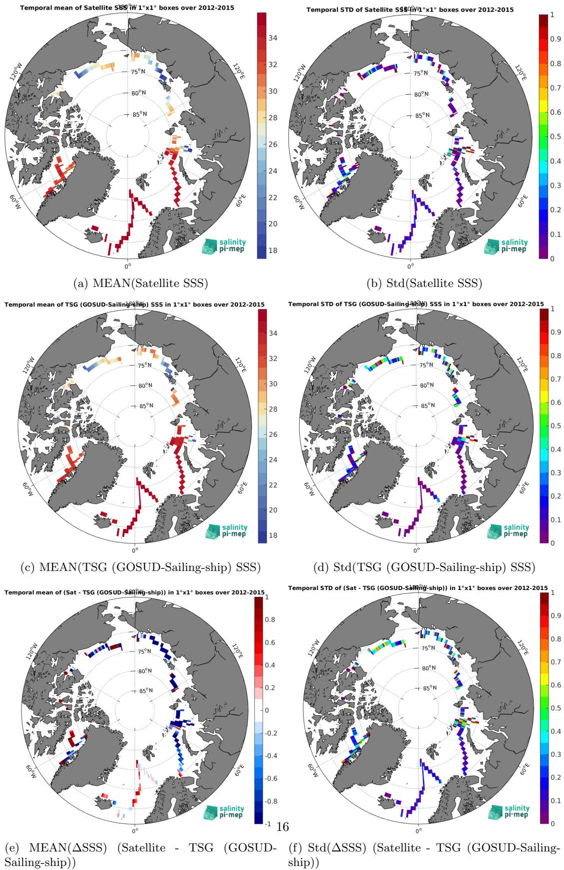
Figure 6: Temporal mean (left) and Std (right) of SSS from SMOS SSS L3 Arctic v2 - 9 Days (CATDS-CEC-LOCEAN) (top), TSG (GOSUD-Sailing-ship) (middle), and of \Delta SSS (Satellite - TSG (GOSUD-Sailing-ship)). Only match-up pairs are used to generate these maps.
