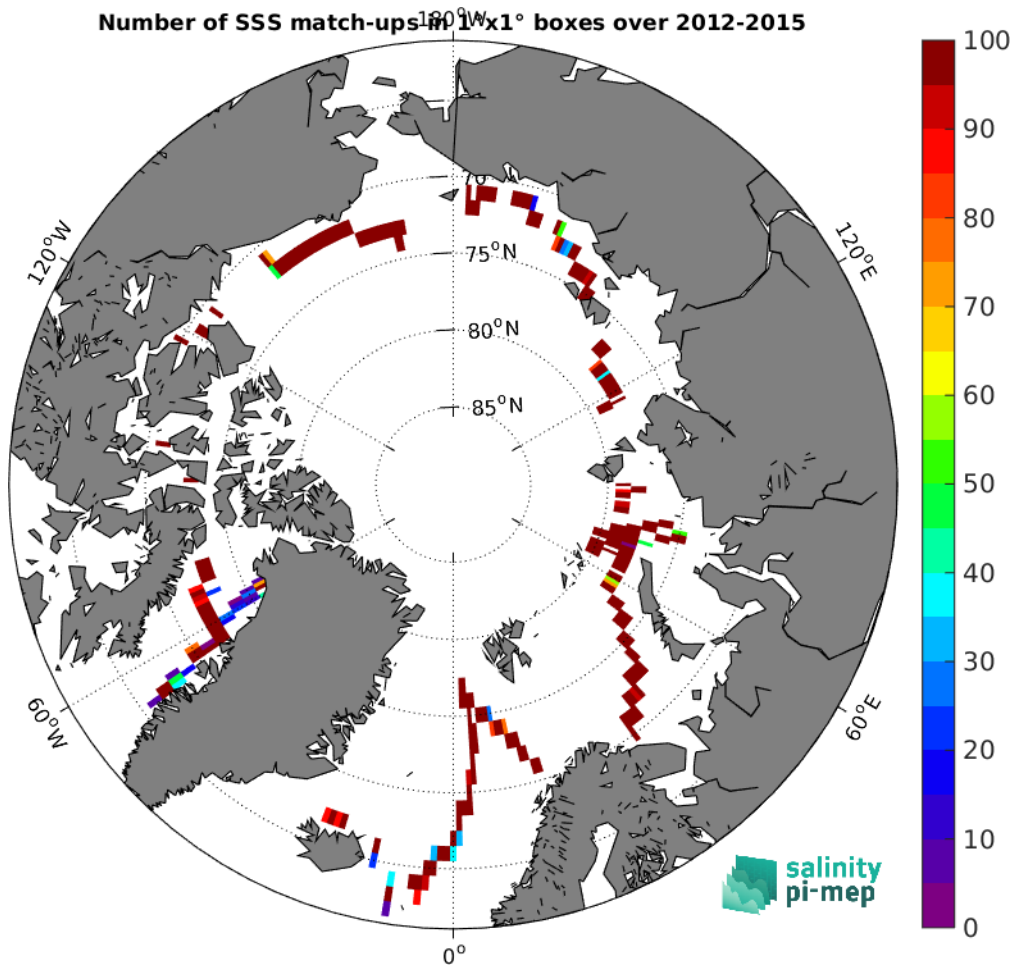
Figure 4: Number of SSS match-ups between TSG (GOSUD-Sailing-ship) SSS and the SMOS SSS L3 Arctic v2 - 9 Days (CATDS-CEC-LOCEAN) SSS product for the Arctic Ocean Pi-MEP region over 1^\circ \times 1^\circ boxes and for the full satellite product period.
