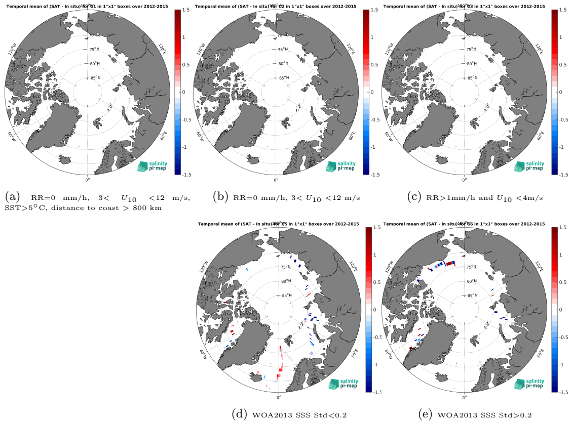
Figure 12: Temporal mean gridded over spatial boxes of size 1^\circ \times 1^\circ of \Delta SSS (SMOS SSS L3 Arctic v2 - 9 Days (CATDS-CEC-LOCEAN) - TSG (GOSUD-Sailing-ship)) for 5 different subdatasets corresponding to: RR=0 mm/h, 3 < U_{10} < 12 m/s, SST>5°C, distance to coast > 800 km (a), RR=0 mm/h, 3 < U_{10} < 12 m/s (b), RR>1mm/h and U_{10} < 4 m/s (c), WOA2013 SSS Std<0.2 (d), WOA2013 SSS Std>0.2 (e).
