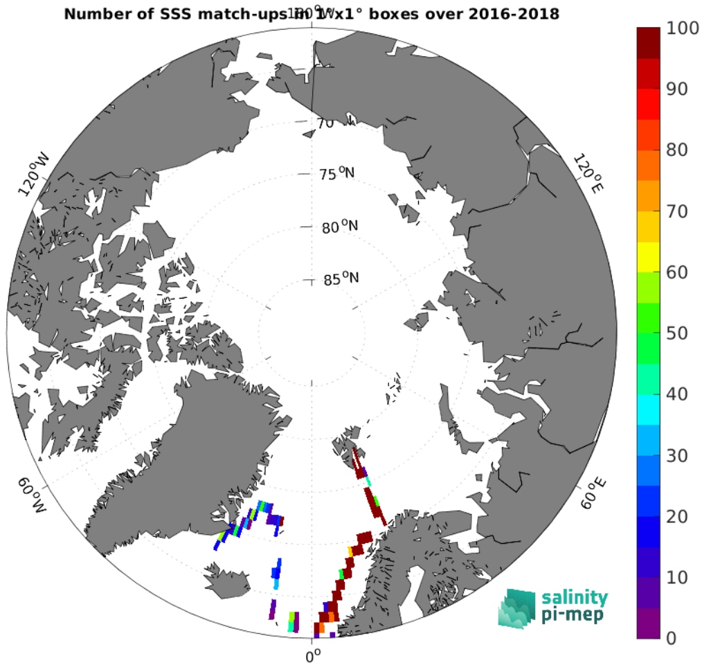
Figure 5: Number of SSS match-ups between TSG (GOSUD-Research-vessel) SSS and the SMOS SSS L3 Arctic v2 - 9 Days (CATDS-CEC-LOCEAN) SSS product for the Arctic Ocean Pi-MEP region over 1^\circ \times 1^\circ boxes and for the full satellite product period.
