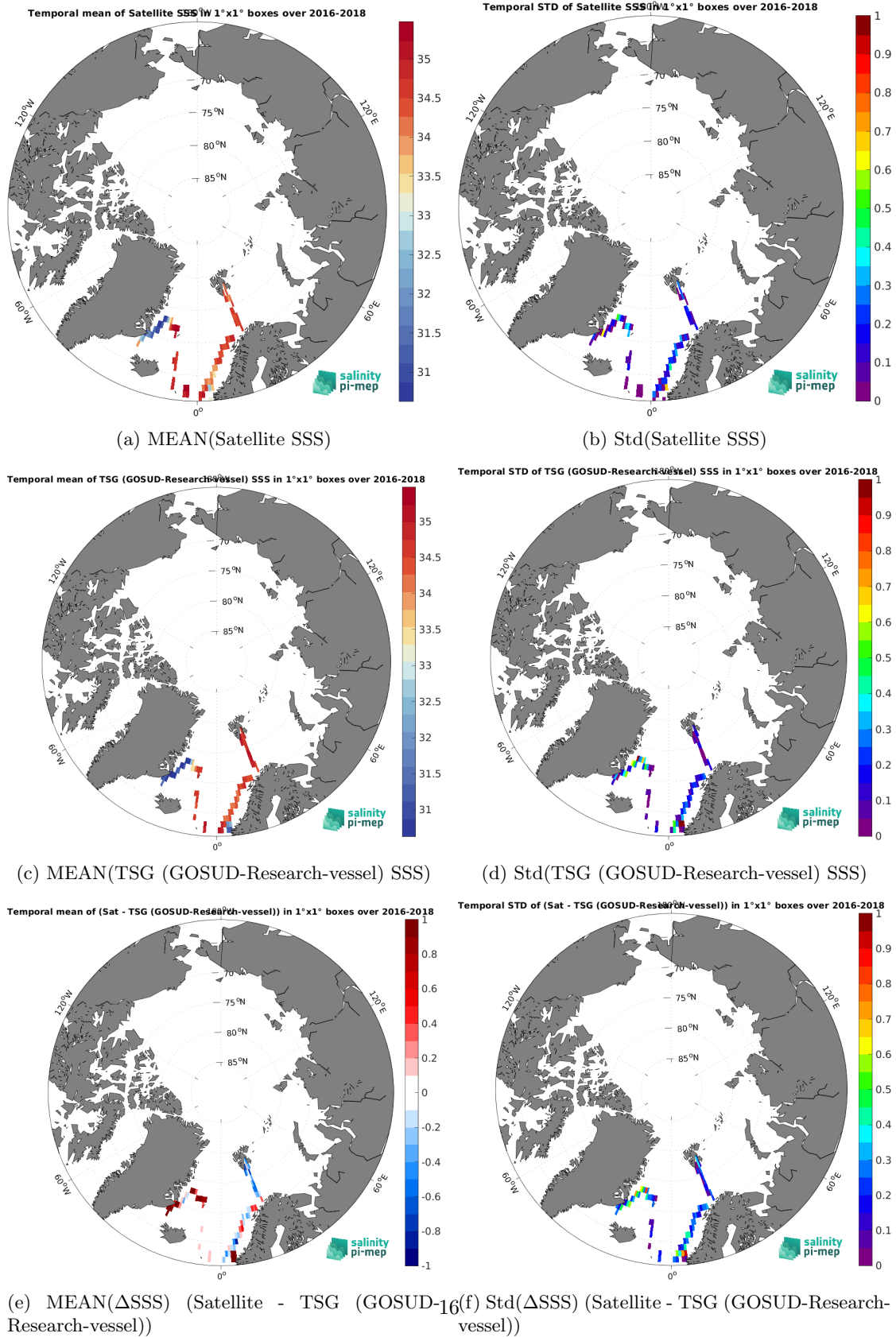
Figure 7: Temporal mean (left) and Std (right) of SSS from SMOS SSS L3 Arctic v2 - 9 Days (CATDS-CEC-LOCEAN) (top), TSG (GOSUD-Research-vessel) (middle), and of \Delta SSS (Satellite - TSG (GOSUD-Research-vessel)). Only match-up pairs are used to generate these maps.
