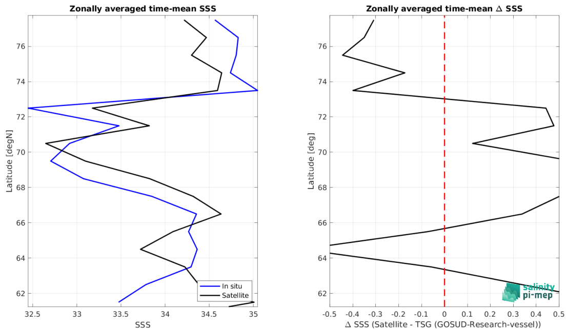
Figure 9: Left panel: Zonal mean SSS from SMOS SSS L3 Arctic v2 - 9 Days (CATDS-CEC-LOCEAN) satellite product (black) and from TSG (GOSUD-Research-vessel) (blue). Right panel: Zonal mean of \Delta SSS (Satellite - TSG (GOSUD-Research-vessel)) for all the collected Pi-MEP match-up pairs estimated over the full satellite product period.
