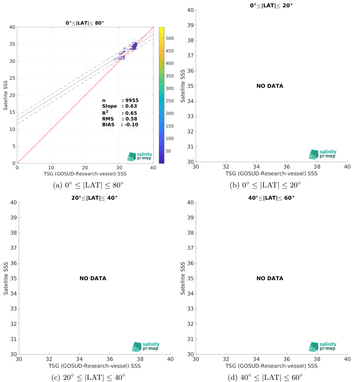
Figure 10: Contour maps of the concentration of SMOS SSS L3 Arctic v2 - 9 Days (CATDS-CEC-LOCEAN) SSS (y-axis) versus TSG (GOSUD-Research-vessel) SSS (x-axis) at match-up pairs for different latitude bands. For each plot, the red line shows x=y . The black thin and dashed lines indicate a linear fit through the data cloud and the \pm 95\% confidence levels, respectively. The number match-up pairs n , the slope and R^2 coefficient of the linear fit, the root mean square (RMS) and the mean bias between satellite and in situ data are indicated for each latitude band in each plots.
