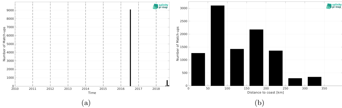
Figure 2: Number of match-ups between TSG (GOSUD-Research-vessel) and SMOS SSS L3 Arctic v2 - 9 Days (CATDS-CEC-LOCEAN) SSS as a function of time (a) and as function of the distance to coast (b) over the Arctic Ocean Pi-MEP region and for the full satellite product period.
