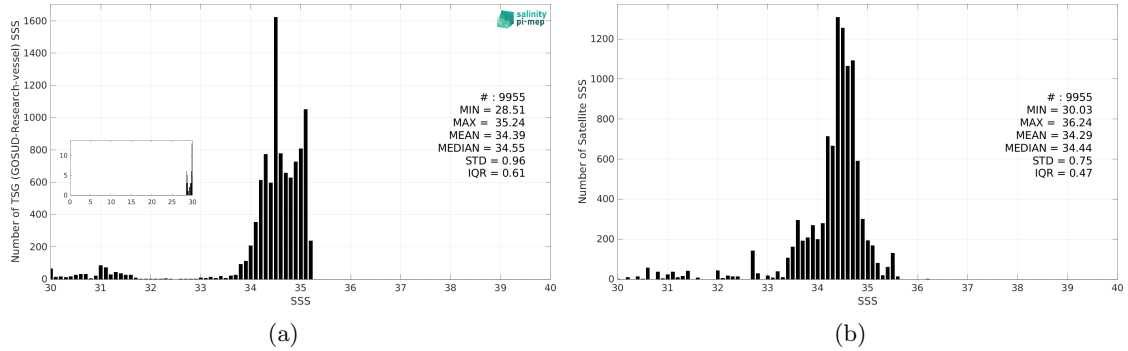
Figure 3: Histograms of SSS from TSG (GOSUD-Research-vessel) (a) and SMOS SSS L3 Arctic v2 - 9 Days (CATDS-CEC-LOCEAN) (b) considering all match-up pairs per bins of 0.1 over the Arctic Ocean Pi-MEP region and for the full satellite product period.
