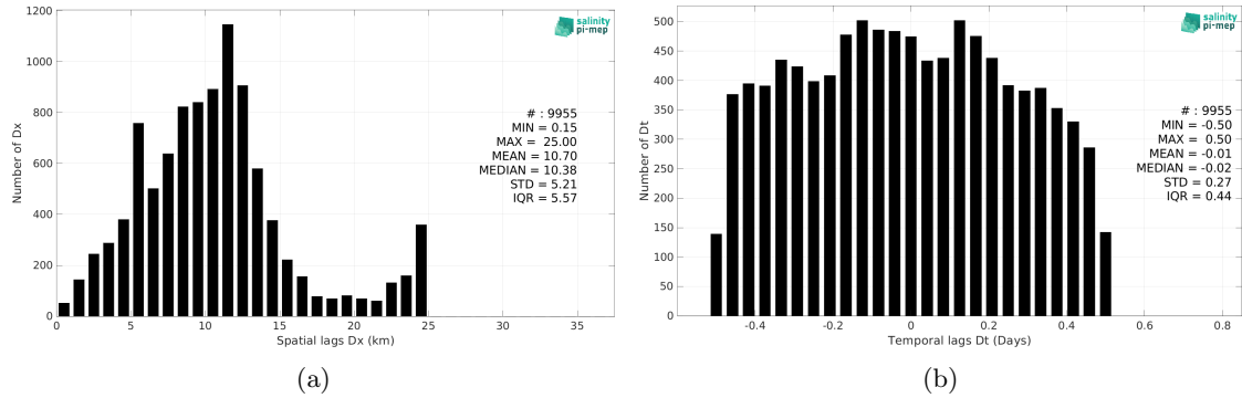
Figure 6: Histograms of the spatial (a) and temporal (b) lags between the location/time of the TSG (GOSUD-Research-vessel) measurement and the date of the corresponding SMOS SSS L3 Arctic v2 - 9 Days (CATDS-CEC-LOCEAN) SSS pixel.
