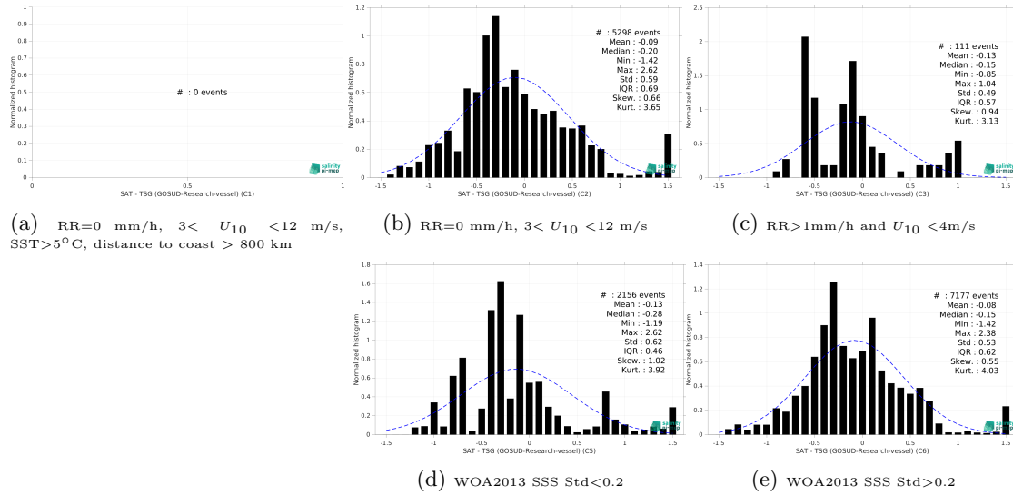
Figure 15: Normalized histogram of \Delta SSS (SMOS SSS L3 Arctic v2 - 9 Days (CATDS-CEC-LOCEAN) - TSG (GOSUD-Research-vessel)) for 5 different subdatasets corresponding to: RR=0 mm/h, 3 < U_{10} < 12 m/s, SST>5°C, distance to coast > 800 km (a), RR=0 mm/h, 3 < U_{10} < 12 m/s (b), RR>1mm/h and U_{10} < 4 m/s (c), WOA2013 SSS Std<0.2 (d), WOA2013 SSS Std>0.2 (e).
