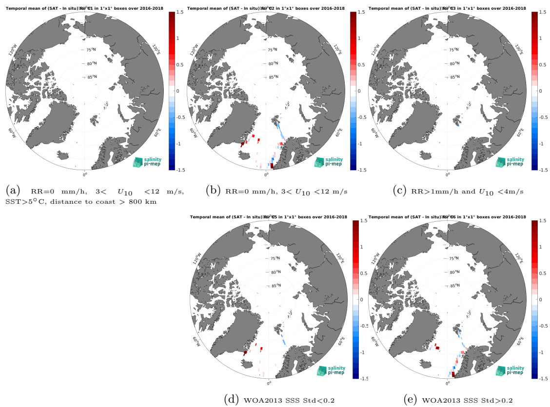
Figure 14: Temporal mean gridded over spatial boxes of size 1^\circ \times 1^\circ of \Delta\text{SSS} (SMOS SSS L3 Arctic v2 - 9 Days (CATDS-CEC-LOCEAN) - TSG (GOSUD-Research-vessel)) for 5 different subdatasets corresponding to: RR=0 mm/h, 3 < U_{10} < 12 m/s, SST > 5°C, distance to coast > 800 km (a), RR=0 mm/h, 3 < U_{10} < 12 m/s (b), RR > 1mm/h and U_{10} < 4 m/s (c), WOA2013 SSS Std < 0.2 (d), WOA2013 SSS Std > 0.2 (e).
