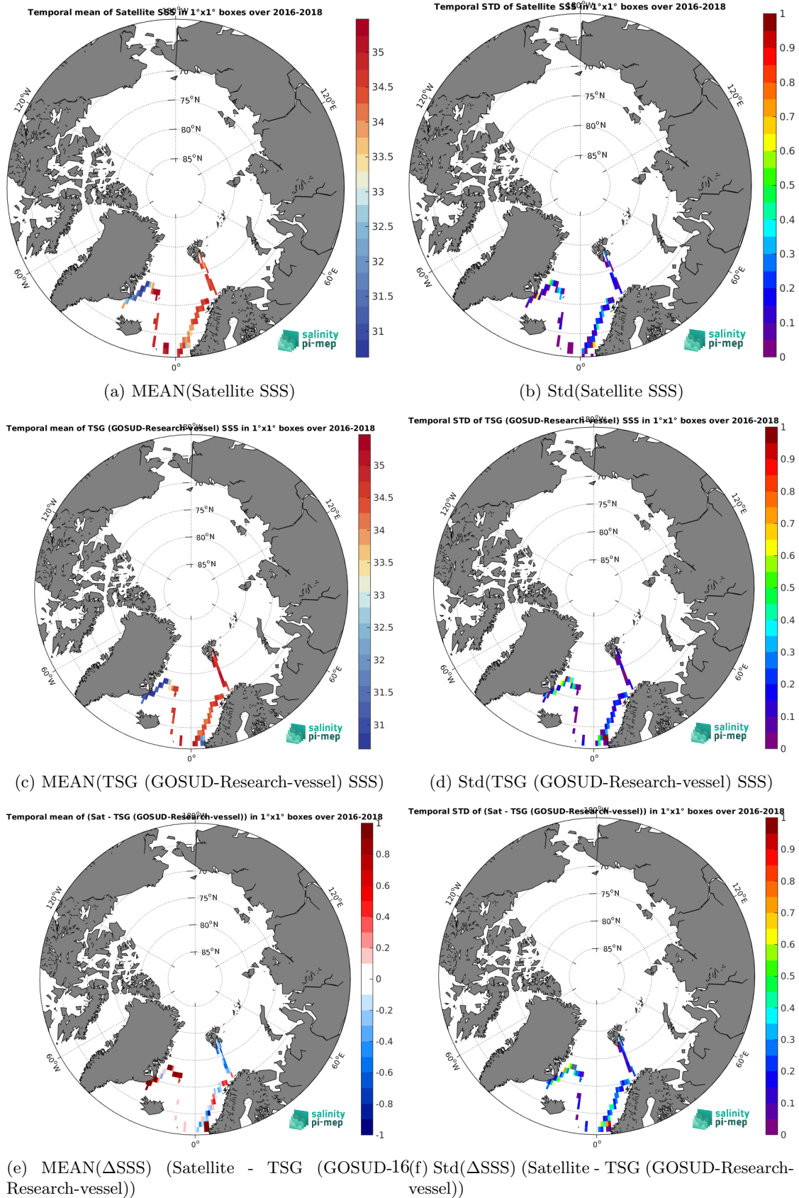
Figure 6: Temporal mean (left) and Std (right) of SSS from SMOS SSS L3 Arctic v2 - 9 Days (CATDS-CEC-LOCEAN) (top), TSG (GOSUD-Research-vessel) (middle), and of \Delta SSS (Satellite - TSG (GOSUD-Research-vessel)). Only match-up pairs are used to generate these maps.
