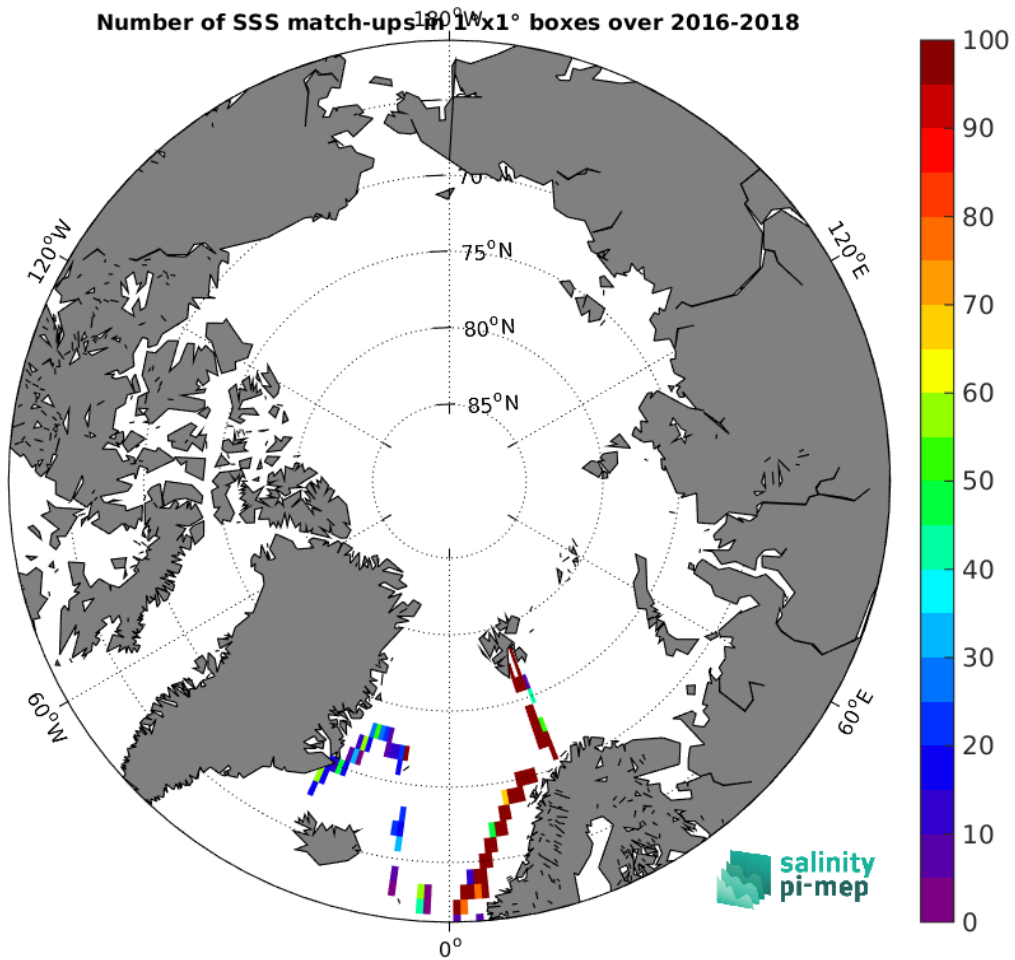
Figure 4: Number of SSS match-ups between TSG (GOSUD-Research-vessel) SSS and the SMOS SSS L3 Arctic v2 - 9 Days (CATDS-CEC-LOCEAN) SSS product for the Arctic Ocean Pi-MEP region over 1^\circ \times 1^\circ boxes and for the full satellite product period.
