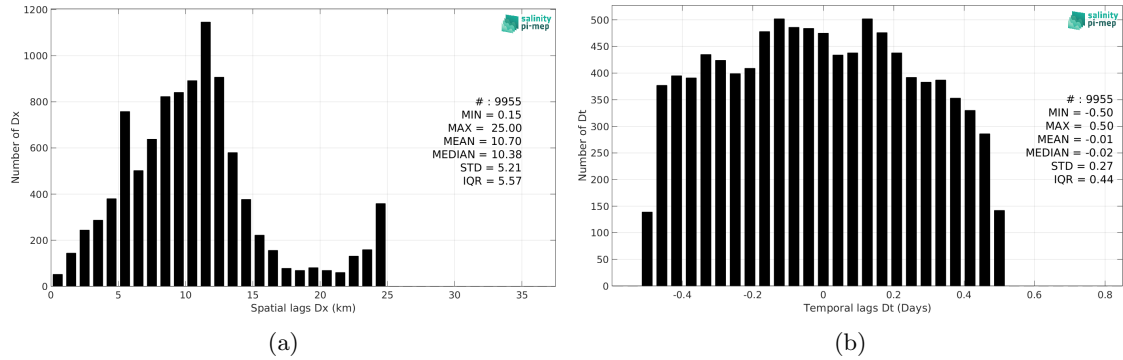
Figure 5: Histograms of the spatial (a) and temporal (b) lags between the location/time of the TSG (GOSUD-Research-vessel) measurement and the date of the corresponding SMOS SSS L3 Arctic v2 - 9 Days (CATDS-CEC-LOCEAN) SSS pixel.
