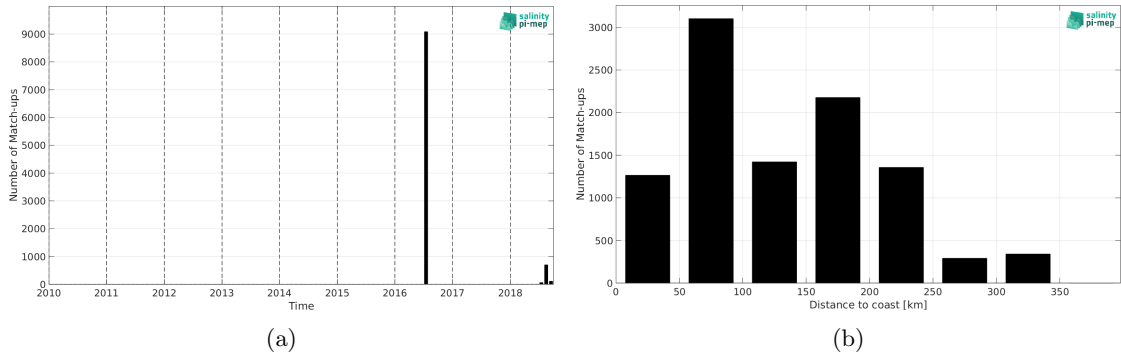
Figure 1: Number of match-ups between TSG (GOSUD-Research-vessel) and SMOS SSS L3 Arctic v2 - 9 Days (CATDS-CEC-LOCEAN) SSS as a function of time (a) and as function of the distance to coast (b) over the Arctic Ocean Pi-MEP region and for the full satellite product period.
