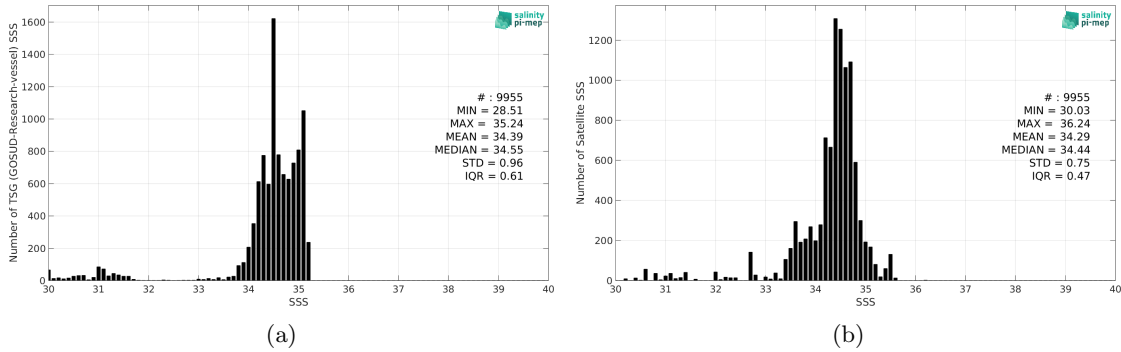
Figure 2: Histograms of SSS from TSG (GOSUD-Research-vessel) (a) and SMOS SSS L3 Arctic v2 - 9 Days (CATDS-CEC-LOCEAN) (b) considering all match-up pairs per bins of 0.1 over the Arctic Ocean Pi-MEP region and for the full satellite product period.
