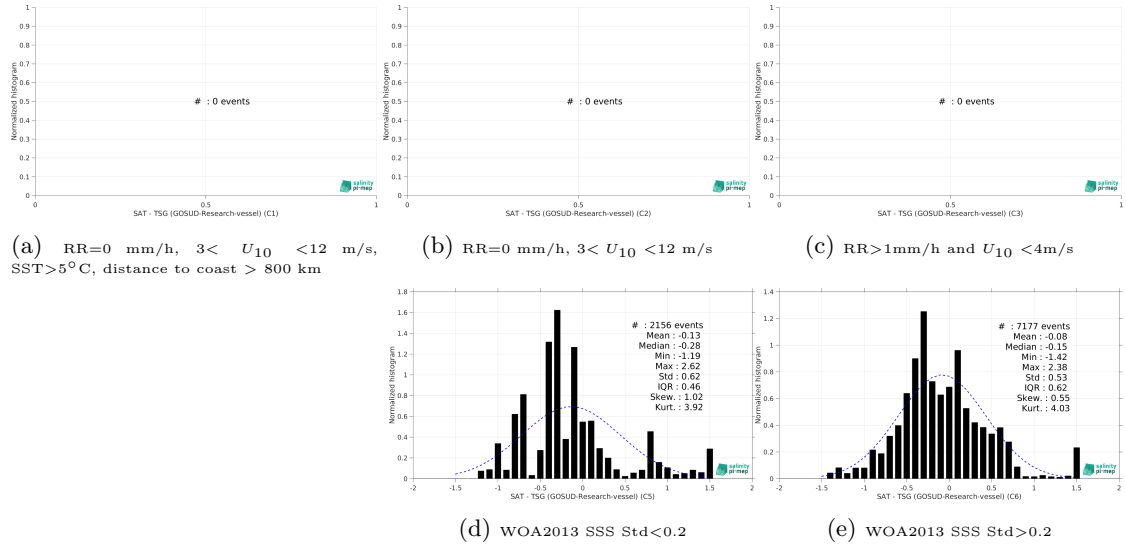
Figure 13: Normalized histogram of \Delta SSS (SMOS SSS L3 Arctic v2 - 9 Days (CATDS-CEC-LOCEAN) - TSG (GOSUD-Research-vessel)) for 5 different subdatasets corresponding to: RR=0 mm/h, 3 < U_{10} < 12 m/s, SST > 5°C, distance to coast > 800 km (a), RR=0 mm/h, 3 < U_{10} < 12 m/s (b), RR > 1mm/h and U_{10} < 4 m/s (c), WOA2013 SSS Std < 0.2 (d), WOA2013 SSS Std > 0.2 (e).
