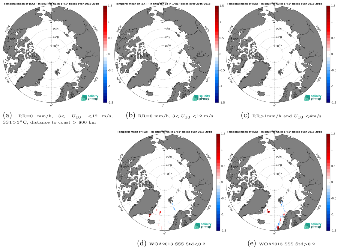
Figure 12: Temporal mean gridded over spatial boxes of size 1^\circ \times 1^\circ of \Delta\text{SSS} (SMOS SSS L3 Arctic v2 - 9 Days (CATDS-CEC-LOCEAN) - TSG (GOSUD-Research-vessel)) for 5 different subdatasets corresponding to: RR=0 mm/h, 3 < U_{10} < 12 m/s, SST > 5^\circ\text{C} , distance to coast > 800 km (a), RR=0 mm/h, 3 < U_{10} < 12 m/s (b), RR > 1 mm/h and U_{10} < 4 m/s (c), WOA2013 SSS Std < 0.2 (d), WOA2013 SSS Std > 0.2 (e).
