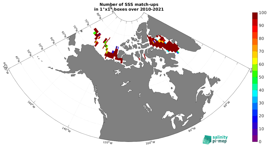
Figure 5: Number of SSS match-ups between TSG (Amundsen) SSS and the SMOS SSS L3 Arctic v2 - 9 Days (CATDS-CEC-LOCEAN) SSS product for the Arctic Ocean Pi-MEP region over 1°×1° boxes and for the full satellite product period.
