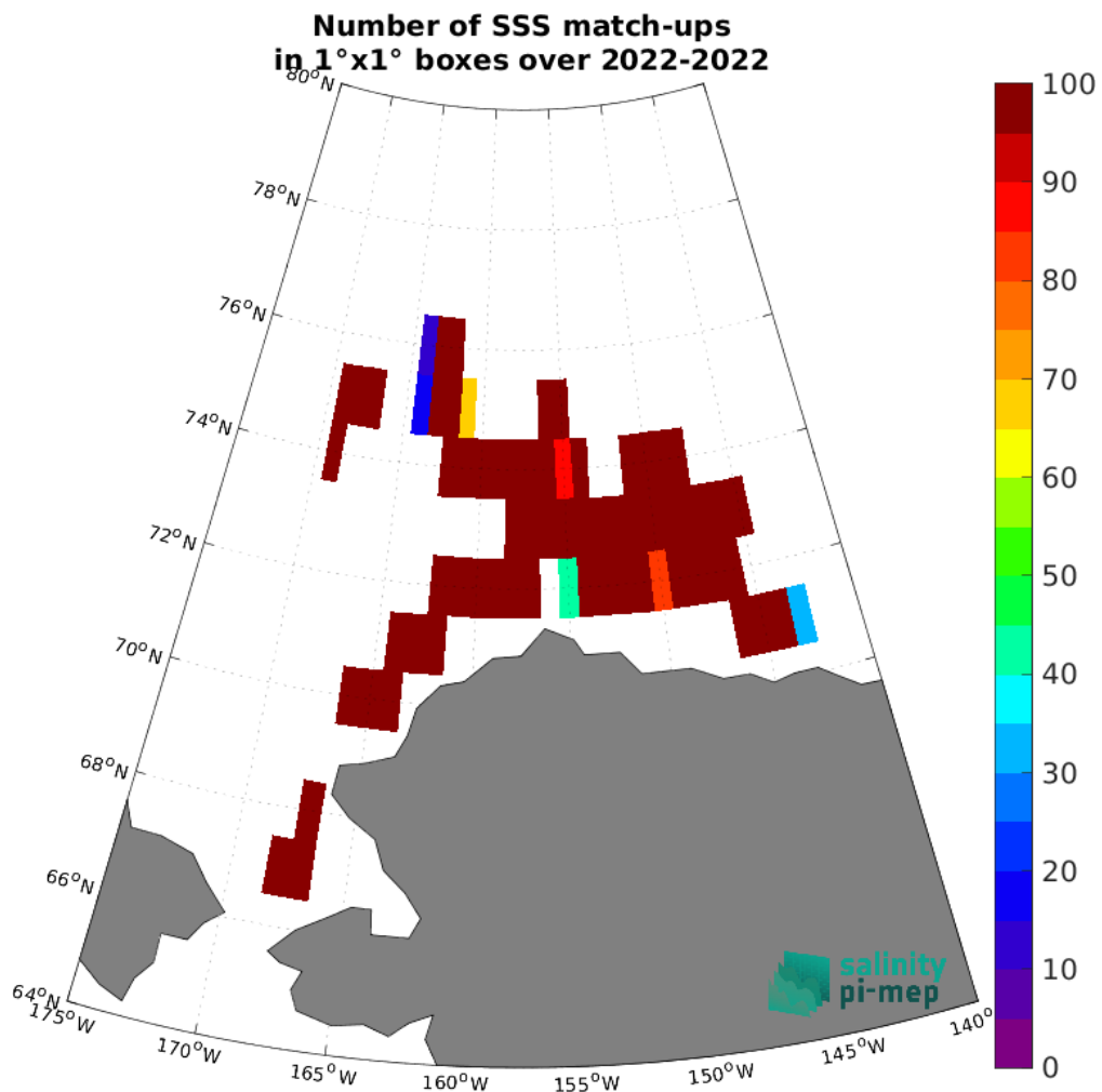
Figure 5: Number of SSS match-ups between SASSIE SSS and the SMOS SSS L3 Arctic v2 - 9 Days (CATDS-CEC-LOCEAN) SSS product for the Arctic Ocean Pi-MEP region over 1^\circ \times 1^\circ boxes and for the full satellite product period.
