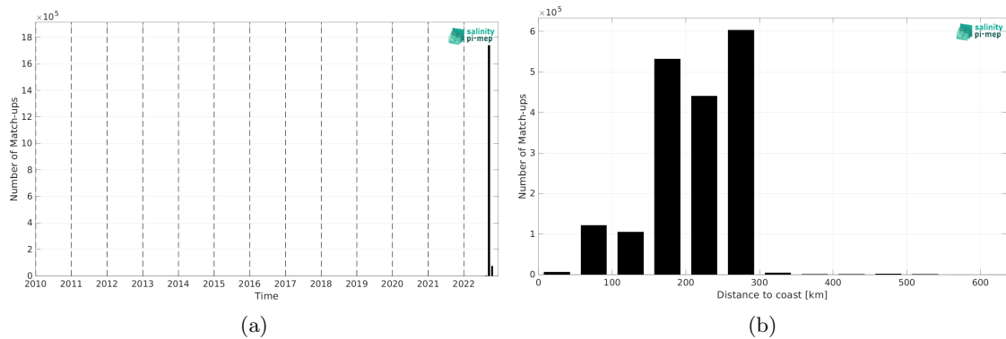
Figure 2: Number of match-ups between SASSIE and SMOS SSS L3 Arctic v2 - 9 Days (CATDS-CEC-LOCEAN) SSS as a function of time (a) and as function of the distance to coast (b) over the Arctic Ocean Pi-MEP region and for the full satellite product period.
