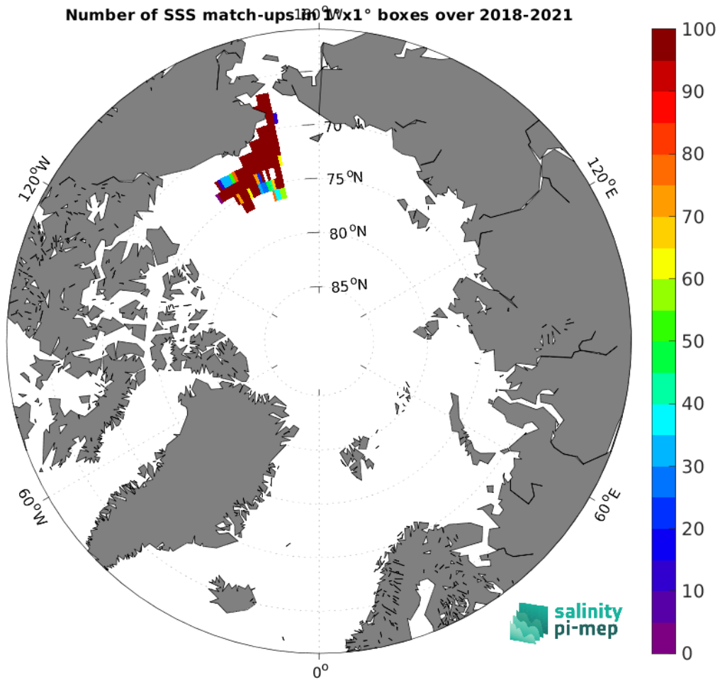
Figure 5: Number of SSS match-ups between Saildrone SSS and the SMOS SSS L3 Arctic v2 - 9 Days (CATDS-CEC-LOCEAN) SSS product for the Arctic Ocean Pi-MEP region over 1^\circ \times 1^\circ boxes and for the full satellite product period.
