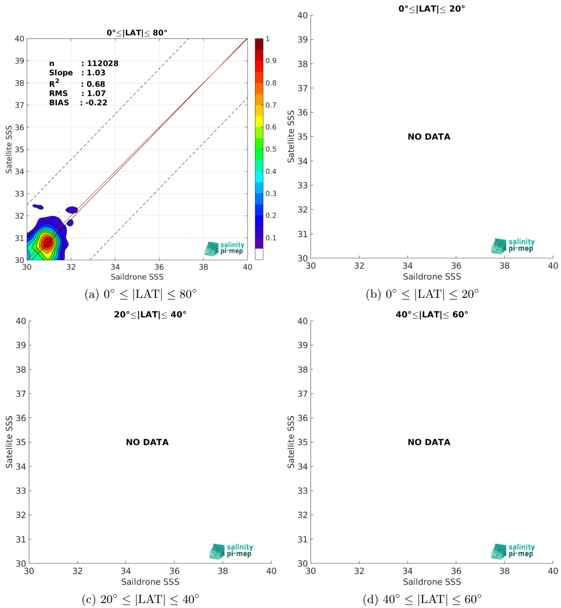
Figure 9: Contour maps of the concentration of SMOS SSS L3 Arctic v2 - 9 Days (CATDS-CEC-LOCEAN) SSS (y-axis) versus Sailldrone SSS (x-axis) at match-up pairs for different latitude bands. For each plot, the red line shows x=y . The black thin and dashed lines indicate a linear fit through the data cloud and the \pm 95\% confidence levels, respectively. The number match-up pairs n , the slope and R^2 coefficient of the linear fit, the root mean square (RMS) and the mean bias between satellite and in situ data are indicated for each latitude band in each plots.
