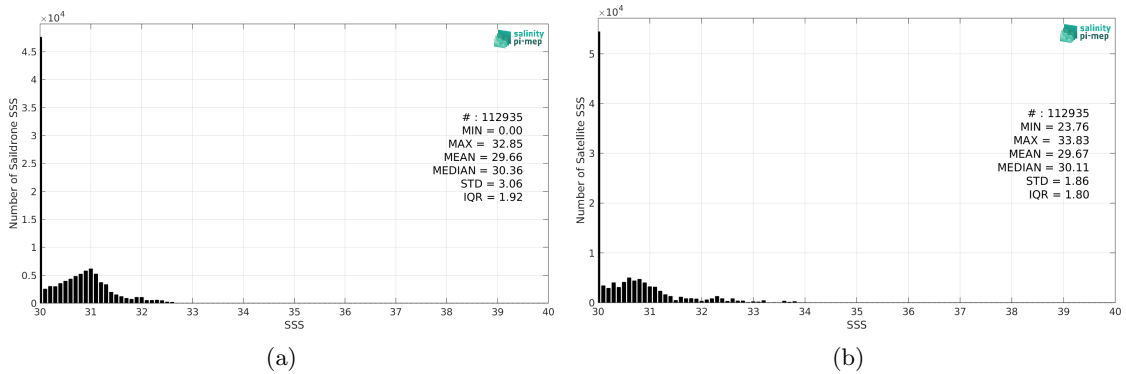
Figure 2: Histograms of SSS from Sailldrone (a) and SMOS SSS L3 Arctic v2 - 9 Days (CATDS-CEC-LOCEAN) (b) considering all match-up pairs per bins of 0.1 over the Arctic Ocean Pi-MEP region and for the full satellite product period.
