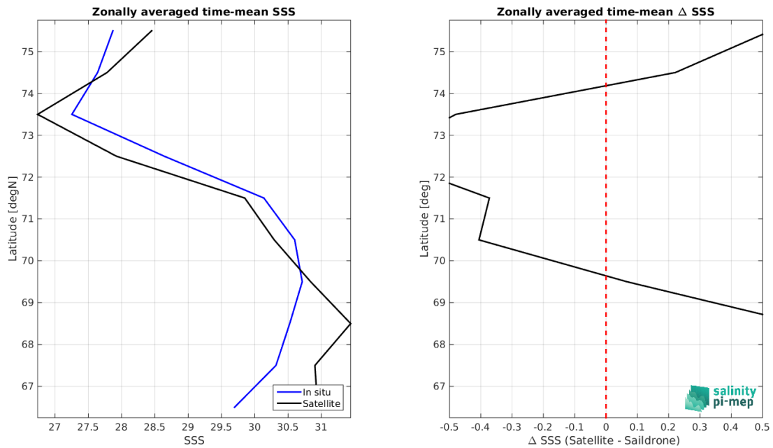
Figure 8: Left panel: Zonal mean SSS from SMOS SSS L3 Arctic v2 - 9 Days (CATDS-CEC-LOCEAN) satellite product (black) and from Saildrone (blue). Right panel: Zonal mean of \Delta SSS (Satellite - Saildrone) for all the collected Pi-MEP match-up pairs estimated over the full satellite product period.
