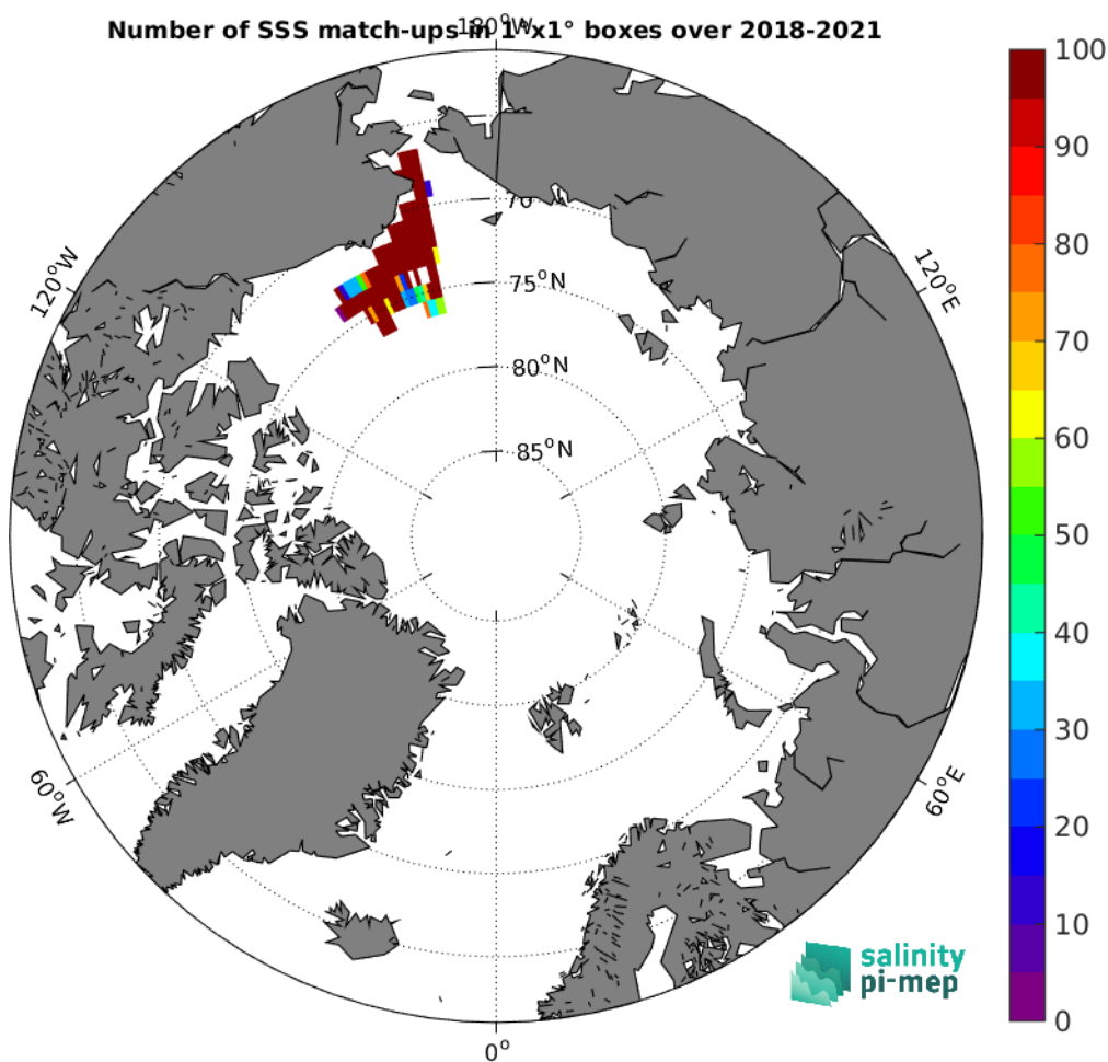
Figure 4: Number of SSS match-ups between Saildrone SSS and the SMOS SSS L3 Arctic v2 - 9 Days (CATDS-CEC-LOCEAN) SSS product for the Arctic Ocean Pi-MEP region over 1^\circ \times 1^\circ boxes and for the full satellite product period.
