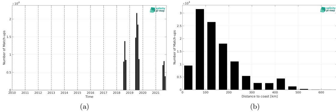
Figure 1: Number of match-ups between Sailldrone and SMOS SSS L3 Arctic v2 - 9 Days (CATDS-CEC-LOCEAN) SSS as a function of time (a) and as function of the distance to coast (b) over the Arctic Ocean Pi-MEP region and for the full satellite product period.
