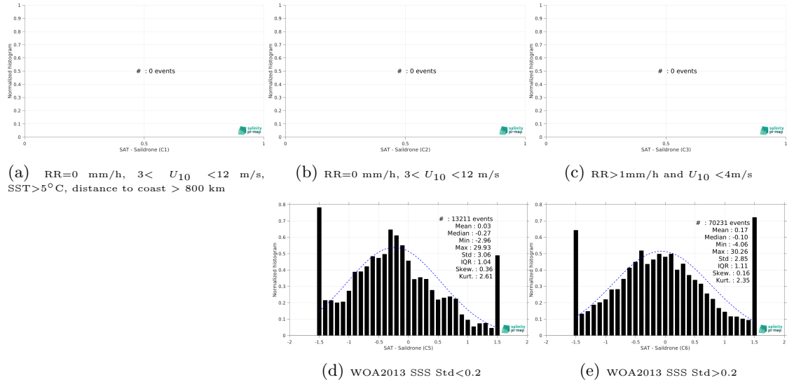
Figure 13: Normalized histogram of \Delta SSS (SMOS SSS L3 Arctic v2 - 9 Days (CATDS-CEC-LOCEAN) - Saildrone) for 5 different subdatasets corresponding to: RR=0 mm/h, 3 < U_{10} < 12 m/s, SST > 5°C, distance to coast > 800 km (a), RR=0 mm/h, 3 < U_{10} < 12 m/s (b), RR > 1mm/h and U_{10} < 4 m/s (c), WOA2013 SSS Std < 0.2 (d), WOA2013 SSS Std > 0.2 (e).
