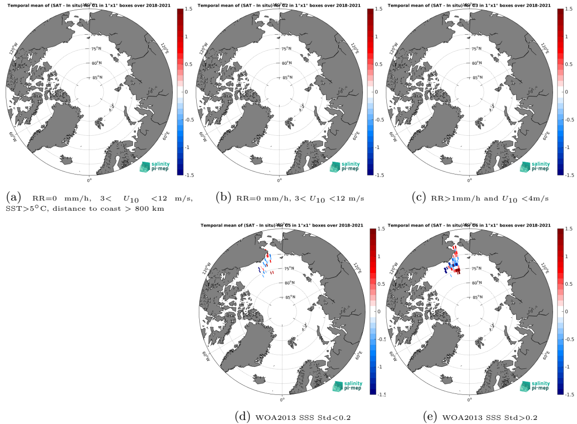
Figure 12: Temporal mean gridded over spatial boxes of size 1^{\circ}\times 1^{\circ} of \Delta\text{SSS} (SMOS SSS L3 Arctic v2 - 9 Days (CATDS-CEC-LOCEAN) - Saildrone) for 5 different subdatasets corresponding to:RR=0 mm/h, 3 < U_{10} < 12 m/s, SST > 5^{\circ}\text{C} , distance to coast > 800 km (a), RR=0 mm/h, 3 < U_{10} < 12 m/s (b), RR > 1 mm/h and U_{10} < 4 m/s (c), WOA2013 SSS Std < 0.2 (d), WOA2013 SSS Std > 0.2 (e).
