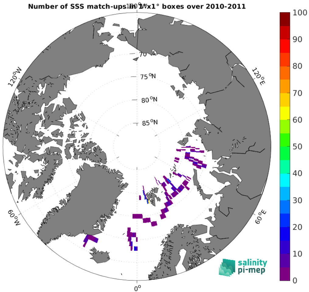
Figure 5: Number of SSS match-ups between Marine mammals SSS and the SMOS SSS L3 Arctic v2 - 9 Days (CATDS-CEC-LOCEAN) SSS product for the Arctic Ocean Pi-MEP region over 1^\circ \times 1^\circ boxes and for the full satellite product period.
