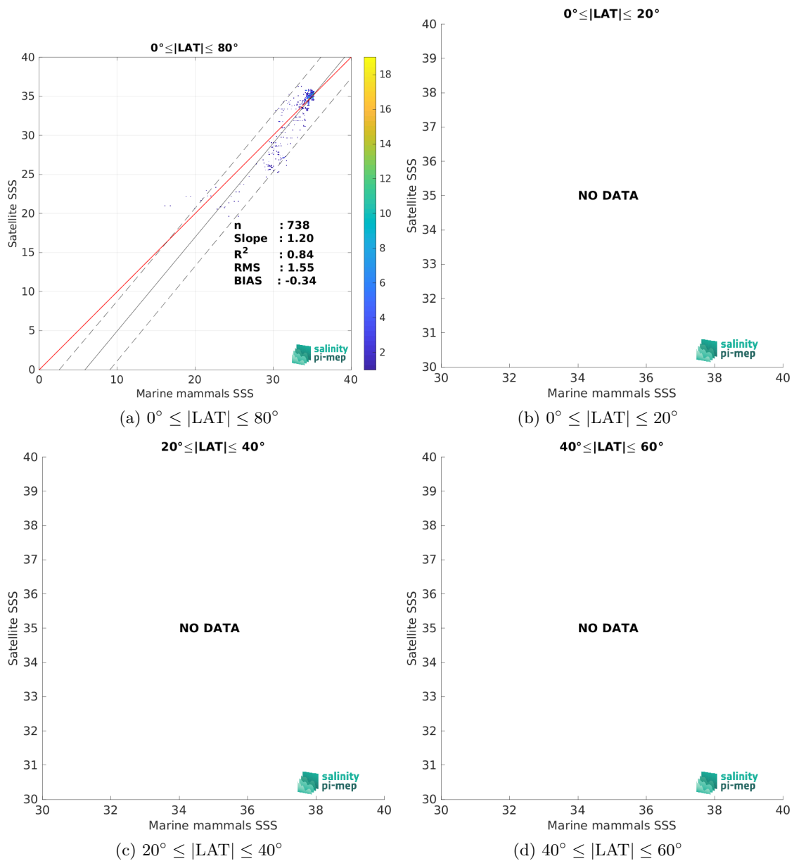
Figure 10: Contour maps of the concentration of SMOS SSS L3 Arctic v2 - 9 Days (CATDS-CEC-LOCEAN) SSS (y-axis) versus Marine mammals SSS (x-axis) at match-up pairs for different latitude bands. For each plot, the red line shows x=y . The black thin and dashed lines indicate a linear fit through the data cloud and the \pm 95\% confidence levels, respectively. The number match-up pairs n , the slope and R^2 coefficient of the linear fit, the root mean square (RMS) and the mean bias between satellite and in situ data are indicated for each latitude band in each plots.
