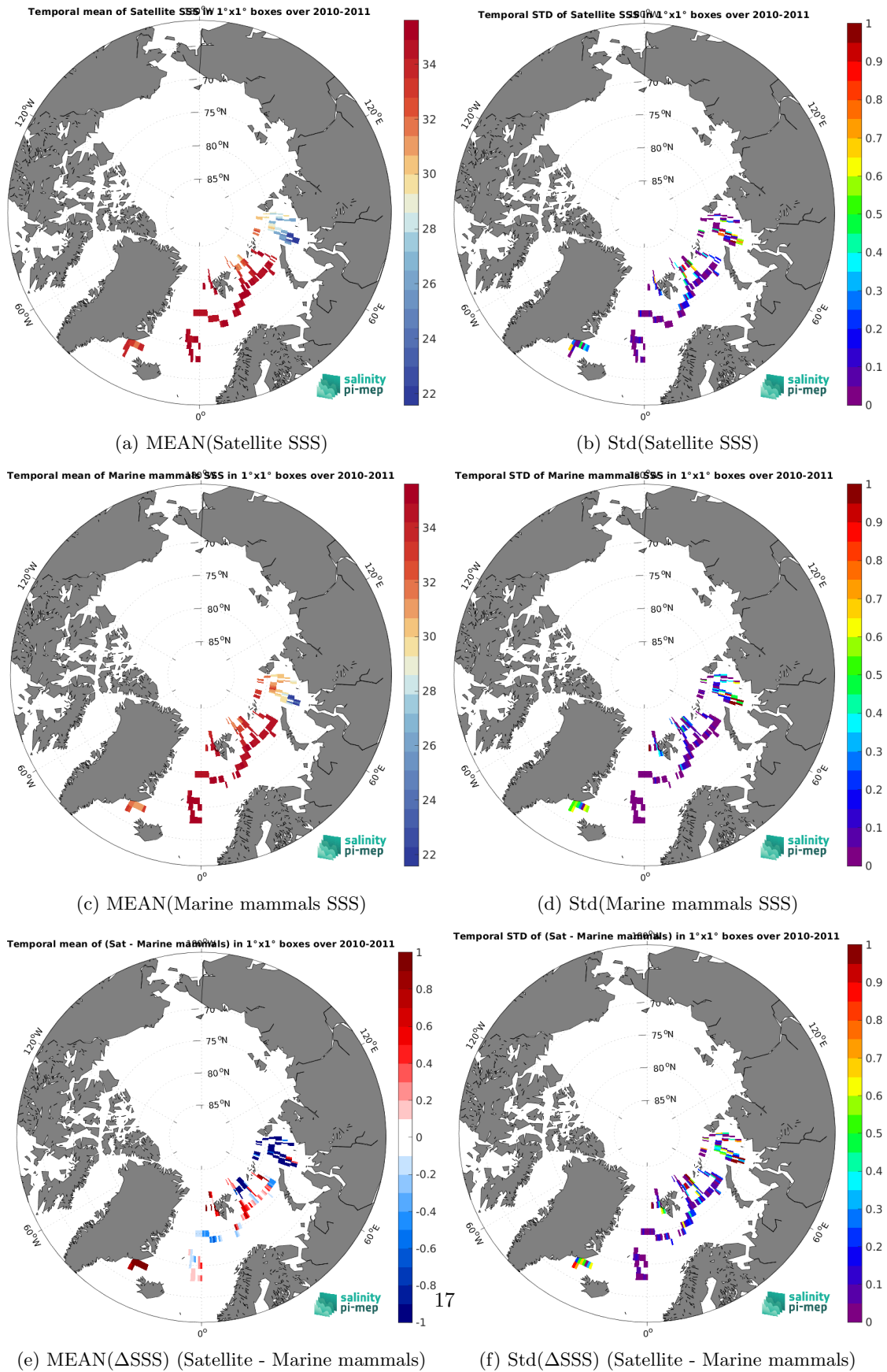
Figure 7: Temporal mean (left) and Std (right) of SSS from SMOS SSS L3 Arctic v2 - 9 Days (CATDS-CEC-LOCEAN) (top), Marine mammals (middle), and of \Delta SSS (Satellite - Marine mammals). Only match-up pairs are used to generate these maps.
