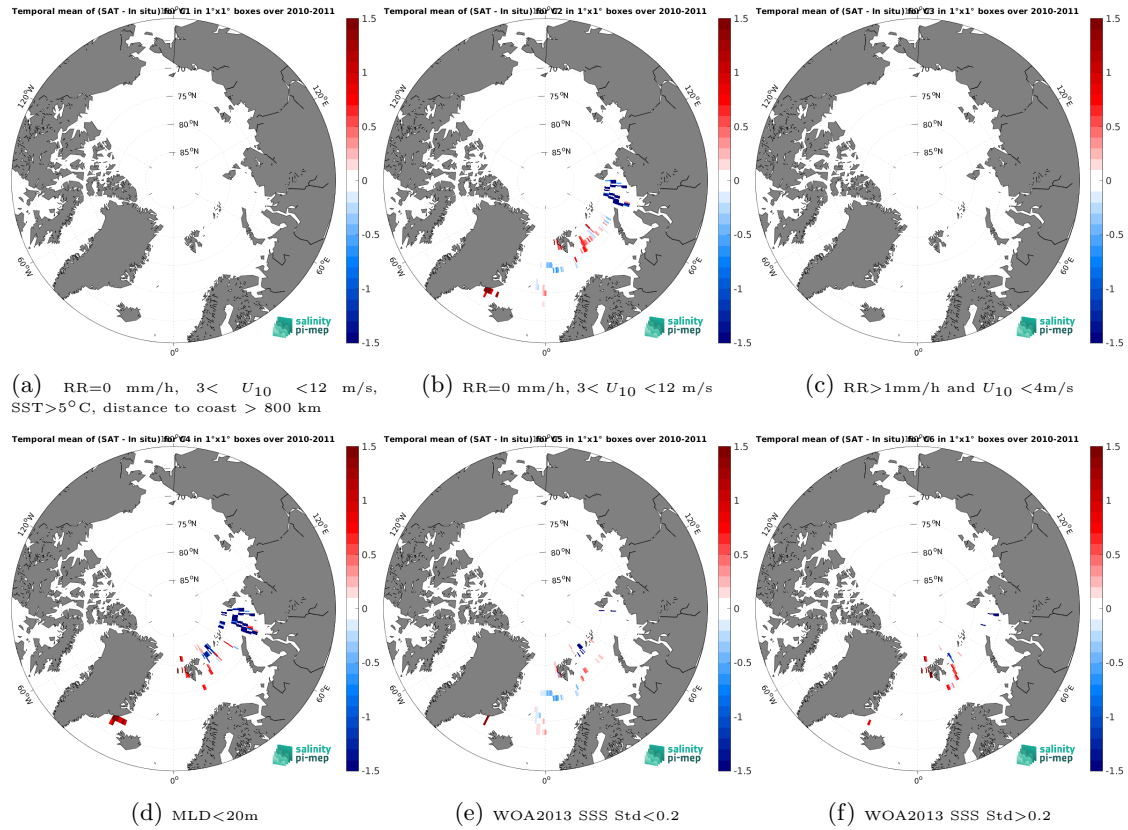
Figure 14: Temporal mean gridded over spatial boxes of size 1^\circ \times 1^\circ of \Delta SSS (SMOS SSS L3 Arctic v2 - 9 Days (CATDS-CEC-LOCEAN) - Marine mammals) for 6 different subdatasets corresponding to:RR=0 mm/h, 3 < U_{10} < 12 m/s, SST>5°C, distance to coast > 800 km (a), RR=0 mm/h, 3 < U_{10} < 12 m/s (b), RR>1mm/h and U_{10} < 4 m/s (c),MLD<20m (d),WOA2013 SSS Std<0.2 (e),WOA2013 SSS Std>0.2 (f).
