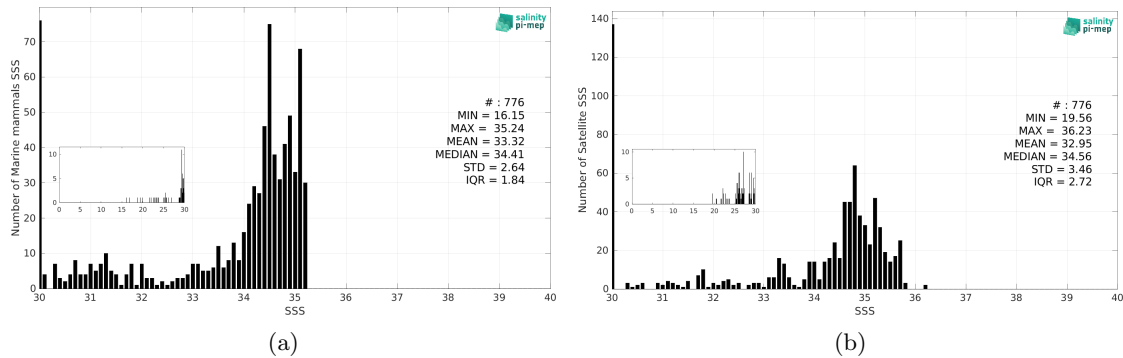
Figure 3: Histograms of SSS from Marine mammals (a) and SMOS SSS L3 Arctic v2 - 9 Days (CATDS-CEC-LOCEAN) (b) considering all match-up pairs per bins of 0.1 over the Arctic Ocean Pi-MEP region and for the full satellite product period.
