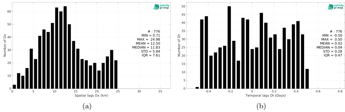
Figure 6: Histograms of the spatial (a) and temporal (b) lags between the location/time of the Marine mammals measurement and the date of the corresponding SMOS SSS L3 Arctic v2 - 9 Days (CATDS-CEC-LOCEAN) SSS pixel.
