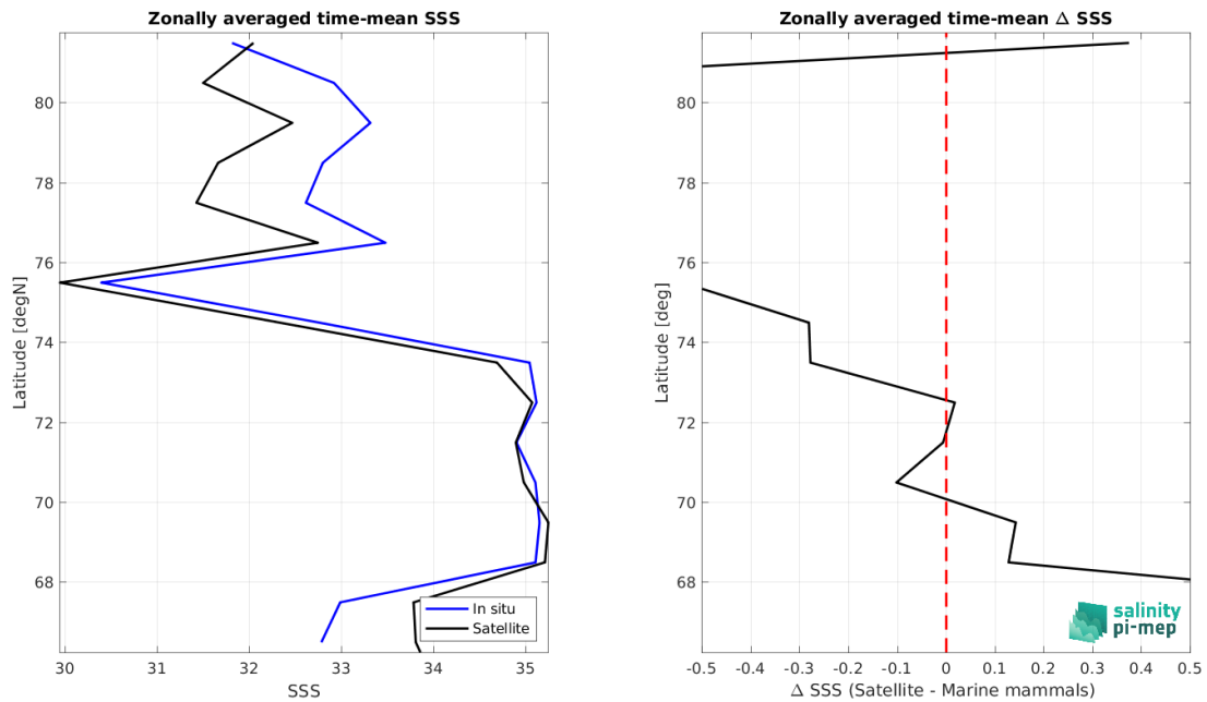
Figure 9: Left panel: Zonal mean SSS from SMOS SSS L3 Arctic v2 - 9 Days (CATDS-CEC-LOCEAN) satellite product (black) and from Marine mammals (blue). Right panel: Zonal mean of \Delta SSS (Satellite - Marine mammals) for all the collected Pi-MEP match-up pairs estimated over the full satellite product period.
