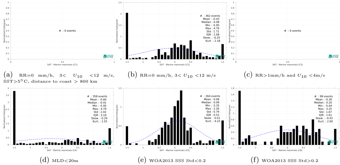
Figure 15: Normalized histogram of \Delta SSS (SMOS SSS L3 Arctic v2 - 9 Days (CATDS-CEC-LOCEAN) - Marine mammals) for 6 different subdatasets corresponding to: RR=0 mm/h, 3 < U_{10} < 12 m/s, SST>5°C, distance to coast > 800 km (a), RR=0 mm/h, 3 < U_{10} < 12 m/s (b), RR>1mm/h and U_{10} < 4 m/s (c), MLD<20m (d), WOA2013 SSS Std<0.2 (e), WOA2013 SSS Std>0.2 (f).
