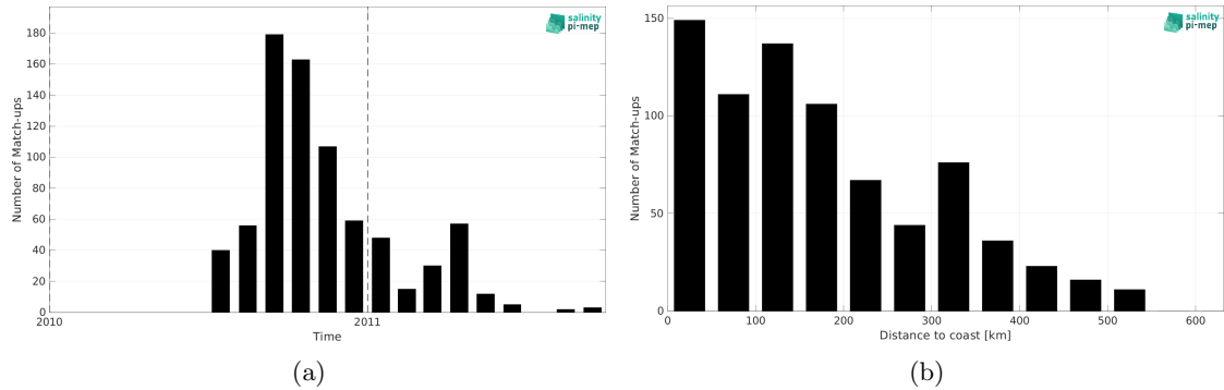
Figure 2: Number of match-ups between Marine mammals and SMOS SSS L3 Arctic v2 - 9 Days (CATDS-CEC-LOCEAN) SSS as a function of time (a) and as function of the distance to coast (b) over the Arctic Ocean Pi-MEP region and for the full satellite product period.
