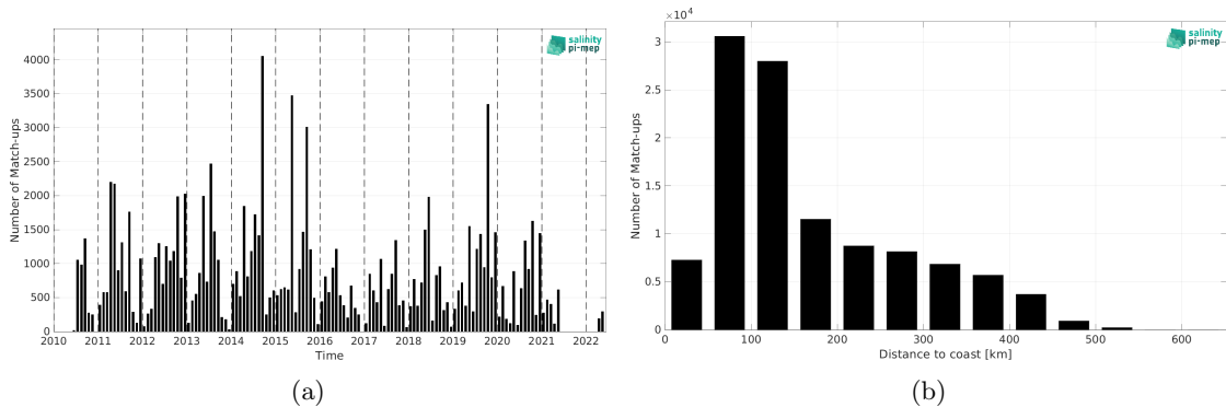
Figure 2: Number of match-ups between ICES and SMOS SSS L3 Arctic v2 - 9 Days (CATDS-CEC-LOCEAN) SSS as a function of time (a) and as function of the distance to coast (b) over the Arctic Ocean Pi-MEP region and for the full satellite product period.
