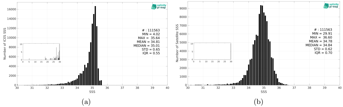
Figure 3: Histograms of SSS from ICES (a) and SMOS SSS L3 Arctic v2 - 9 Days (CATDS-CEC-LOCEAN) (b) considering all match-up pairs per bins of 0.1 over the Arctic Ocean Pi-MEP region and for the full satellite product period.
