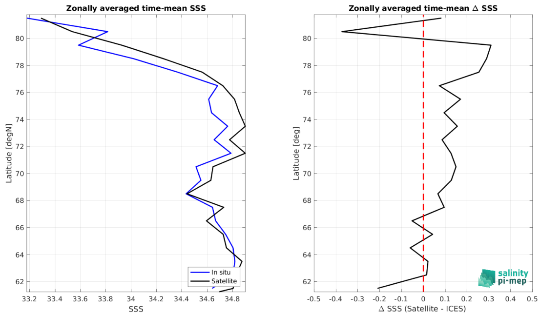
Figure 9: Left panel: Zonal mean SSS from SMOS SSS L3 Arctic v2 - 9 Days (CATDS-CEC-LOCEAN) satellite product (black) and from ICES (blue). Right panel: Zonal mean of \Delta SSS (Satellite - ICES) for all the collected Pi-MEP match-up pairs estimated over the full satellite product period.
