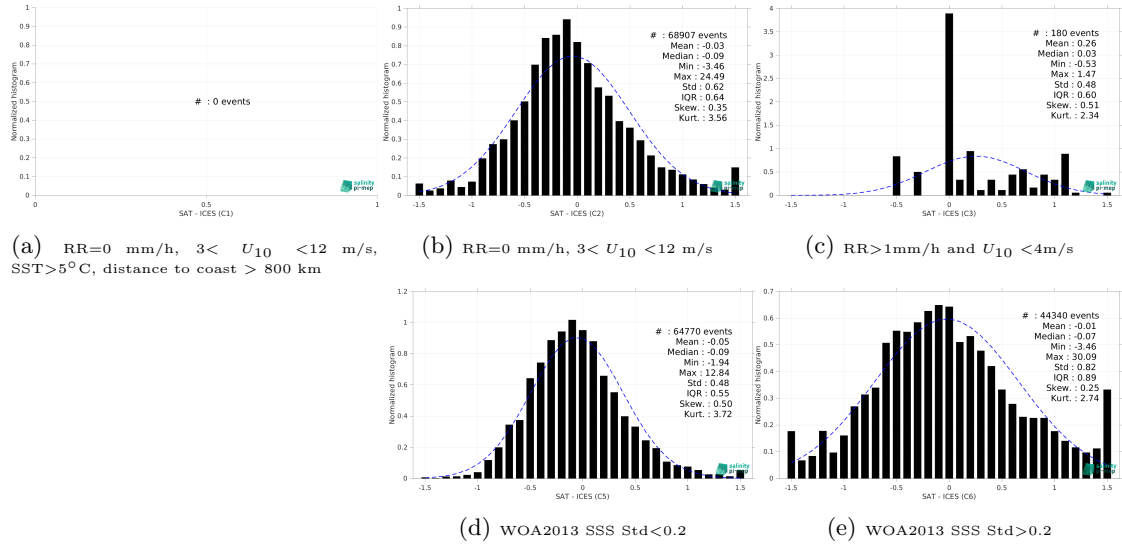
Figure 15: Normalized histogram of \Delta SSS (SMOS SSS L3 Arctic v2 - 9 Days (CATDS-CEC-LOCEAN) - ICES) for 5 different subdatasets corresponding to: RR=0 mm/h, 3 < U_{10} < 12 m/s, SST > 5°C, distance to coast > 800 km (a), RR=0 mm/h, 3 < U_{10} < 12 m/s (b), RR > 1mm/h and U_{10} < 4 m/s (c), WOA2013 SSS Std < 0.2 (d), WOA2013 SSS Std > 0.2 (e).
