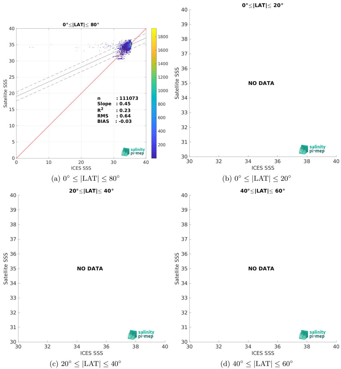
Figure 10: Contour maps of the concentration of SMOS SSS L3 Arctic v2 - 9 Days (CATDS-CEC-LOCEAN) SSS (y-axis) versus ICES SSS (x-axis) at match-up pairs for different latitude bands. For each plot, the red line shows x=y . The black thin and dashed lines indicate a linear fit through the data cloud and the \pm 95\% confidence levels, respectively. The number match-up pairs n , the slope and R^2 coefficient of the linear fit, the root mean square (RMS) and the mean bias between satellite and in situ data are indicated for each latitude band in each plots.
