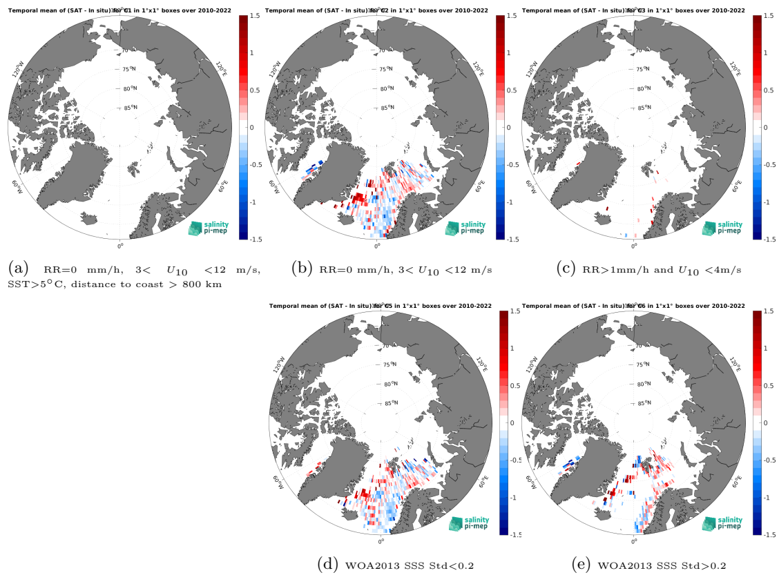
Figure 14: Temporal mean gridded over spatial boxes of size 1^\circ \times 1^\circ of \Delta\text{SSS} (SMOS SSS L3 Arctic v2 - 9 Days (CATDS-CEC-LOCEAN) - ICES) for 5 different subdatasets corresponding to:RR=0 mm/h, 3 < U_{10} < 12 m/s, SST>5°C, distance to coast > 800 km (a), RR=0 mm/h, 3 < U_{10} < 12 m/s (b), RR>1mm/h and U_{10} < 4 m/s (c), WOA2013 SSS Std<0.2 (d), WOA2013 SSS Std>0.2 (e).
