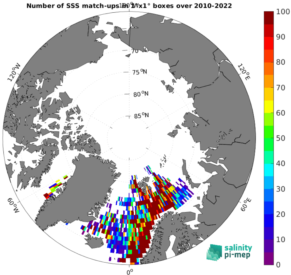
Figure 5: Number of SSS match-ups between ICES SSS and the SMOS SSS L3 Arctic v2 - 9 Days (CATDS-CEC-LOCEAN) SSS product for the Arctic Ocean Pi-MEP region over 1^\circ \times 1^\circ boxes and for the full satellite product period.
