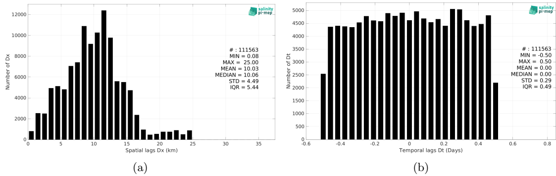
Figure 6: Histograms of the spatial (a) and temporal (b) lags between the location/time of the ICES measurement and the date of the corresponding SMOS SSS L3 Arctic v2 - 9 Days (CATDS-CEC-LOCEAN) SSS pixel.
