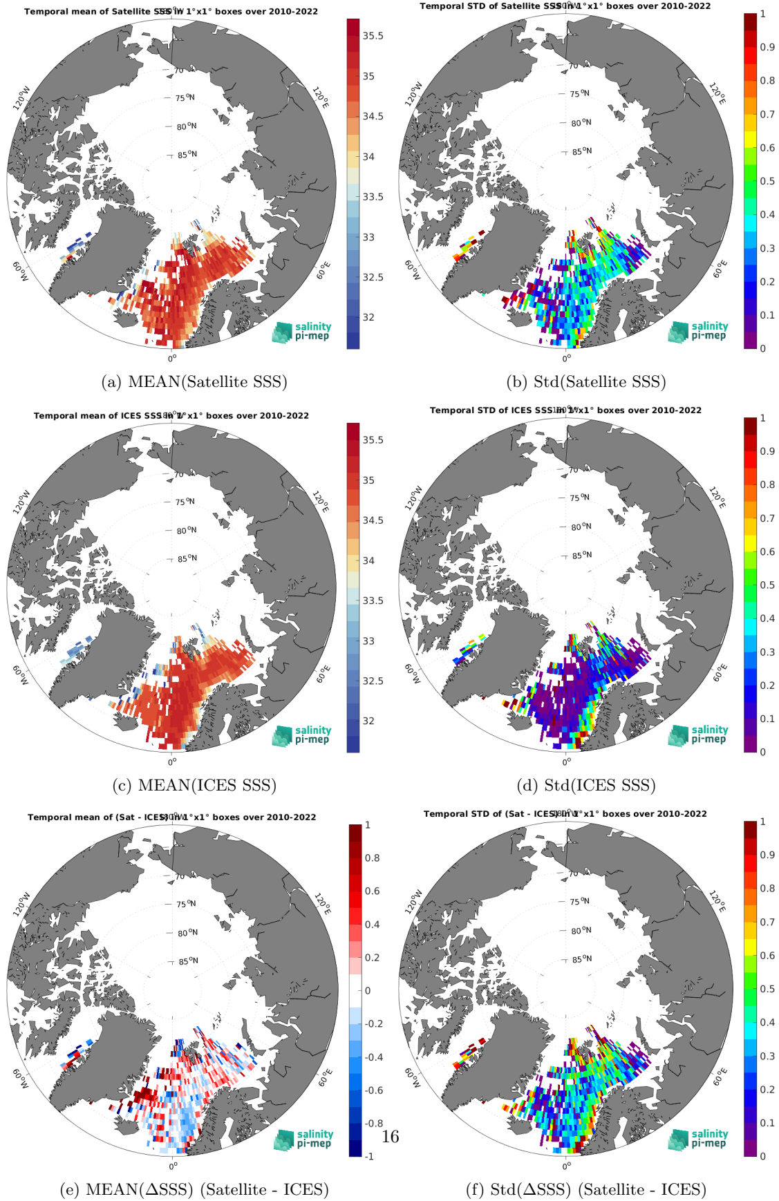
Figure 7: Temporal mean (left) and Std (right) of SSS from SMOS SSS L3 Arctic v2 - 9 Days (CATDS-CEC-LOCEAN) (top), ICES (middle), and of \Delta SSS (Satellite - ICES). Only match-up pairs are used to generate these maps.
