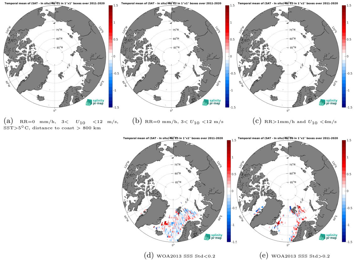
Figure 12: Temporal mean gridded over spatial boxes of size 1^{\circ}\times 1^{\circ} of \Delta\text{SSS} (SMOS SSS L3 Arctic v2 - 9 Days (CATDS-CEC-LOCEAN) - ICES) for 5 different subdatasets corresponding to:RR=0 mm/h, 3 < U_{10} < 12 m/s, SST >5^{\circ}\text{C} , distance to coast > 800 km (a), RR=0 mm/h, 3 < U_{10} < 12 m/s (b), RR >1 mm/h and U_{10} < 4 m/s (c), WOA2013 SSS Std <0.2 (d), WOA2013 SSS Std >0.2 (e).
