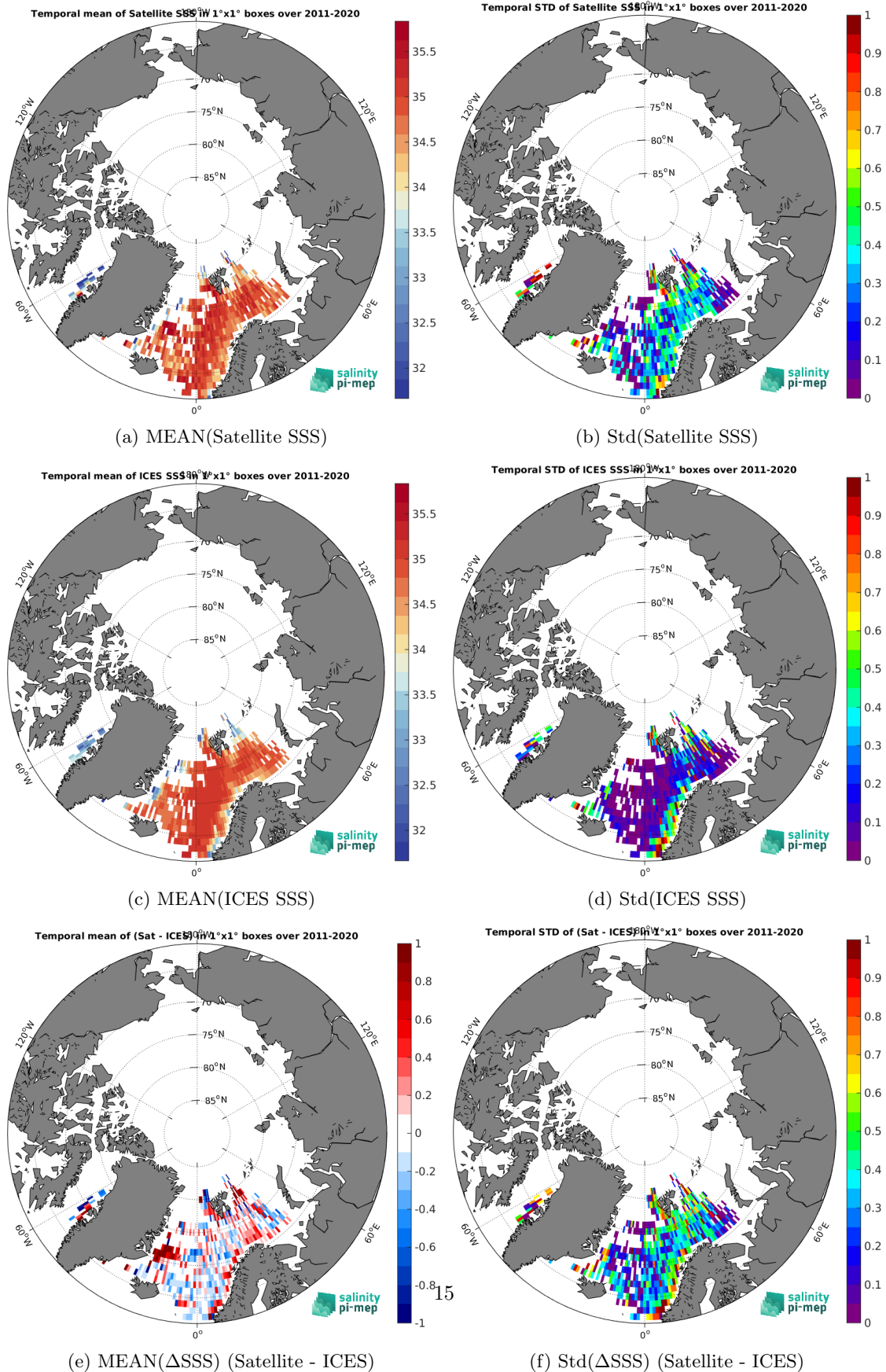
Figure 6: Temporal mean (left) and Std (right) of SSS from SMOS SSS L3 Arctic v2 - 9 Days (CATDS-CEC-LOCEAN) (top), ICES (middle), and of \Delta SSS (Satellite - ICES). Only match-up pairs are used to generate these maps.
