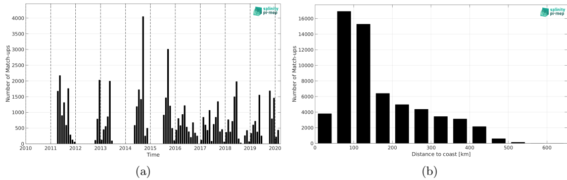
Figure 1: Number of match-ups between ICES and SMOS SSS L3 Arctic v2 - 9 Days (CATDS-CEC-LOCEAN) SSS as a function of time (a) and as function of the distance to coast (b) over the Arctic Ocean Pi-MEP region and for the full satellite product period.
