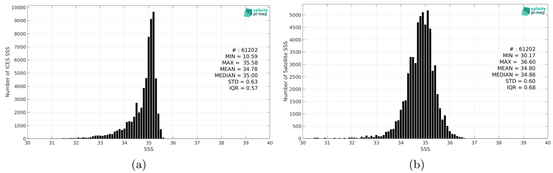
Figure 2: Histograms of SSS from ICES (a) and SMOS SSS L3 Arctic v2 - 9 Days (CATDS-CEC-LOCEAN) (b) considering all match-up pairs per bins of 0.1 over the Arctic Ocean Pi-MEP region and for the full satellite product period.
