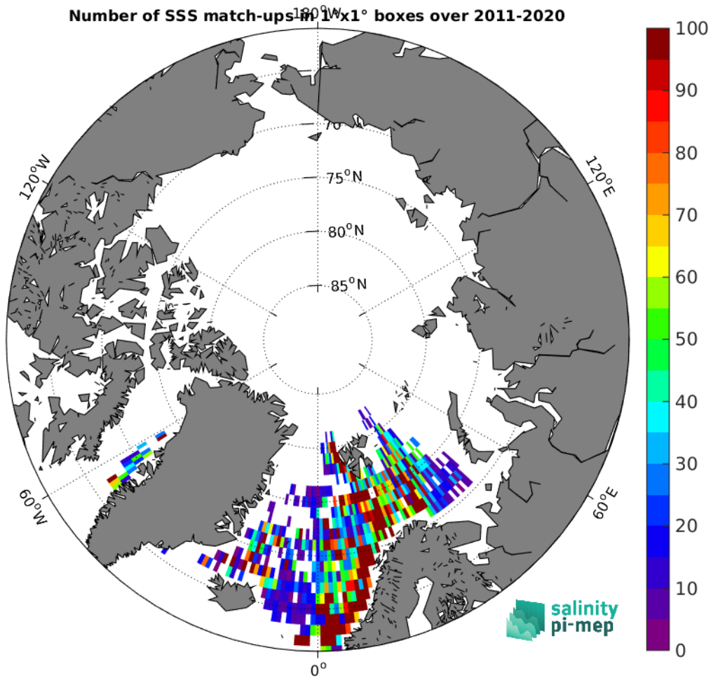
Figure 4: Number of SSS match-ups between ICES SSS and the SMOS SSS L3 Arctic v2 - 9 Days (CATDS-CEC-LOCEAN) SSS product for the Arctic Ocean Pi-MEP region over 1^\circ \times 1^\circ boxes and for the full satellite product period.
