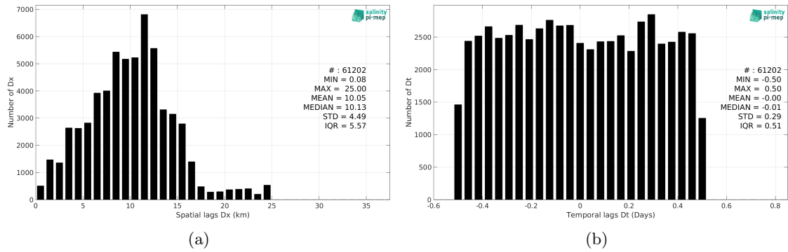
Figure 5: Histograms of the spatial (a) and temporal (b) lags between the location/time of the ICES measurement and the date of the corresponding SMOS SSS L3 Arctic v2 - 9 Days (CATDS-CEC-LOCEAN) SSS pixel.
