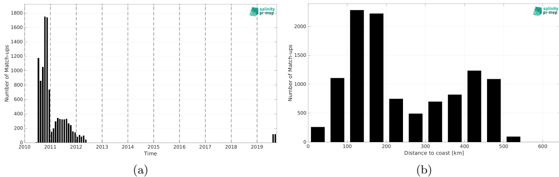
Figure 2: Number of match-ups between Surface drifters and SMOS SSS L3 Arctic v2 - 9 Days (CATDS-CEC-LOCEAN) SSS as a function of time (a) and as function of the distance to coast (b) over the Arctic Ocean Pi-MEP region and for the full satellite product period.
