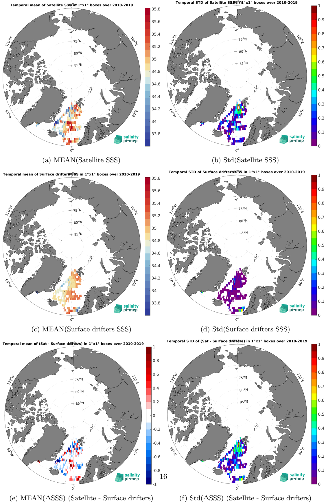
Figure 6: Temporal mean (left) and Std (right) of SSS from SMOS SSS L3 Arctic v2 - 9 Days (CATDS-CEC-LOCEAN) (top), Surface drifters (middle), and of \Delta SSS (Satellite - Surface drifters). Only match-up pairs are used to generate these maps.
