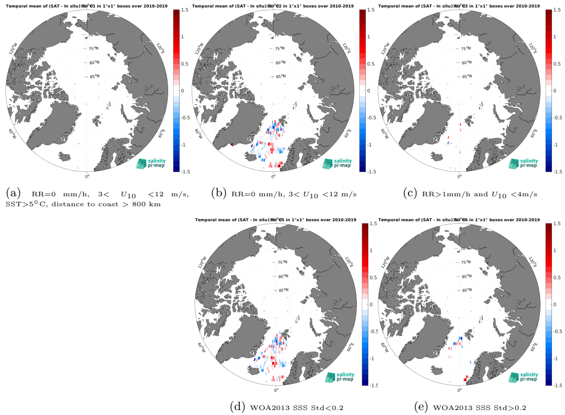
Figure 13: Temporal mean gridded over spatial boxes of size 1^\circ \times 1^\circ of \Delta SSS (SMOS SSS L3 Arctic v2 - 9 Days (CATDS-CEC-LOCEAN) - Surface drifters) for 5 different subdatasets corresponding to:RR=0 mm/h, 3 < U_{10} < 12 m/s, SST >5^\circ C, distance to coast > 800 km (a), RR=0 mm/h, 3 < U_{10} < 12 m/s (b), RR >1 mm/h and U_{10} < 4 m/s (c), WOA2013 SSS Std <0.2 (d), WOA2013 SSS Std >0.2 (e).
