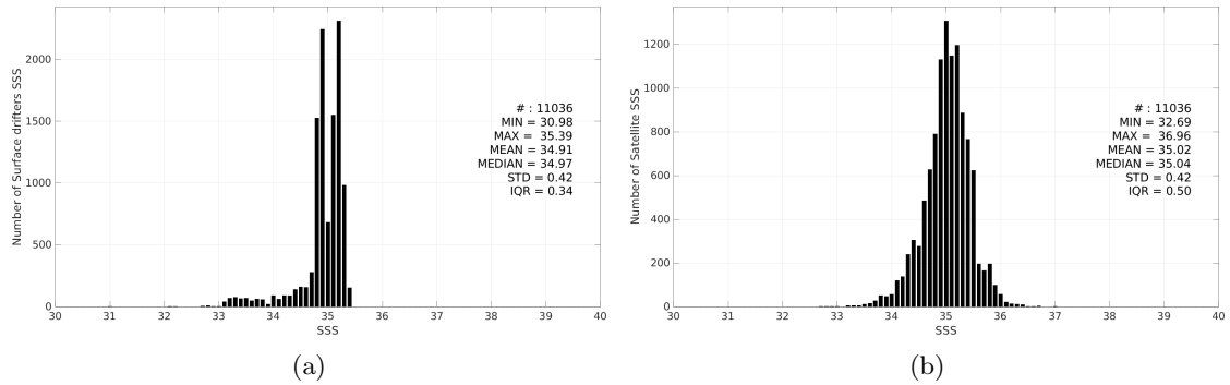
Figure 3: Histograms of SSS from Surface drifters (a) and SMOS SSS L3 Arctic v2 - 9 Days (CATDS-CEC-LOCEAN) (b) considering all match-up pairs per bins of 0.1 over the Arctic Ocean Pi-MEP region and for the full satellite product period.
