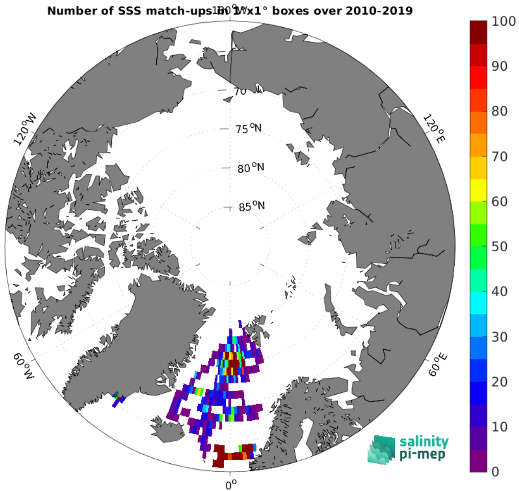
Figure 4: Number of SSS match-ups between Surface drifters SSS and the SMOS SSS L3 Arctic v2 - 9 Days (CATDS-CEC-LOCEAN) SSS product for the Arctic Ocean Pi-MEP region over 1^\circ \times 1^\circ boxes and for the full satellite product period.
