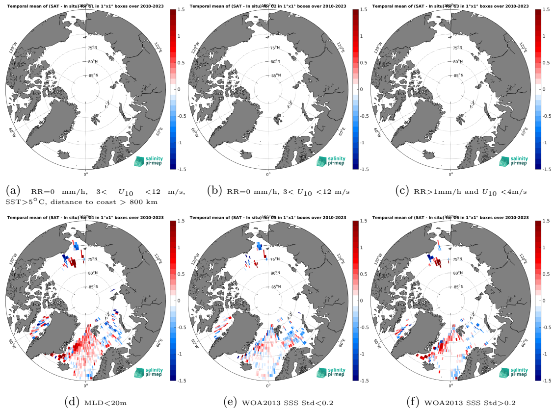
Figure 12: Temporal mean gridded over spatial boxes of size 1^{\circ}\times 1^{\circ} of \Delta\text{SSS} (SMOS SSS L3 Arctic v2 - 9 Days (CATDS-CEC-LOCEAN) - Argo) for 6 different subdatasets corresponding to: RR=0 mm/h, 3 < U_{10} < 12 m/s, SST > 5^{\circ}\text{C} , distance to coast > 800 km (a), RR=0 mm/h, 3 < U_{10} < 12 m/s (b), RR > 1\text{mm/h} and U_{10} < 4\text{m/s} (c), MLD < 20\text{m} (d), WOA2013 SSS Std < 0.2 (e), WOA2013 SSS Std > 0.2 (f).
