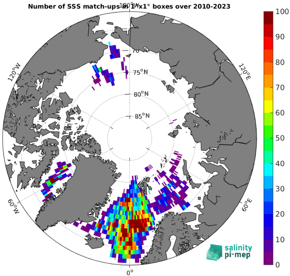
Figure 4: Number of SSS match-ups between Argo SSS and the SMOS SSS L3 Arctic v2 - 9 Days (CATDS-CEC-LOCEAN) SSS product for the Arctic Ocean Pi-MEP region over 1^\circ \times 1^\circ boxes and for the full satellite product period.
