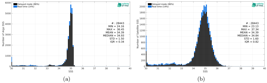
Figure 2: Histograms of SSS from Argo (a) and SMOS SSS L3 Arctic v2 - 9 Days (CATDS-CEC-LOCEAN) (b) considering all match-up pairs per bins of 0.1 over the Arctic Ocean Pi-MEP region and for the full satellite product period.
