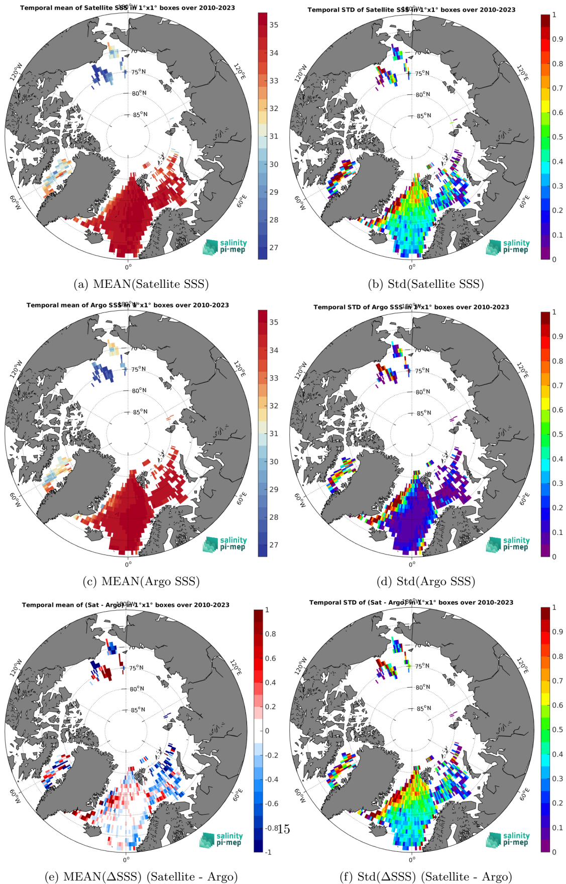
Figure 6: Temporal mean (left) and Std (right) of SSS from SMOS SSS L3 Arctic v2 - 9 Days (CATDS-CEC-LOCEAN) (top), Argo (middle), and of \Delta SSS (Satellite - Argo). Only match-up pairs are used to generate these maps.
