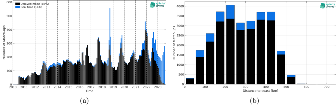
Figure 1: Number of match-ups between Argo and SMOS SSS L3 Arctic v2 - 9 Days (CATDS-CEC-LOCEAN) SSS as a function of time (a) and as function of the distance to coast (b) over the Arctic Ocean Pi-MEP region and for the full satellite product period.
