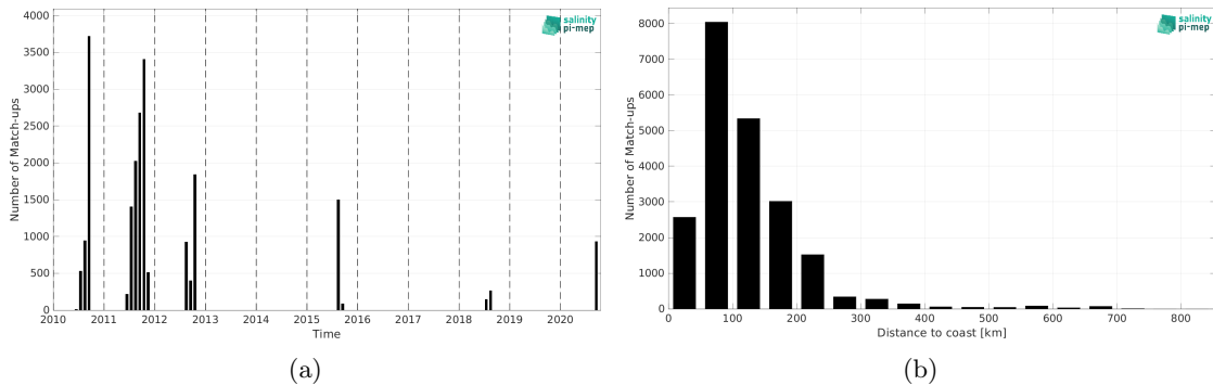
Figure 2: Number of match-ups between TSG (SAMOS) and SMOS SSS L3 Arctic v2 - 18 Days (CATDS-CEC-LOCEAN) SSS as a function of time (a) and as function of the distance to coast (b) over the Arctic Ocean Pi-MEP region and for the full satellite product period.
