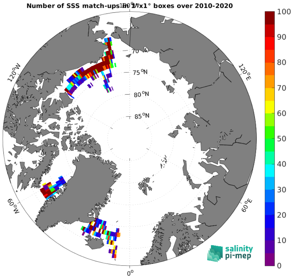
Figure 5: Number of SSS match-ups between TSG (SAMOS) SSS and the SMOS SSS L3 Arctic v2 - 18 Days (CATDS-CEC-LOCEAN) SSS product for the Arctic Ocean Pi-MEP region over 1^\circ \times 1^\circ boxes and for the full satellite product period.
