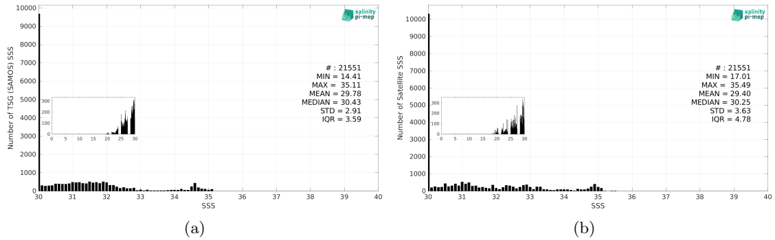
Figure 3: Histograms of SSS from TSG (SAMOS) (a) and SMOS SSS L3 Arctic v2 - 18 Days (CATDS-CEC-LOCEAN) (b) considering all match-up pairs per bins of 0.1 over the Arctic Ocean Pi-MEP region and for the full satellite product period.
