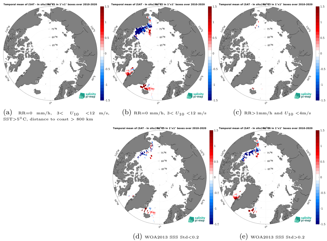
Figure 14: Temporal mean gridded over spatial boxes of size 1^\circ \times 1^\circ of \Delta SSS (SMOS SSS L3 Arctic v2 - 18 Days (CATDS-CEC-LOCEAN) - TSG (SAMOS)) for 5 different subdatasets corresponding to: RR=0 mm/h, 3 < U_{10} < 12 m/s, SST>5°C, distance to coast > 800 km (a), RR=0 mm/h, 3 < U_{10} < 12 m/s (b), RR>1mm/h and U_{10} < 4 m/s (c), WOA2013 SSS Std<0.2 (d), WOA2013 SSS Std>0.2 (e).
