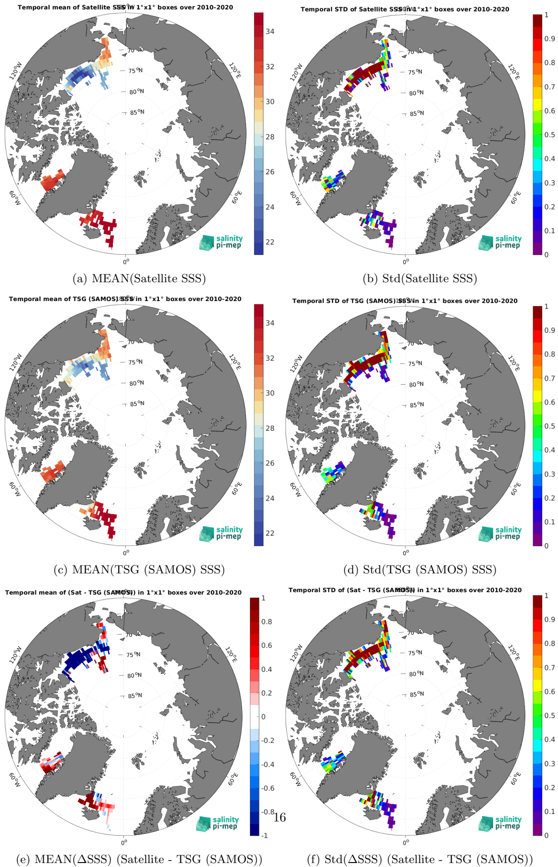
Figure 7: Temporal mean (left) and Std (right) of SSS from SMOS SSS L3 Arctic v2 - 18 Days (CATDS-CEC-LOCEAN) (top), TSG (SAMOS) (middle), and of \Delta SSS (Satellite - TSG (SAMOS)). Only match-up pairs are used to generate these maps.
