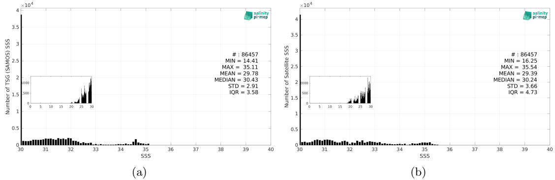
Figure 3: Histograms of SSS from TSG (SAMOS) (a) and SMOS SSS L3 Arctic v2 - 18 Days (CATDS-CEC-LOCEAN) (b) considering all match-up pairs per bins of 0.1 over the Arctic Ocean Pi-MEP region and for the full satellite product period.
