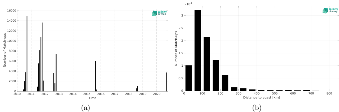
Figure 2: Number of match-ups between TSG (SAMOS) and SMOS SSS L3 Arctic v2 - 18 Days (CATDS-CEC-LOCEAN) SSS as a function of time (a) and as function of the distance to coast (b) over the Arctic Ocean Pi-MEP region and for the full satellite product period.
