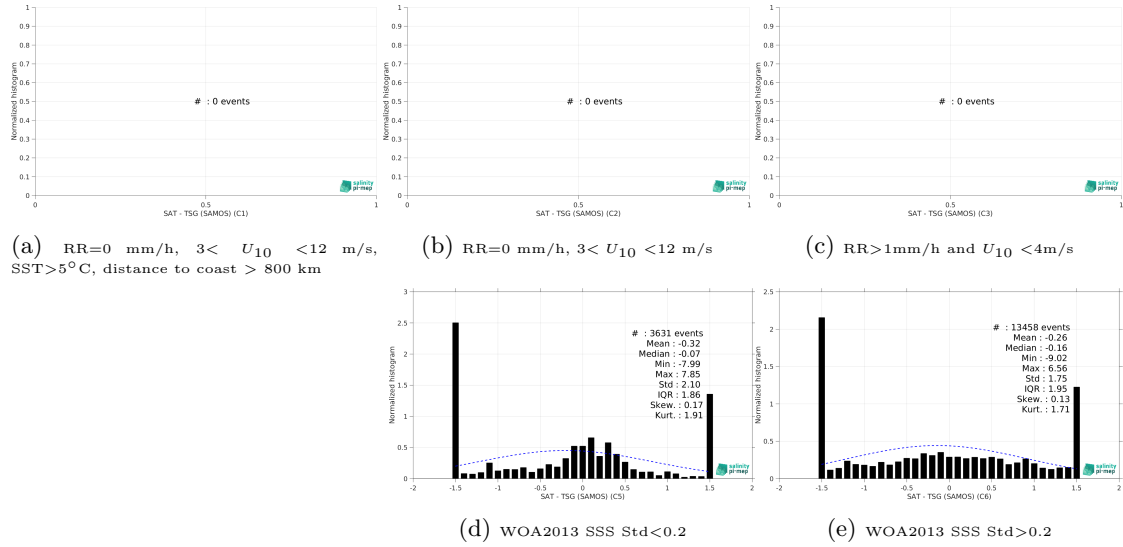
Figure 13: Normalized histogram of \Delta SSS (SMOS SSS L3 Arctic v2 - 18 Days (CATDS-CEC-LOCEAN) - TSG (SAMOS)) for 5 different subdatasets corresponding to: RR=0 mm/h, 3 < U_{10} < 12 m/s, SST > 5°C, distance to coast > 800 km (a), RR=0 mm/h, 3 < U_{10} < 12 m/s (b), RR > 1mm/h and U_{10} < 4 m/s (c), WOA2013 SSS Std < 0.2 (d), WOA2013 SSS Std > 0.2 (e).
