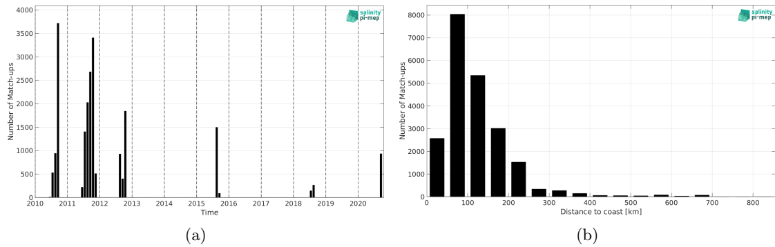
Figure 1: Number of match-ups between TSG (SAMOS) and SMOS SSS L3 Arctic v2 - 18 Days (CATDS-CEC-LOCEAN) SSS as a function of time (a) and as function of the distance to coast (b) over the Arctic Ocean Pi-MEP region and for the full satellite product period.
