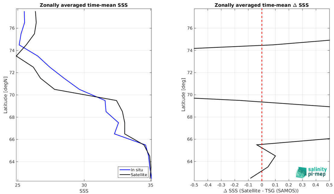
Figure 8: Left panel: Zonal mean SSS from SMOS SSS L3 Arctic v2 - 18 Days (CATDS-CEC-LOCEAN) satellite product (black) and from TSG (SAMOS) (blue). Right panel: Zonal mean of \Delta SSS (Satellite - TSG (SAMOS)) for all the collected Pi-MEP match-up pairs estimated over the full satellite product period.
