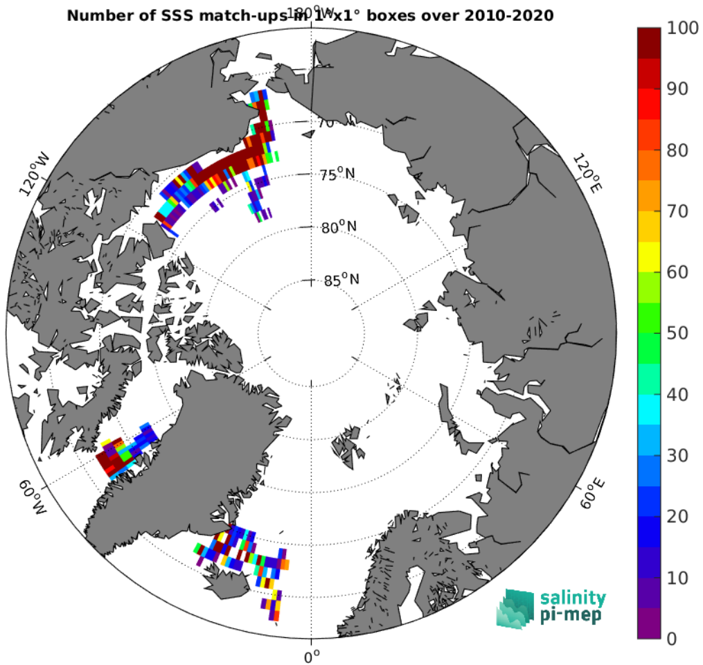
Figure 4: Number of SSS match-ups between TSG (SAMOS) SSS and the SMOS SSS L3 Arctic v2 - 18 Days (CATDS-CEC-LOCEAN) SSS product for the Arctic Ocean Pi-MEP region over 1^\circ \times 1^\circ boxes and for the full satellite product period.
