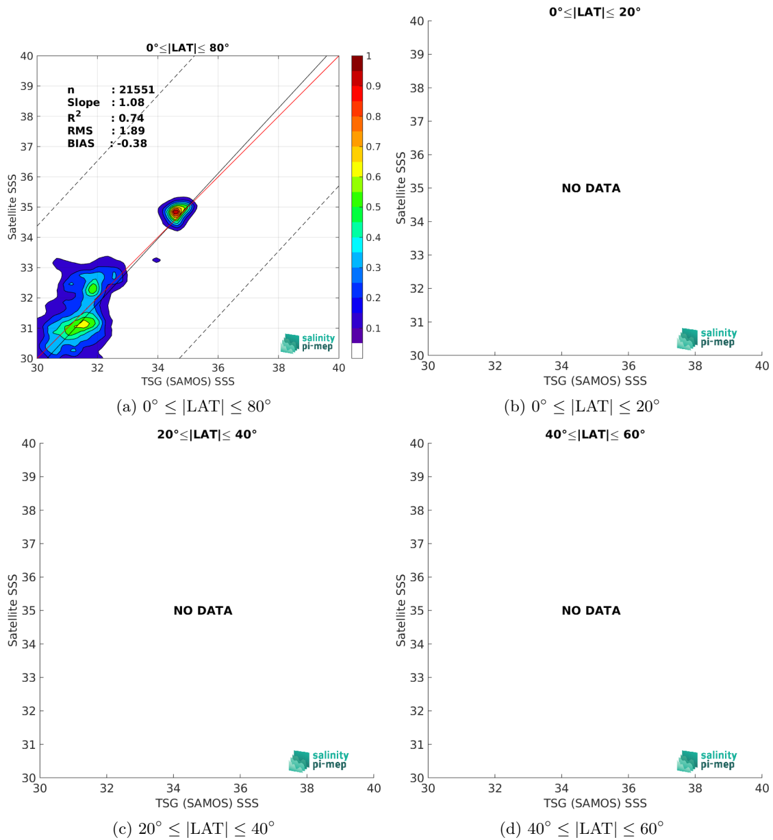
Figure 9: Contour maps of the concentration of SMOS SSS L3 Arctic v2 - 18 Days (CATDS-CEC-LOCEAN) SSS (y-axis) versus TSG (SAMOS) SSS (x-axis) at match-up pairs for different latitude bands. For each plot, the red line shows x=y . The black thin and dashed lines indicate a linear fit through the data cloud and the \pm 95\% confidence levels, respectively. The number match-up pairs n , the slope and R^2 coefficient of the linear fit, the root mean square (RMS) and the mean bias between satellite and in situ data are indicated for each latitude band in each plots.
