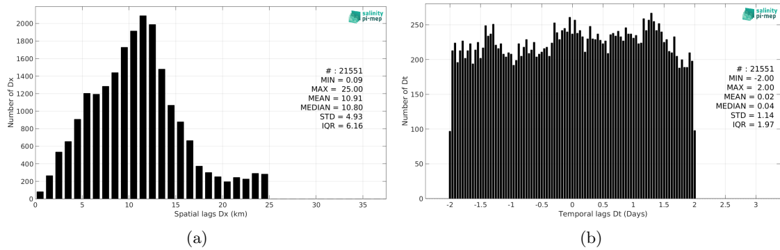
Figure 5: Histograms of the spatial (a) and temporal (b) lags between the location/time of the TSG (SAMOS) measurement and the date of the corresponding SMOS SSS L3 Arctic v2 - 18 Days (CATDS-CEC-LOCEAN) SSS pixel.
