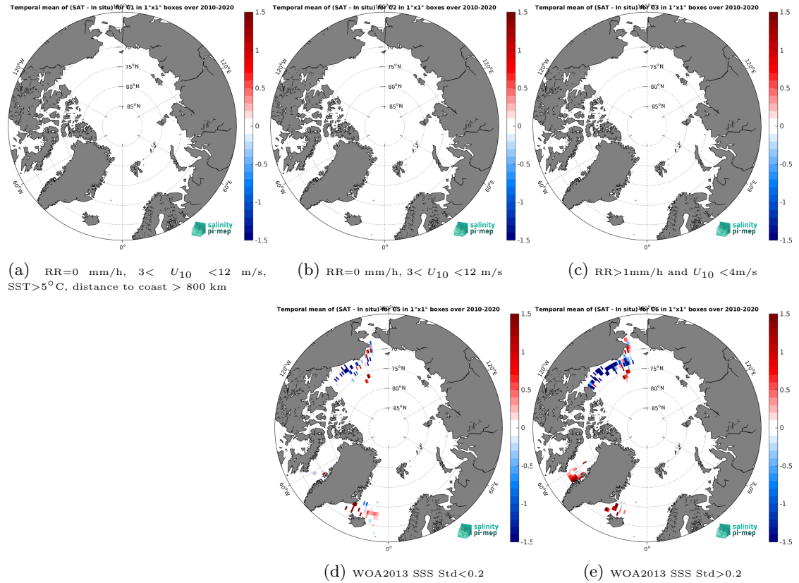
Figure 12: Temporal mean gridded over spatial boxes of size 1^{\circ}\times 1^{\circ} of \Delta\text{SSS} (SMOS SSS L3 Arctic v2 - 18 Days (CATDS-CEC-LOCEAN) - TSG (SAMOS)) for 5 different subdatasets corresponding to:RR=0 mm/h, 3 < U_{10} < 12 m/s, SST > 5^{\circ}\text{C} , distance to coast > 800 km (a), RR=0 mm/h, 3 < U_{10} < 12 m/s (b), RR > 1 mm/h and U_{10} < 4 m/s (c), WOA2013 SSS Std < 0.2 (d), WOA2013 SSS Std > 0.2 (e).
