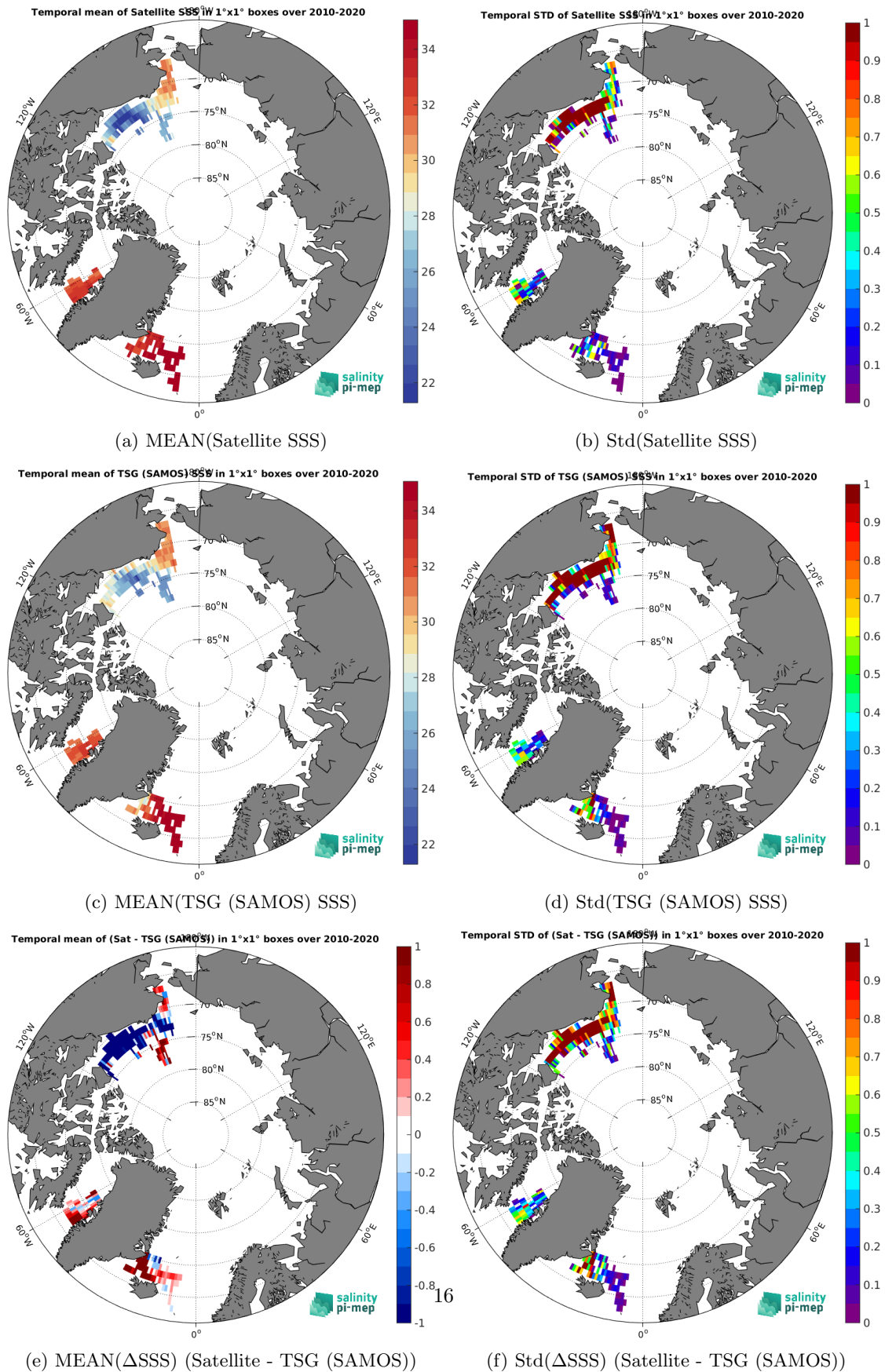
Figure 6: Temporal mean (left) and Std (right) of SSS from SMOS SSS L3 Arctic v2 - 18 Days (CATDS-CEC-LOCEAN) (top), TSG (SAMOS) (middle), and of \Delta SSS (Satellite - TSG (SAMOS)). Only match-up pairs are used to generate these maps.
