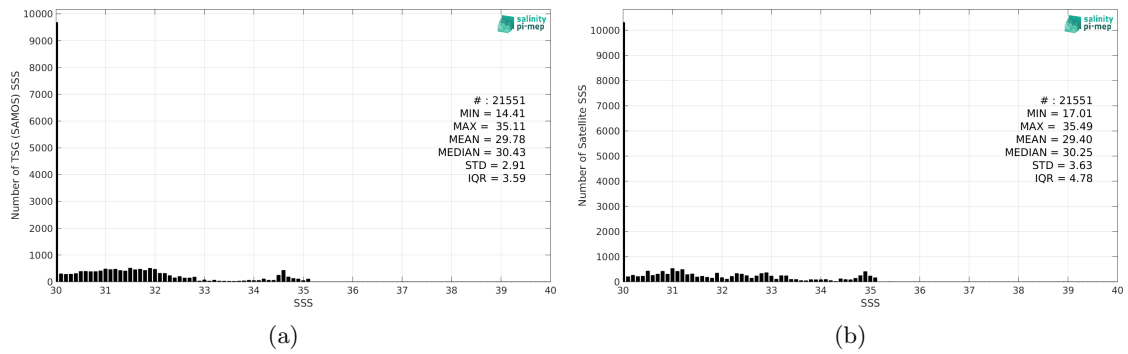
Figure 2: Histograms of SSS from TSG (SAMOS) (a) and SMOS SSS L3 Arctic v2 - 18 Days (CATDS-CEC-LOCEAN) (b) considering all match-up pairs per bins of 0.1 over the Arctic Ocean Pi-MEP region and for the full satellite product period.
