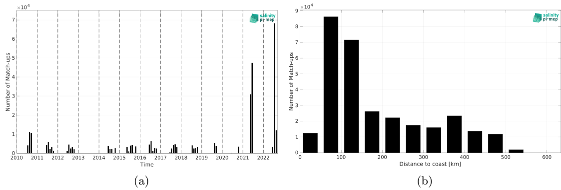
Figure 2: Number of match-ups between TSG (Polarstern) and SMOS SSS L3 Arctic v2 - 18 Days (CATDS-CEC-LOCEAN) SSS as a function of time (a) and as function of the distance to coast (b) over the Arctic Ocean Pi-MEP region and for the full satellite product period.
