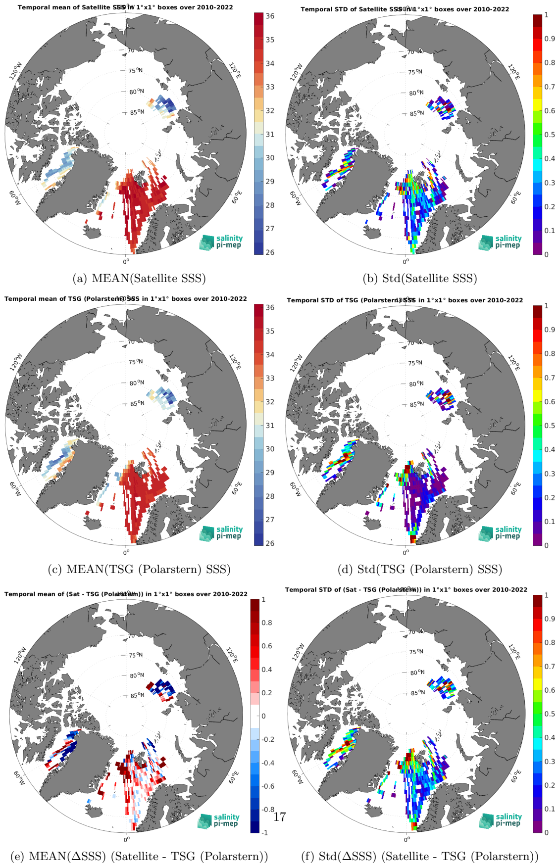
Figure 7: Temporal mean (left) and Std (right) of SSS from SMOS SSS L3 Arctic v2 - 18 Days (CATDS-CEC-LOCEAN) (top), TSG (Polarstern) (middle), and of \Delta SSS (Satellite - TSG (Polarstern)). Only match-up pairs are used to generate these maps.
