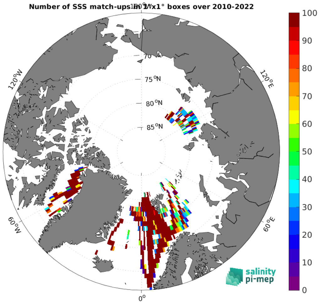
Figure 5: Number of SSS match-ups between TSG (Polarstern) SSS and the SMOS SSS L3 Arctic v2 - 18 Days (CATDS-CEC-LOCEAN) SSS product for the Arctic Ocean Pi-MEP region over 1^\circ \times 1^\circ boxes and for the full satellite product period.
