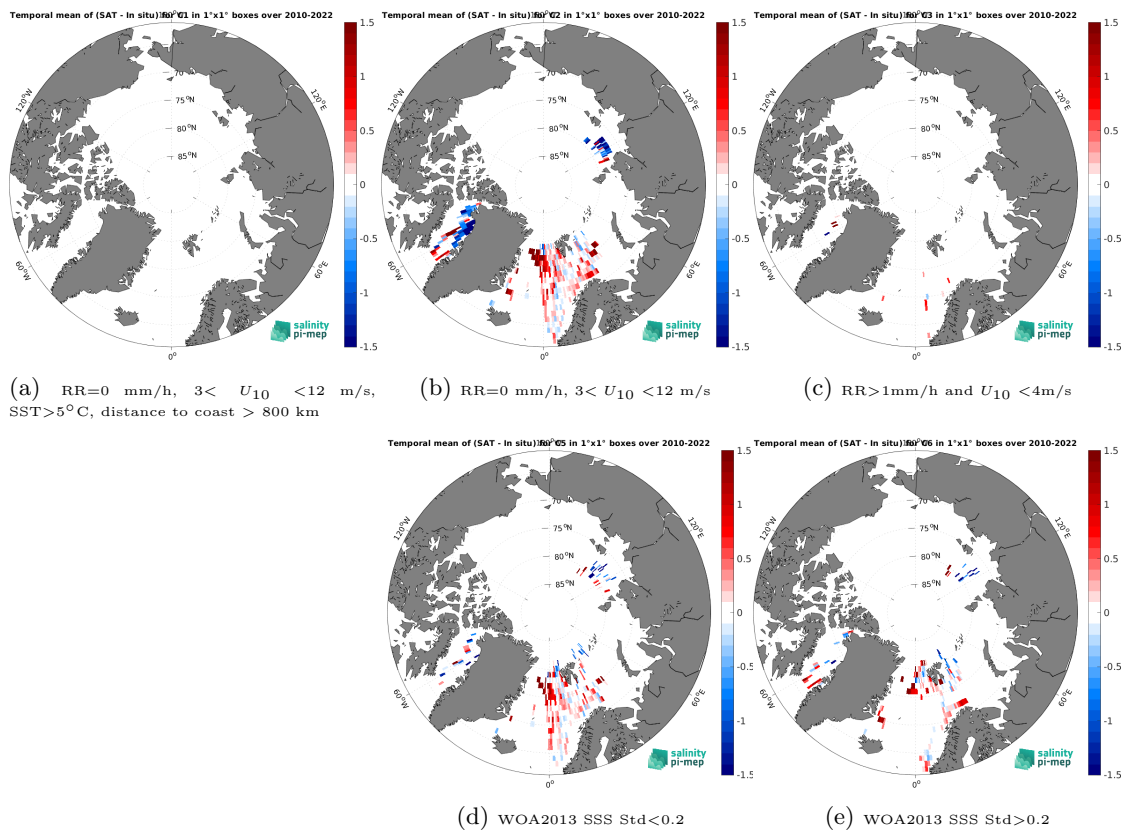
Figure 14: Temporal mean gridded over spatial boxes of size 1^\circ \times 1^\circ of \Delta\text{SSS} (SMOS SSS L3 Arctic v2 - 18 Days (CATDS-CEC-LOCEAN) - TSG (Polarstern)) for 5 different subdatasets corresponding to:RR=0 mm/h, 3 < U_{10} < 12 m/s, SST>5°C, distance to coast > 800 km (a), RR=0 mm/h, 3 < U_{10} < 12 m/s (b), RR>1mm/h and U_{10} < 4 m/s (c), WOA2013 SSS Std<0.2 (d), WOA2013 SSS Std>0.2 (e).
