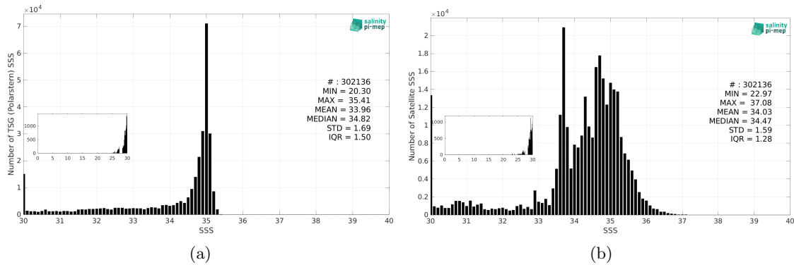
Figure 3: Histograms of SSS from TSG (Polarstern) (a) and SMOS SSS L3 Arctic v2 - 18 Days (CATDS-CEC-LOCEAN) (b) considering all match-up pairs per bins of 0.1 over the Arctic Ocean Pi-MEP region and for the full satellite product period.
