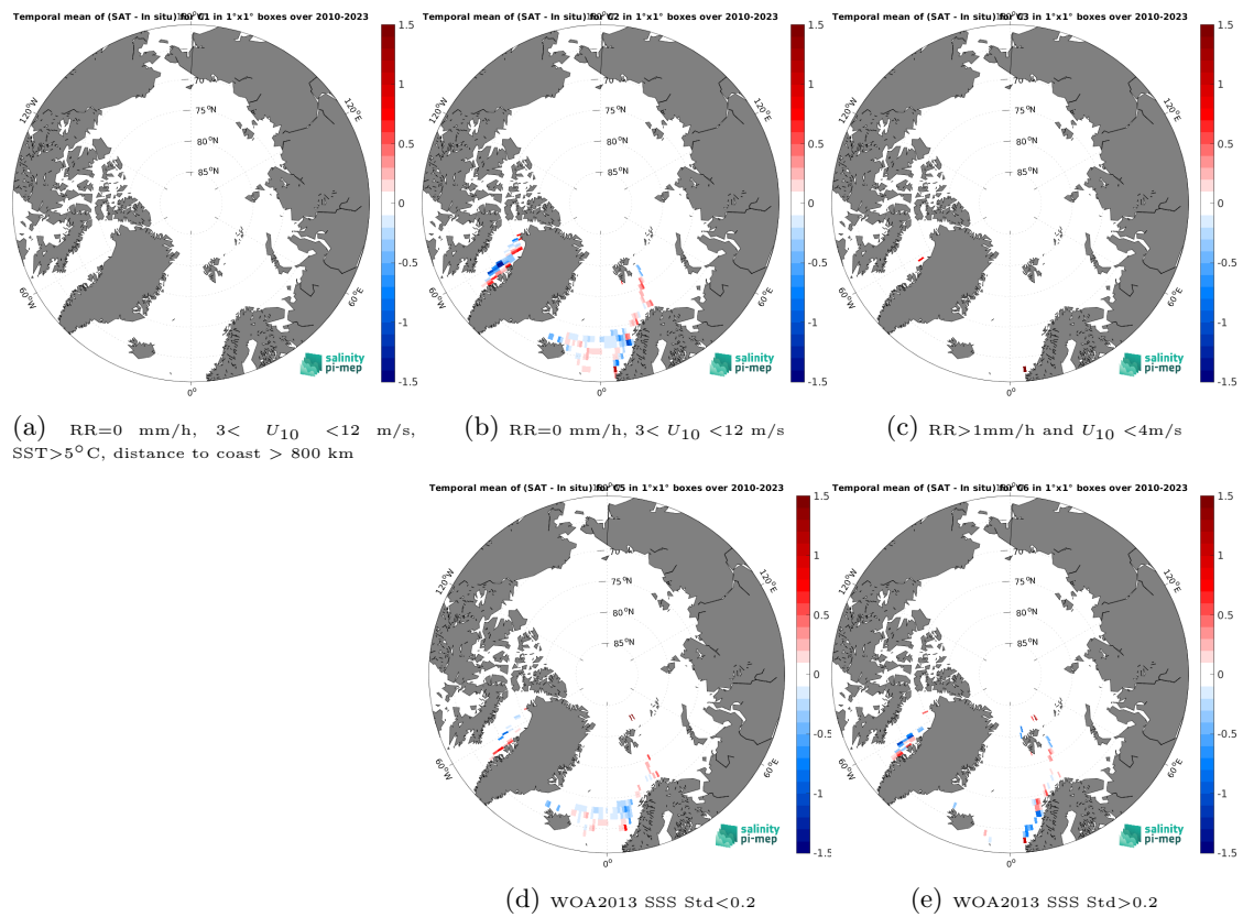
Figure 14: Temporal mean gridded over spatial boxes of size 1^\circ \times 1^\circ of \Delta SSS (SMOS SSS L3 Arctic v2 - 18 Days (CATDS-CEC-LOCEAN) - TSG (LEGOS-DM)) for 5 different subdatasets corresponding to: RR=0 mm/h, 3 < U_{10} < 12 m/s, SST >5^\circ\text{C} , distance to coast > 800 km (a), RR=0 mm/h, 3 < U_{10} < 12 m/s (b), RR >1 mm/h and U_{10} < 4 m/s (c), WOA2013 SSS Std <0.2 (d), WOA2013 SSS Std >0.2 (e).
