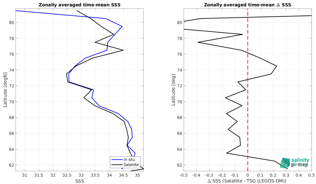
Figure 9: Left panel: Zonal mean SSS from SMOS SSS L3 Arctic v2 - 18 Days (CATDS-CEC-LOCEAN) satellite product (black) and from TSG (LEGOS-DM) (blue). Right panel: Zonal mean of \Delta SSS (Satellite - TSG (LEGOS-DM)) for all the collected Pi-MEP match-up pairs estimated over the full satellite product period.
