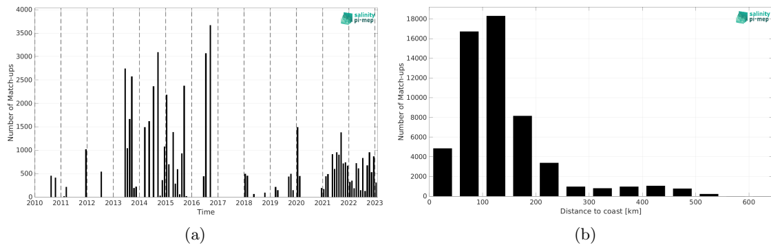
Figure 2: Number of match-ups between TSG (LEGOS-DM) and SMOS SSS L3 Arctic v2 - 18 Days (CATDS-CEC-LOCEAN) SSS as a function of time (a) and as function of the distance to coast (b) over the Arctic Ocean Pi-MEP region and for the full satellite product period.
