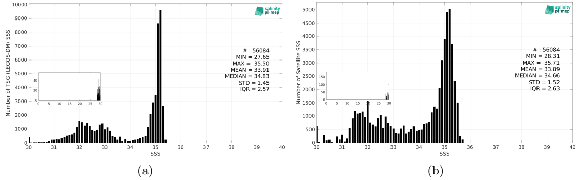
Figure 3: Histograms of SSS from TSG (LEGOS-DM) (a) and SMOS SSS L3 Arctic v2 - 18 Days (CATDS-CEC-LOCEAN) (b) considering all match-up pairs per bins of 0.1 over the Arctic Ocean Pi-MEP region and for the full satellite product period.
