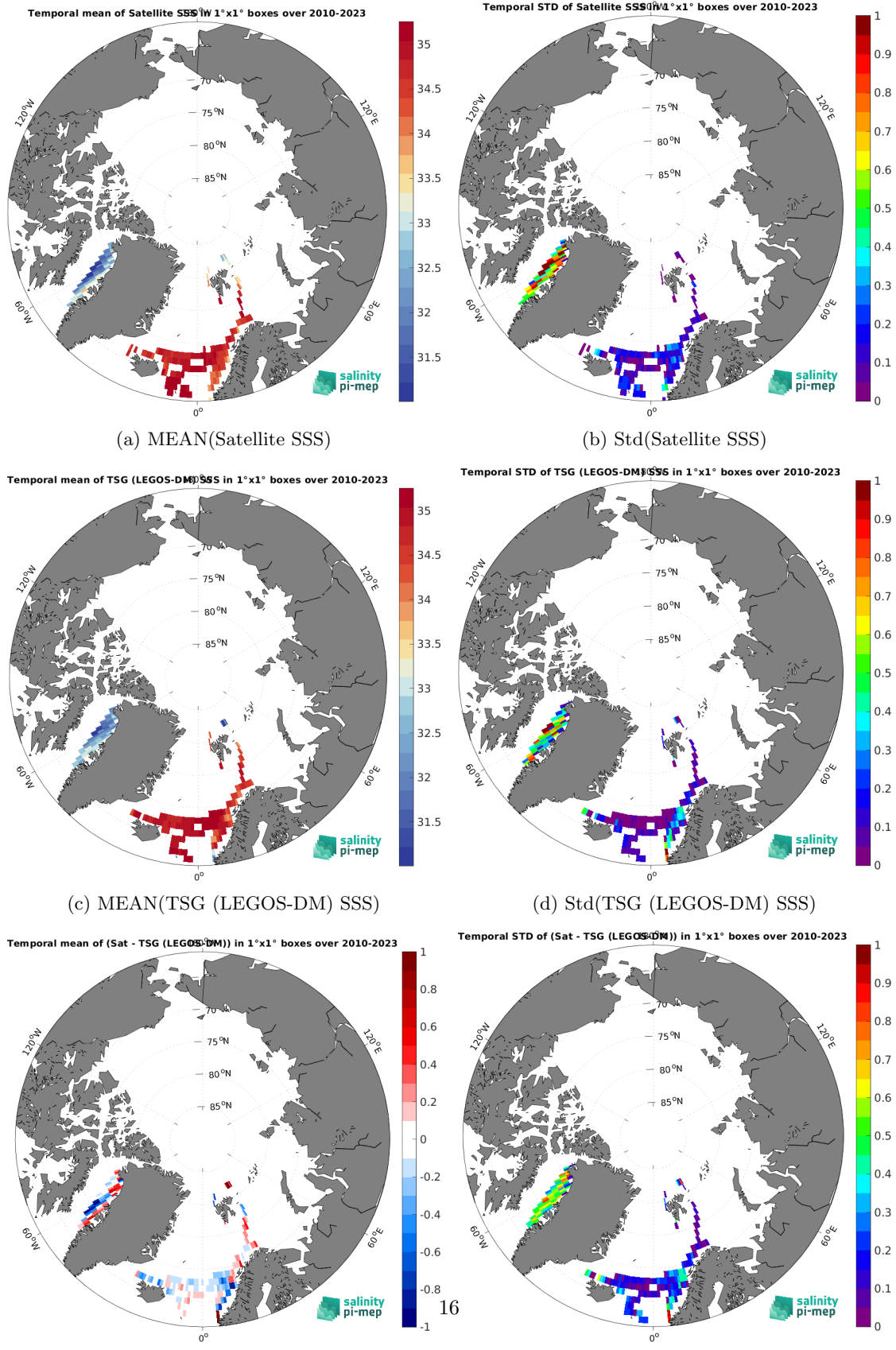
(e) MEAN( \Delta SSS) (Satellite - TSG (LEGOS-DM)) (f) Std( \Delta SSS) (Satellite - TSG (LEGOS-DM)) Figure 7: Temporal mean (left) and Std (right) of SSS from SMOS SSS L3 Arctic v2 - 18 Days (CATDS-CEC-LOCEAN) (top), TSG (LEGOS-DM) (middle), and of \Delta SSS (Satellite - TSG (LEGOS-DM)). Only match-up pairs are used to generate these maps.
