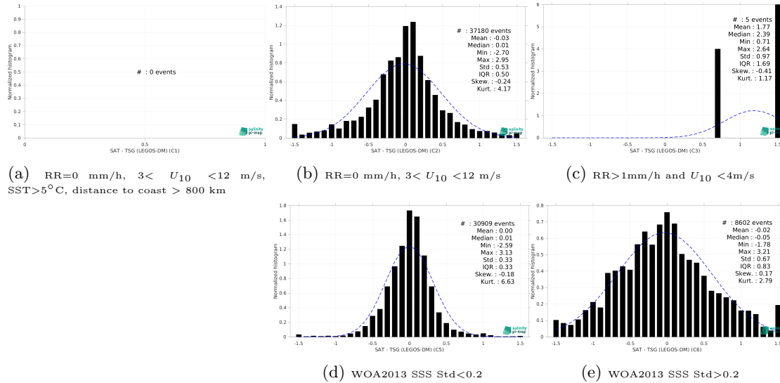
Figure 15: Normalized histogram of \Delta SSS (SMOS SSS L3 Arctic v2 - 18 Days (CATDS-CEC-LOCEAN) - TSG (LEGOS-DM)) for 5 different subdatasets corresponding to: RR=0 mm/h, 3 < U_{10} < 12 m/s, SST>5°C, distance to coast > 800 km (a), RR=0 mm/h, 3 < U_{10} < 12 m/s (b), RR>1mm/h and U_{10} < 4 m/s (c), WOA2013 SSS Std<0.2 (d), WOA2013 SSS Std>0.2 (e).
