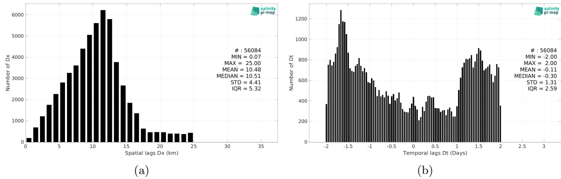
Figure 6: Histograms of the spatial (a) and temporal (b) lags between the location/time of the TSG (LEGOS-DM) measurement and the date of the corresponding SMOS SSS L3 Arctic v2 - 18 Days (CATDS-CEC-LOCEAN) SSS pixel.
