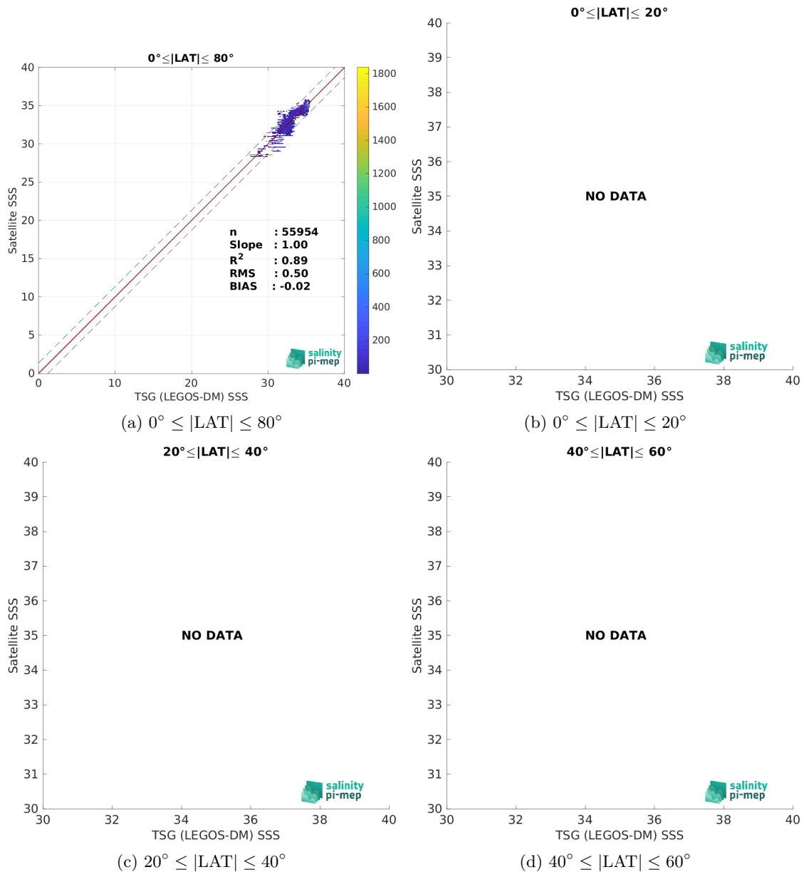
Figure 10: Contour maps of the concentration of SMOS SSS L3 Arctic v2 - 18 Days (CATDS-CEC-LOCEAN) SSS (y-axis) versus TSG (LEGOS-DM) SSS (x-axis) at match-up pairs for different latitude bands. For each plot, the red line shows x=y . The black thin and dashed lines indicate a linear fit through the data cloud and the \pm 95\% confidence levels, respectively. The number match-up pairs n , the slope and R^2 coefficient of the linear fit, the root mean square (RMS) and the mean bias between satellite and in situ data are indicated for each latitude band in each plots.
