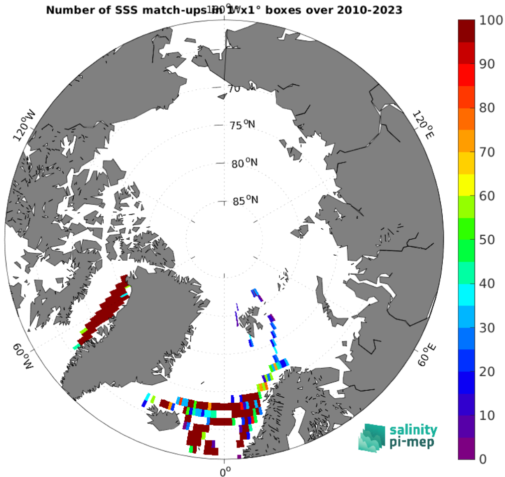
Figure 5: Number of SSS match-ups between TSG (LEGOS-DM) SSS and the SMOS SSS L3 Arctic v2 - 18 Days (CATDS-CEC-LOCEAN) SSS product for the Arctic Ocean Pi-MEP region over 1^\circ \times 1^\circ boxes and for the full satellite product period.
