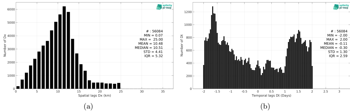
Figure 5: Histograms of the spatial (a) and temporal (b) lags between the location/time of the TSG (LEGOS-DM) measurement and the date of the corresponding SMOS SSS L3 Arctic v2 - 18 Days (CATDS-CEC-LOCEAN) SSS pixel.
