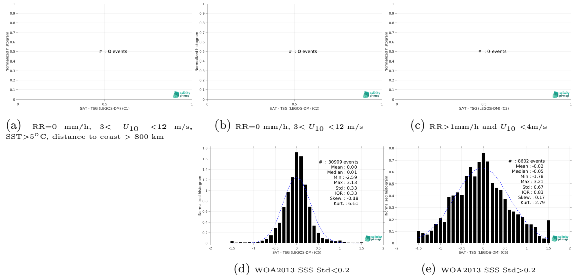
Figure 13: Normalized histogram of \Delta SSS (SMOS SSS L3 Arctic v2 - 18 Days (CATDS-CEC-LOCEAN) - TSG (LEGOS-DM)) for 5 different subdatasets corresponding to: RR=0 mm/h, 3 < U_{10} < 12 m/s, SST > 5°C, distance to coast > 800 km (a), RR=0 mm/h, 3 < U_{10} < 12 m/s (b), RR > 1mm/h and U_{10} < 4 m/s (c), WOA2013 SSS Std < 0.2 (d), WOA2013 SSS Std > 0.2 (e).
