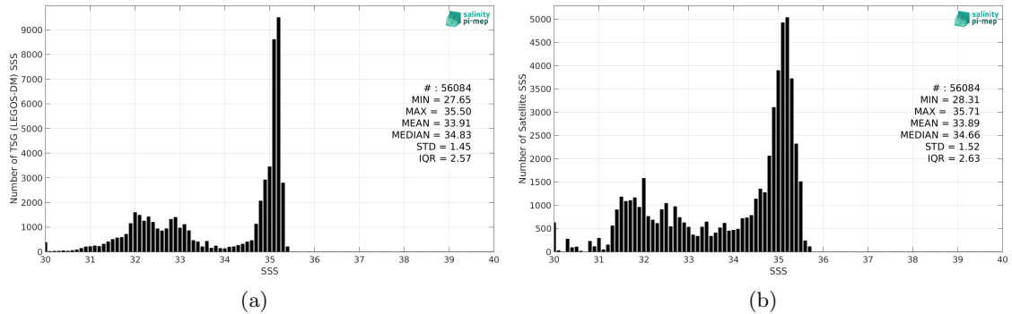
Figure 2: Histograms of SSS from TSG (LEGOS-DM) (a) and SMOS SSS L3 Arctic v2 - 18 Days (CATDS-CEC-LOCEAN) (b) considering all match-up pairs per bins of 0.1 over the Arctic Ocean Pi-MEP region and for the full satellite product period.
