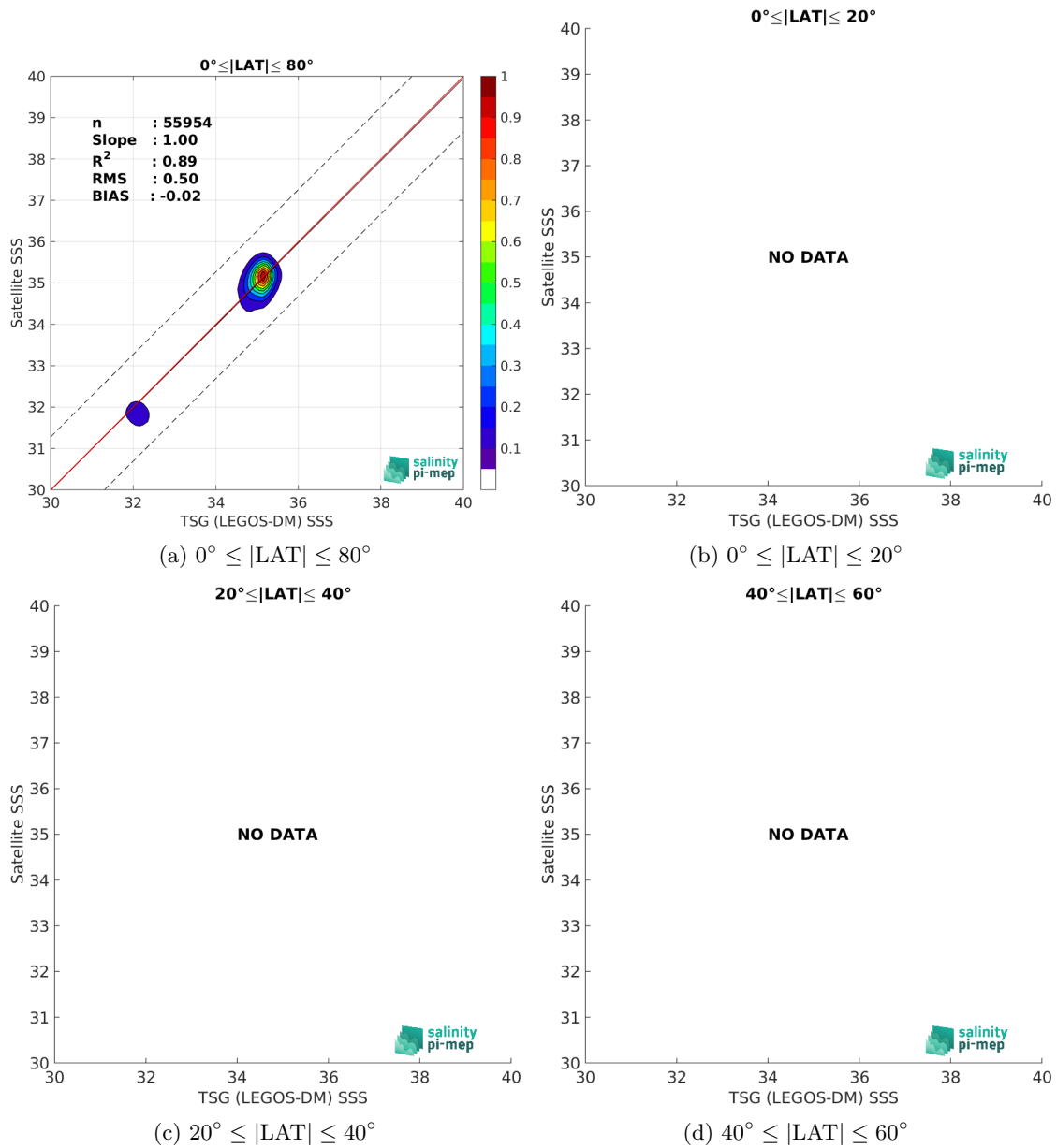
Figure 9: Contour maps of the concentration of SMOS SSS L3 Arctic v2 - 18 Days (CATDS-CEC-LOCEAN) SSS (y-axis) versus TSG (LEGOS-DM) SSS (x-axis) at match-up pairs for different latitude bands. For each plot, the red line shows x=y . The black thin and dashed lines indicate a linear fit through the data cloud and the \pm 95\% confidence levels, respectively. The number match-up pairs n , the slope and R^2 coefficient of the linear fit, the root mean square (RMS) and the mean bias between satellite and in situ data are indicated for each latitude band in each plots.
