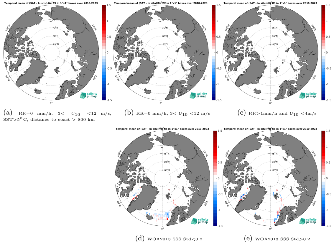
Figure 12: Temporal mean gridded over spatial boxes of size 1^{\circ}\times 1^{\circ} of \Delta\text{SSS} (SMOS SSS L3 Arctic v2 - 18 Days (CATDS-CEC-LOCEAN) - TSG (LEGOS-DM)) for 5 different subdatasets corresponding to:RR=0 mm/h, 3 < U_{10} < 12 m/s, SST > 5^{\circ}\text{C} , distance to coast > 800 km (a), RR=0 mm/h, 3 < U_{10} < 12 m/s (b), RR > 1 mm/h and U_{10} < 4 m/s (c), WOA2013 SSS Std < 0.2 (d), WOA2013 SSS Std > 0.2 (e).
