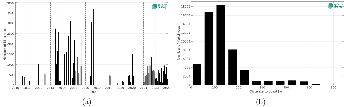
Figure 1: Number of match-ups between TSG (LEGOS-DM) and SMOS SSS L3 Arctic v2 - 18 Days (CATDS-CEC-LOCEAN) SSS as a function of time (a) and as function of the distance to coast (b) over the Arctic Ocean Pi-MEP region and for the full satellite product period.
