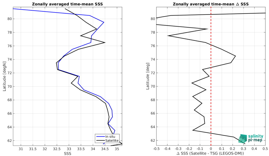
Figure 8: Left panel: Zonal mean SSS from SMOS SSS L3 Arctic v2 - 18 Days (CATDS-CEC-LOCEAN) satellite product (black) and from TSG (LEGOS-DM) (blue). Right panel: Zonal mean of \Delta SSS (Satellite - TSG (LEGOS-DM)) for all the collected Pi-MEP match-up pairs estimated over the full satellite product period.
