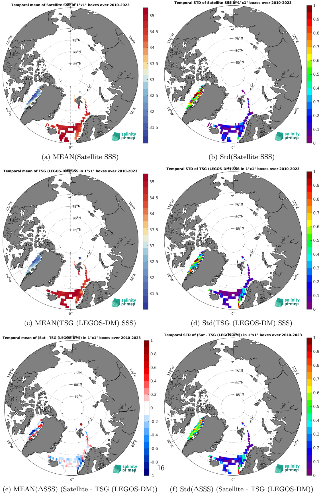
Figure 6: Temporal mean (left) and Std (right) of SSS from SMOS SSS L3 Arctic v2 - 18 Days (CATDS-CEC-LOCEAN) (top), TSG (LEGOS-DM) (middle), and of \Delta SSS (Satellite - TSG (LEGOS-DM)). Only match-up pairs are used to generate these maps.
