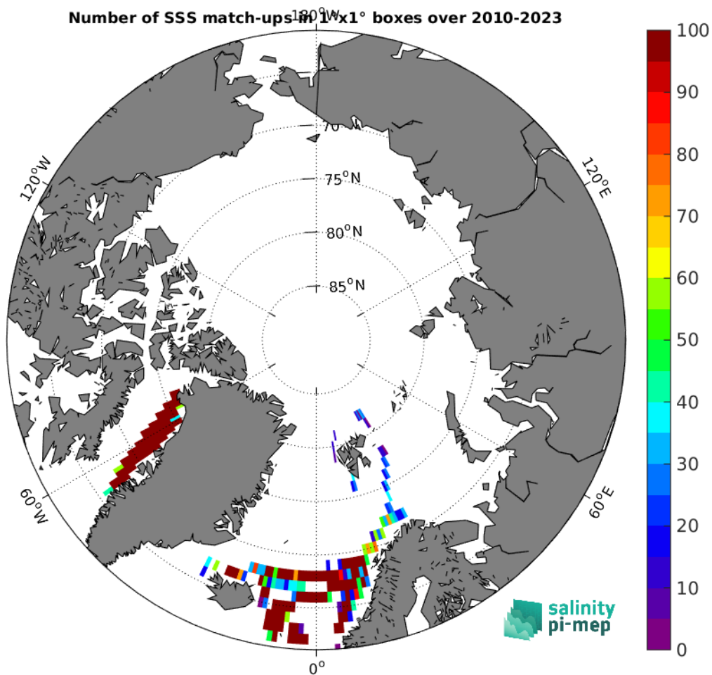
Figure 4: Number of SSS match-ups between TSG (LEGOS-DM) SSS and the SMOS SSS L3 Arctic v2 - 18 Days (CATDS-CEC-LOCEAN) SSS product for the Arctic Ocean Pi-MEP region over 1^\circ \times 1^\circ boxes and for the full satellite product period.
