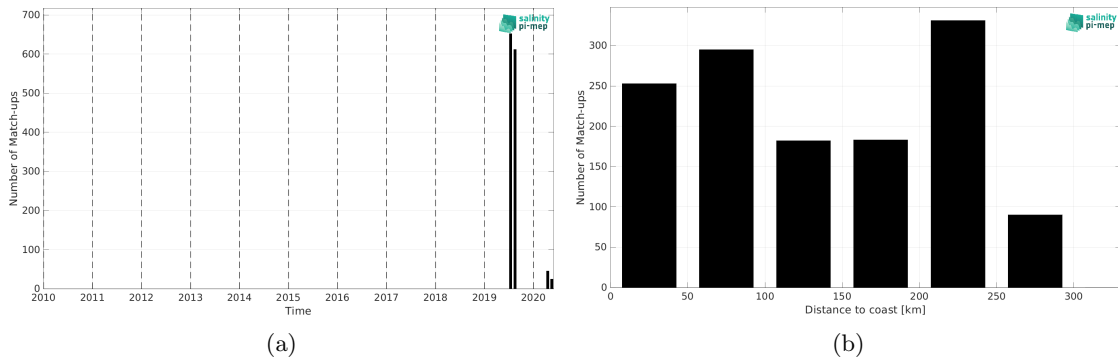
Figure 2: Number of match-ups between TSG (Lauge-Koch) and SMOS SSS L3 Arctic v2 - 18 Days (CATDS-CEC-LOCEAN) SSS as a function of time (a) and as function of the distance to coast (b) over the Arctic Ocean Pi-MEP region and for the full satellite product period.
