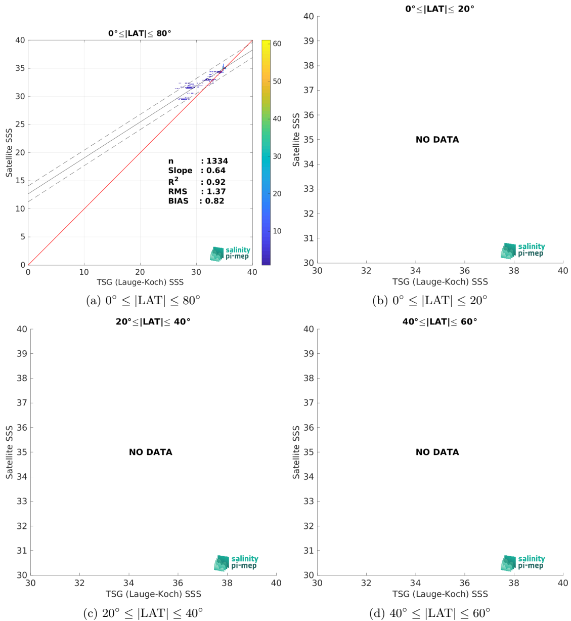
Figure 10: Contour maps of the concentration of SMOS SSS L3 Arctic v2 - 18 Days (CATDS-CEC-LOCEAN) SSS (y-axis) versus TSG (Lauge-Koch) SSS (x-axis) at match-up pairs for different latitude bands. For each plot, the red line shows x=y . The black thin and dashed lines indicate a linear fit through the data cloud and the \pm 95\% confidence levels, respectively. The number match-up pairs n , the slope and R^2 coefficient of the linear fit, the root mean square (RMS) and the mean bias between satellite and in situ data are indicated for each latitude band in each plots.
