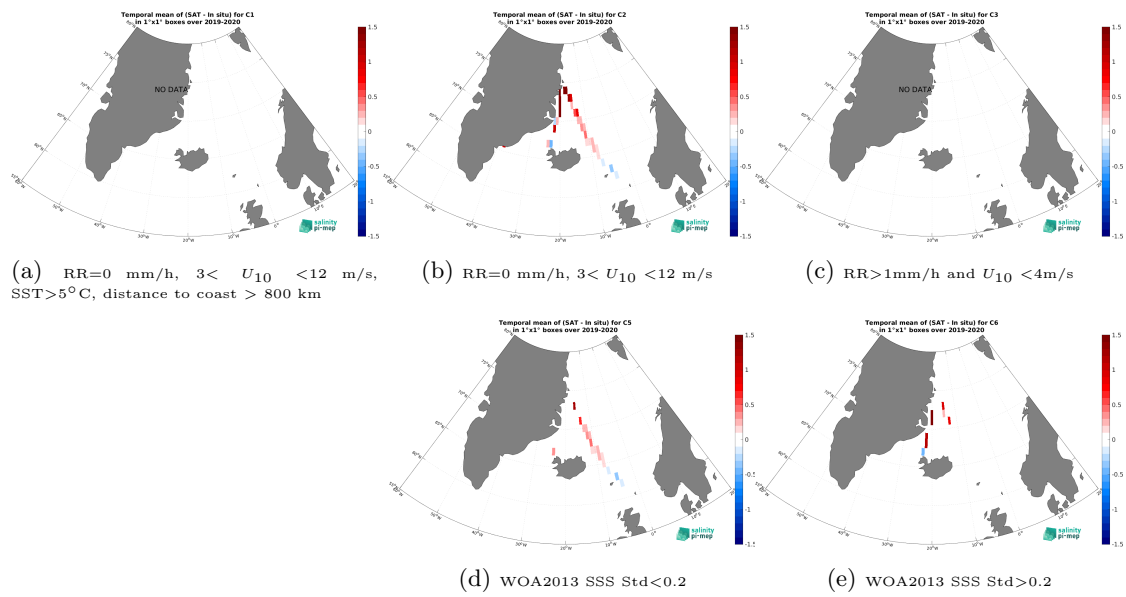
Figure 14: Temporal mean gridded over spatial boxes of size 1^\circ \times 1^\circ of \Delta SSS (SMOS SSS L3 Arctic v2 - 18 Days (CATDS-CEC-LOCEAN) - TSG (Lauge-Koch)) for 5 different subdatasets corresponding to: RR=0 mm/h, 3 < U_{10} < 12 m/s, SST > 5^\circ\text{C} , distance to coast > 800 km (a), RR=0 mm/h, 3 < U_{10} < 12 m/s (b), RR > 1 mm/h and U_{10} < 4 m/s (c), WOA2013 SSS Std < 0.2 (d), WOA2013 SSS Std > 0.2 (e).
