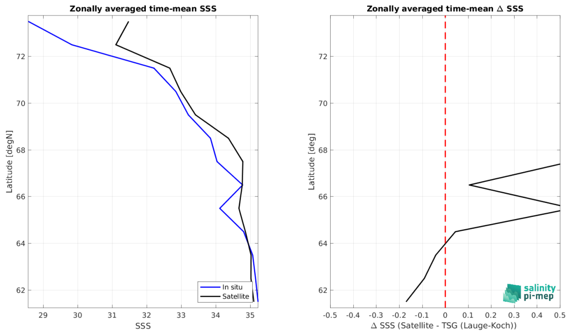
Figure 9: Left panel: Zonal mean SSS from SMOS SSS L3 Arctic v2 - 18 Days (CATDS-CEC-LOCEAN) satellite product (black) and from TSG (Lauge-Koch) (blue). Right panel: Zonal mean of \Delta SSS (Satellite - TSG (Lauge-Koch)) for all the collected Pi-MEP match-up pairs estimated over the full satellite product period.
