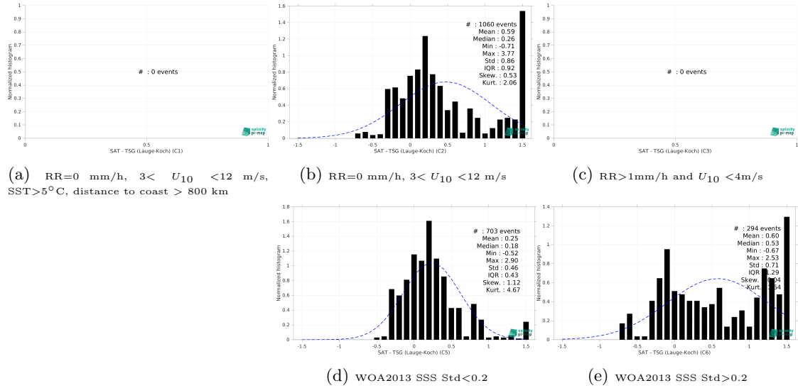
Figure 15: Normalized histogram of \Delta SSS (SMOS SSS L3 Arctic v2 - 18 Days (CATDS-CEC-LOCEAN) - TSG (Lauge-Koch)) for 5 different subdatasets corresponding to: RR=0 mm/h, 3 < U_{10} < 12 m/s, SST > 5°C, distance to coast > 800 km (a), RR=0 mm/h, 3 < U_{10} < 12 m/s (b), RR > 1mm/h and U_{10} < 4 m/s (c), WOA2013 SSS Std < 0.2 (d), WOA2013 SSS Std > 0.2 (e).
