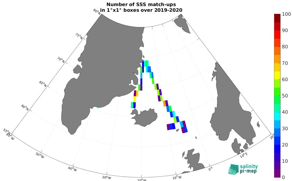
Figure 5: Number of SSS match-ups between TSG (Lauge-Koch) SSS and the SMOS SSS L3 Arctic v2 - 18 Days (CATDS-CEC-LOCEAN) SSS product for the Arctic Ocean Pi-MEP region over 1^\circ \times 1^\circ boxes and for the full satellite product period.
