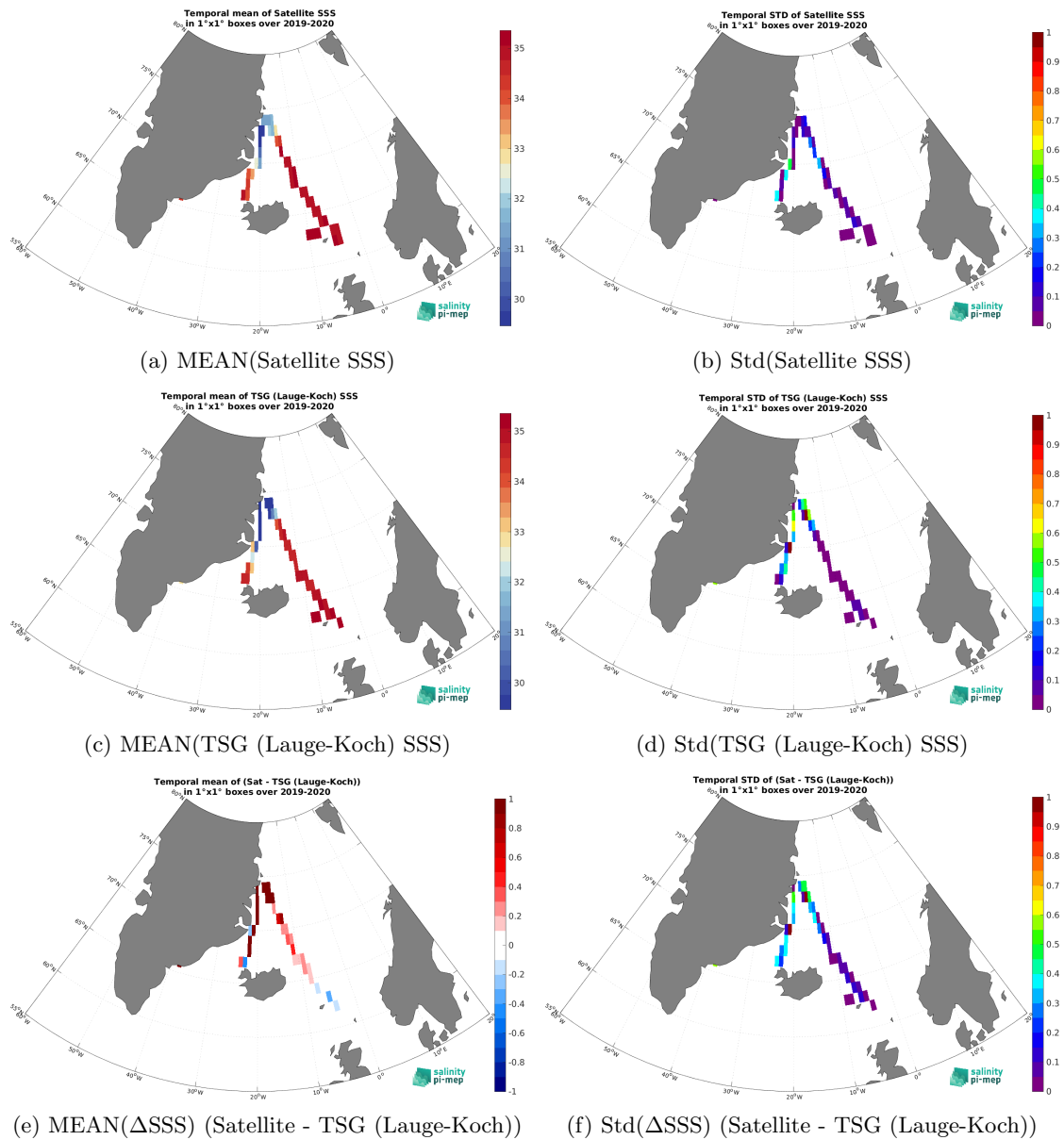
Figure 7: Temporal mean (left) and Std (right) of SSS from SMOS SSS L3 Arctic v2 - 18 Days (CATDS-CEC-LOCEAN) (top), TSG (Lauge-Koch) (middle), and of \Delta SSS (Satellite - TSG (Lauge-Koch)). Only match-up pairs are used to generate these maps.
