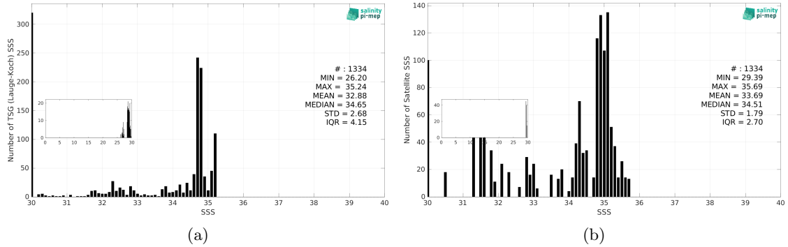
Figure 3: Histograms of SSS from TSG (Lauge-Koch) (a) and SMOS SSS L3 Arctic v2 - 18 Days (CATDS-CEC-LOCEAN) (b) considering all match-up pairs per bins of 0.1 over the Arctic Ocean Pi-MEP region and for the full satellite product period.
