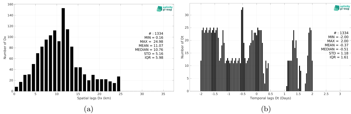
Figure 6: Histograms of the spatial (a) and temporal (b) lags between the location/time of the TSG (Lauge-Koch) measurement and the date of the corresponding SMOS SSS L3 Arctic v2 - 18 Days (CATDS-CEC-LOCEAN) SSS pixel.
