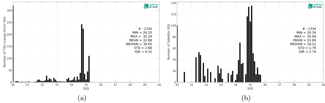
Figure 2: Histograms of SSS from TSG (Lauge-Koch) (a) and SMOS SSS L3 Arctic v2 - 18 Days (CATDS-CEC-LOCEAN) (b) considering all match-up pairs per bins of 0.1 over the Arctic Ocean Pi-MEP region and for the full satellite product period.
