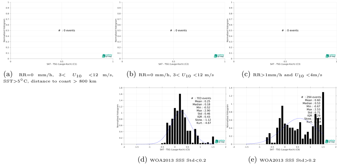
Figure 13: Normalized histogram of \Delta SSS (SMOS SSS L3 Arctic v2 - 18 Days (CATDS-CEC-LOCEAN) - TSG (Lauge-Koch)) for 5 different subdatasets corresponding to: RR=0 mm/h, 3 < U_{10} < 12 m/s, SST > 5°C, distance to coast > 800 km (a), RR=0 mm/h, 3 < U_{10} < 12 m/s (b), RR > 1mm/h and U_{10} < 4 m/s (c), WOA2013 SSS Std < 0.2 (d), WOA2013 SSS Std > 0.2 (e).
