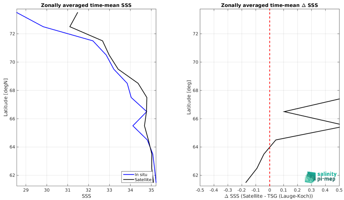
Figure 8: Left panel: Zonal mean SSS from SMOS SSS L3 Arctic v2 - 18 Days (CATDS-CEC-LOCEAN) satellite product (black) and from TSG (Lauge-Koch) (blue). Right panel: Zonal mean of \Delta SSS (Satellite - TSG (Lauge-Koch)) for all the collected Pi-MEP match-up pairs estimated over the full satellite product period.
