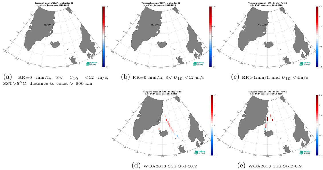
Figure 12: Temporal mean gridded over spatial boxes of size 1^{\circ}\times 1^{\circ} of \Delta\text{SSS} (SMOS SSS L3 Arctic v2 - 18 Days (CATDS-CEC-LOCEAN) - TSG (Lauge-Koch)) for 5 different subdatasets corresponding to:RR=0 mm/h, 3 < U_{10} < 12 m/s, SST >5^{\circ}\text{C} , distance to coast > 800 km (a), RR=0 mm/h, 3 < U_{10} < 12 m/s (b), RR >1 mm/h and U_{10} < 4 m/s (c), WOA2013 SSS Std <0.2 (d), WOA2013 SSS Std >0.2 (e).
