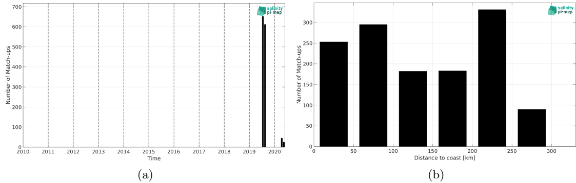
Figure 1: Number of match-ups between TSG (Lauge-Koch) and SMOS SSS L3 Arctic v2 - 18 Days (CATDS-CEC-LOCEAN) SSS as a function of time (a) and as function of the distance to coast (b) over the Arctic Ocean Pi-MEP region and for the full satellite product period.
