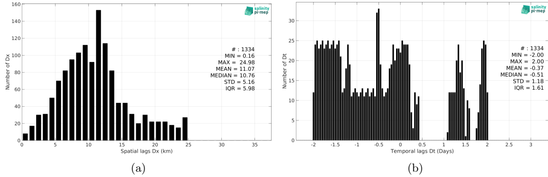
Figure 5: Histograms of the spatial (a) and temporal (b) lags between the location/time of the TSG (Lauge-Koch) measurement and the date of the corresponding SMOS SSS L3 Arctic v2 - 18 Days (CATDS-CEC-LOCEAN) SSS pixel.
