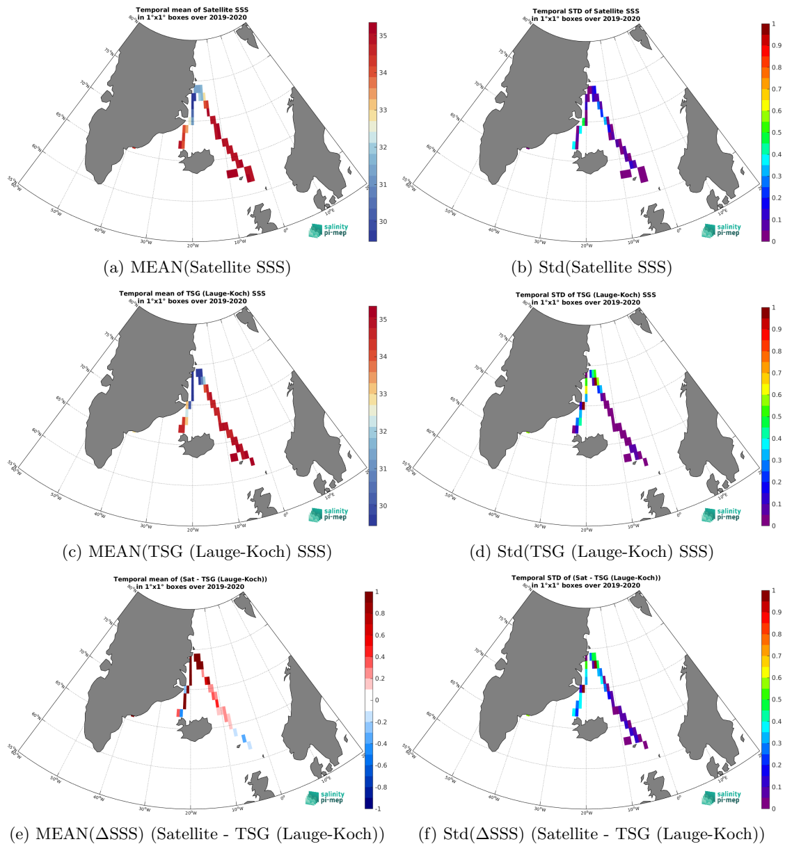
Figure 6: Temporal mean (left) and Std (right) of SSS from SMOS SSS L3 Arctic v2 - 18 Days (CATDS-CEC-LOCEAN) (top), TSG (Lauge-Koch) (middle), and of \Delta SSS (Satellite - TSG (Lauge-Koch)). Only match-up pairs are used to generate these maps.
