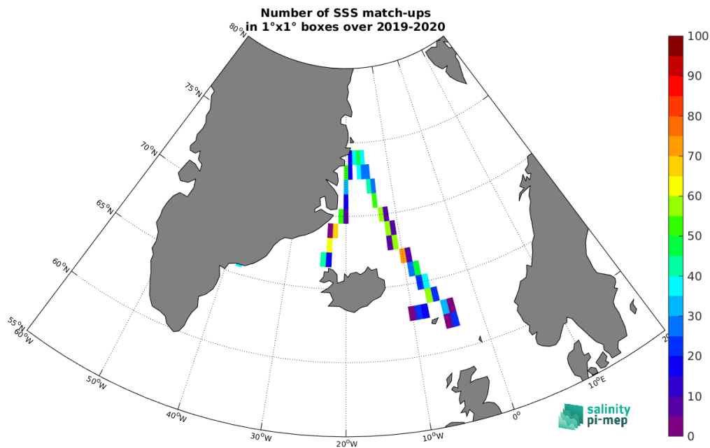
Figure 4: Number of SSS match-ups between TSG (Lauge-Koch) SSS and the SMOS SSS L3 Arctic v2 - 18 Days (CATDS-CEC-LOCEAN) SSS product for the Arctic Ocean Pi-MEP region over 1^\circ \times 1^\circ boxes and for the full satellite product period.
