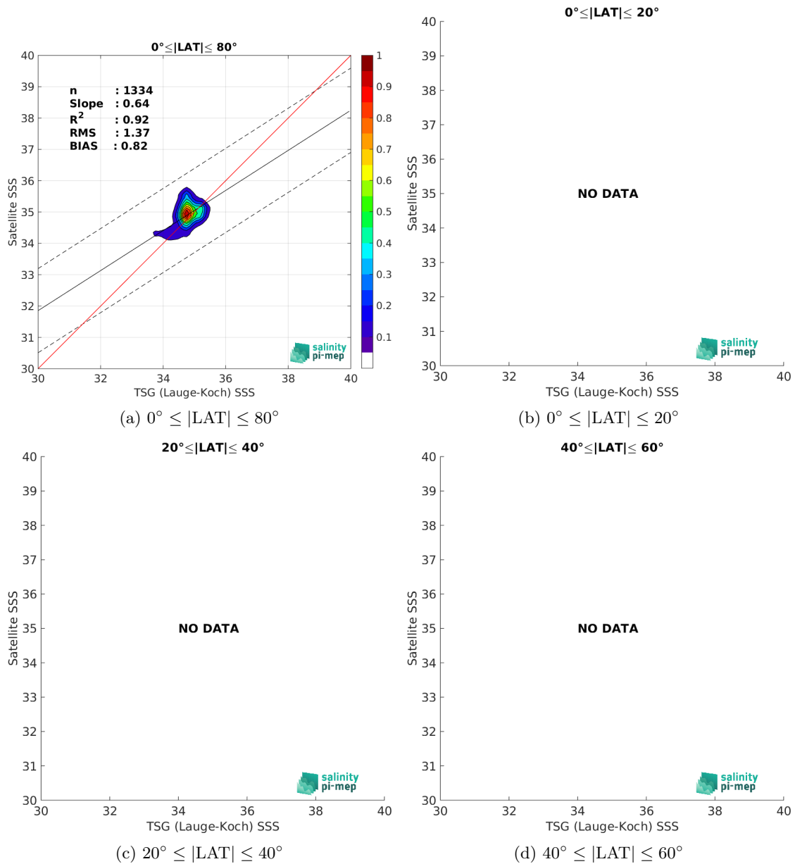
Figure 9: Contour maps of the concentration of SMOS SSS L3 Arctic v2 - 18 Days (CATDS-CEC-LOCEAN) SSS (y-axis) versus TSG (Lauge-Koch) SSS (x-axis) at match-up pairs for different latitude bands. For each plot, the red line shows x=y . The black thin and dashed lines indicate a linear fit through the data cloud and the \pm 95\% confidence levels, respectively. The number match-up pairs n , the slope and R^2 coefficient of the linear fit, the root mean square (RMS) and the mean bias between satellite and in situ data are indicated for each latitude band in each plots.
