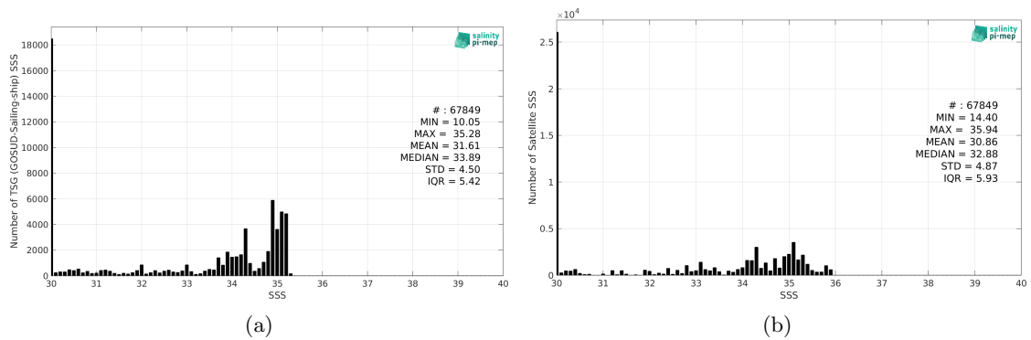
Figure 2: Histograms of SSS from TSG (GOSUD-Sailing-ship) (a) and SMOS SSS L3 Arctic v2 - 18 Days (CATDS-CEC-LOCEAN) (b) considering all match-up pairs per bins of 0.1 over the Arctic Ocean Pi-MEP region and for the full satellite product period.
