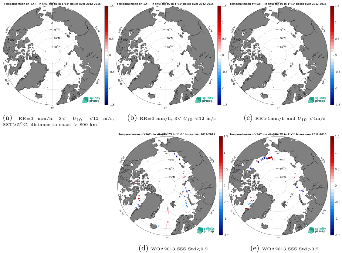
Figure 12: Temporal mean gridded over spatial boxes of size 1^\circ \times 1^\circ of \Delta SSS (SMOS SSS L3 Arctic v2 - 18 Days (CATDS-CEC-LOCEAN) - TSG (GOSUD-Sailing-ship)) for 5 different subdatasets corresponding to:RR=0 mm/h, 3 < U_{10} < 12 m/s, SST>5°C, distance to coast > 800 km (a), RR=0 mm/h, 3 < U_{10} < 12 m/s (b), RR>1mm/h and U_{10} < 4 m/s (c), WOA2013 SSS Std<0.2 (d), WOA2013 SSS Std>0.2 (e).
