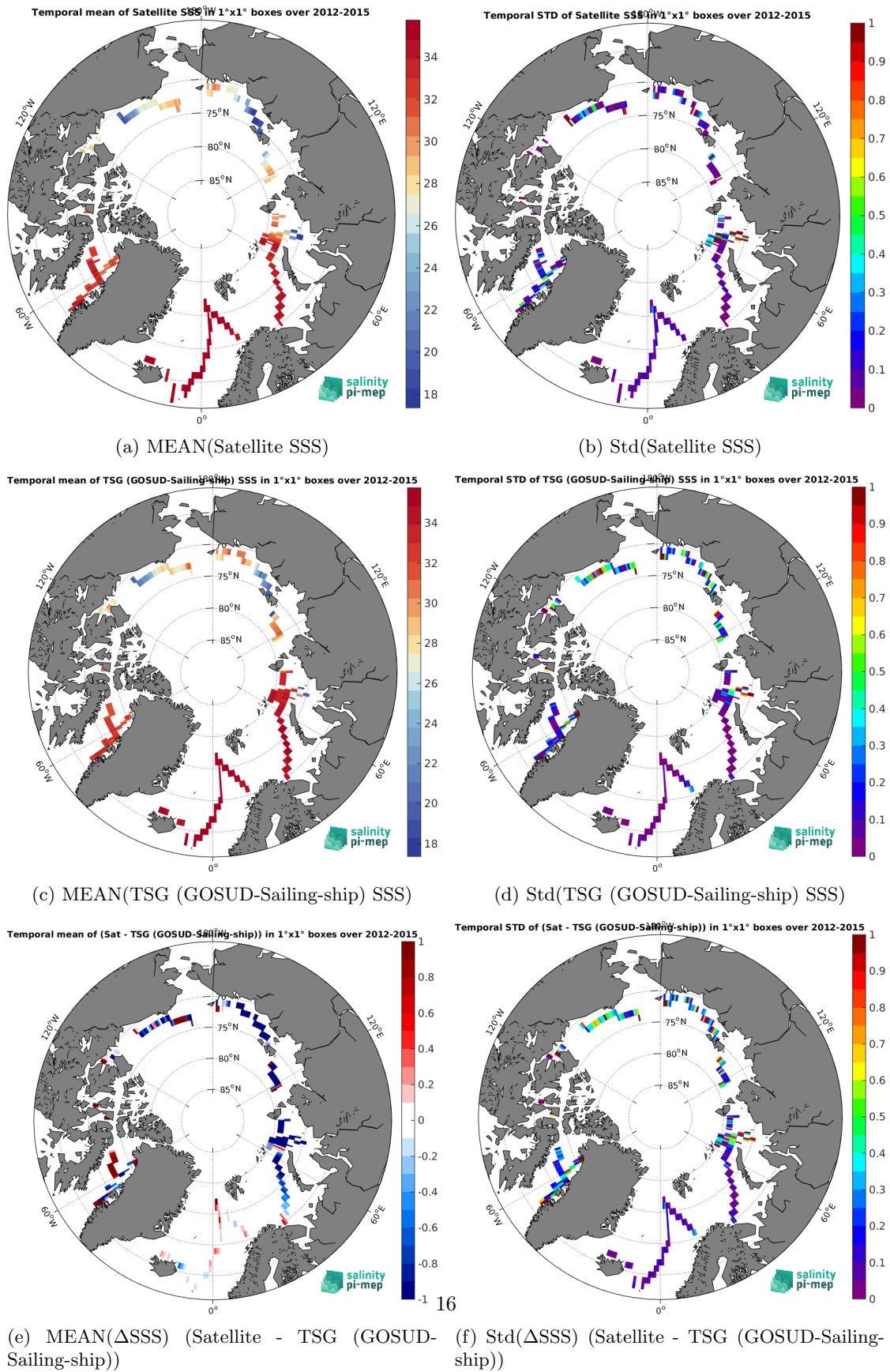
Figure 6: Temporal mean (left) and Std (right) of SSS from SMOS SSS L3 Arctic v2 - 18 Days (CATDS-CEC-LOCEAN) (top), TSG (GOSUD-Sailing-ship) (middle), and of \Delta SSS (Satellite - TSG (GOSUD-Sailing-ship)). Only match-up pairs are used to generate these maps.
