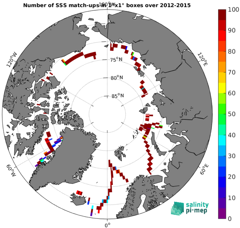
Figure 4: Number of SSS match-ups between TSG (GOSUD-Sailing-ship) SSS and the SMOS SSS L3 Arctic v2 - 18 Days (CATDS-CEC-LOCEAN) SSS product for the Arctic Ocean Pi-MEP region over 1^\circ \times 1^\circ boxes and for the full satellite product period.
