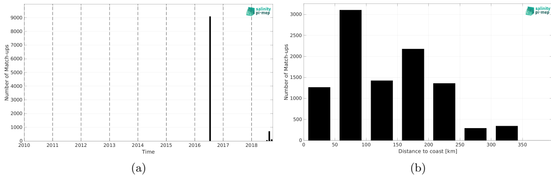
Figure 2: Number of match-ups between TSG (GOSUD-Research-vessel) and SMOS SSS L3 Arctic v2 - 18 Days (CATDS-CEC-LOCEAN) SSS as a function of time (a) and as function of the distance to coast (b) over the Arctic Ocean Pi-MEP region and for the full satellite product period.
