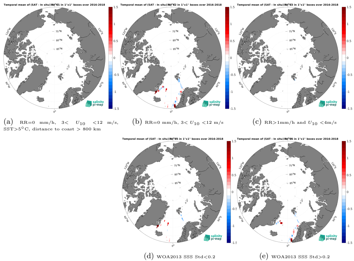
Figure 14: Temporal mean gridded over spatial boxes of size 1^\circ \times 1^\circ of \Delta\text{SSS} (SMOS SSS L3 Arctic v2 - 18 Days (CATDS-CEC-LOCEAN) - TSG (GOSUD-Research-vessel)) for 5 different subdatasets corresponding to:RR=0 mm/h, 3 < U_{10} < 12 m/s, SST>5°C, distance to coast > 800 km (a), RR=0 mm/h, 3 < U_{10} < 12 m/s (b), RR>1mm/h and U_{10} < 4 m/s (c), WOA2013 SSS Std<0.2 (d), WOA2013 SSS Std>0.2 (e).
