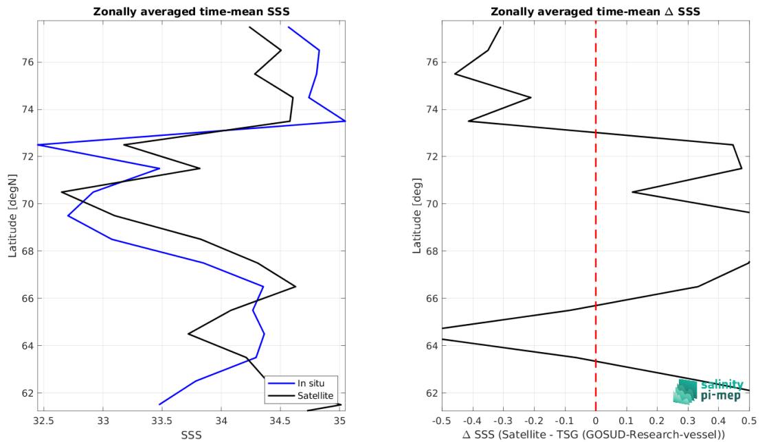
Figure 9: Left panel: Zonal mean SSS from SMOS SSS L3 Arctic v2 - 18 Days (CATDS-CEC-LOCEAN) satellite product (black) and from TSG (GOSUD-Research-vessel) (blue). Right panel: Zonal mean of \Delta SSS (Satellite - TSG (GOSUD-Research-vessel)) for all the collected Pi-MEP match-up pairs estimated over the full satellite product period.
