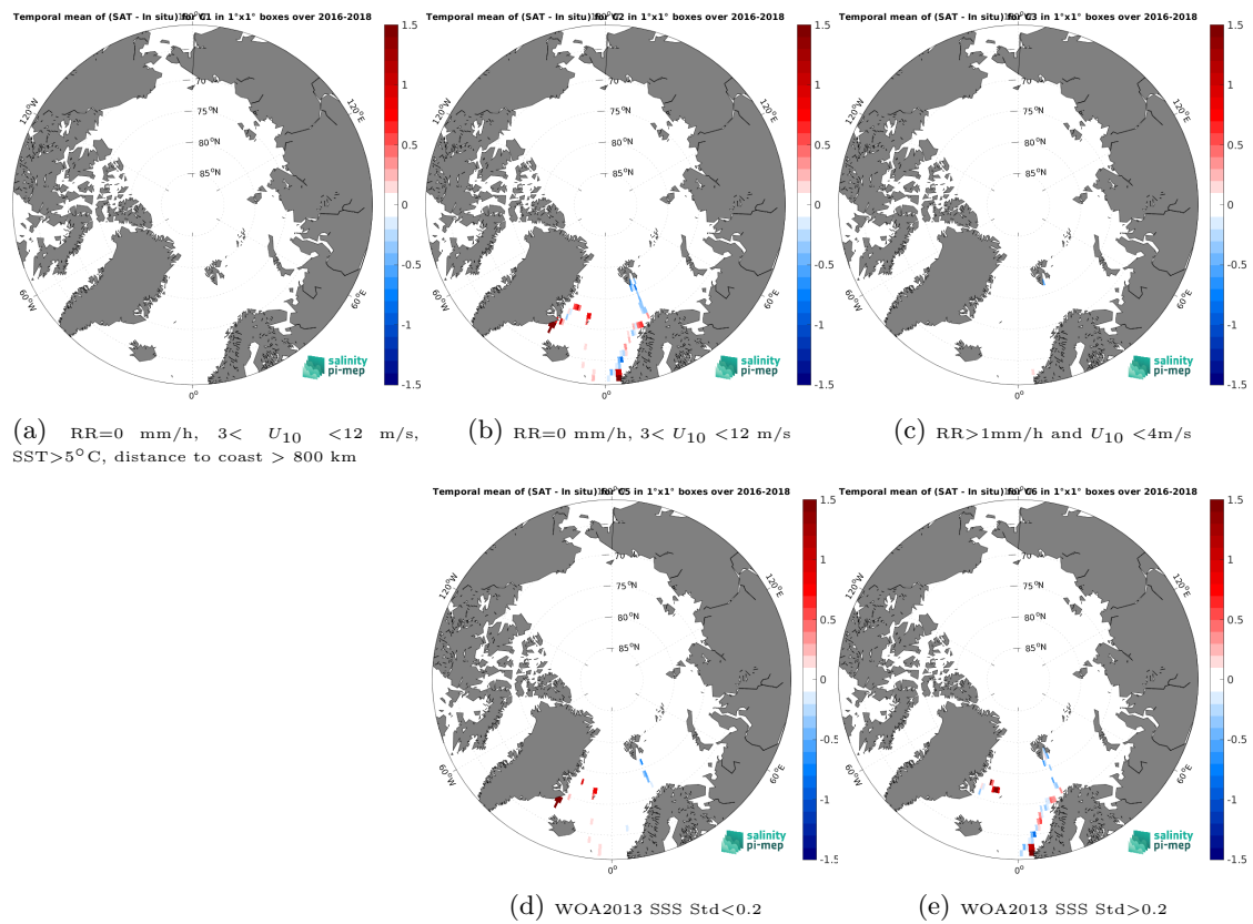
Figure 14: Temporal mean gridded over spatial boxes of size 1^\circ \times 1^\circ of \Delta SSS (SMOS SSS L3 Arctic v2 - 18 Days (CATDS-CEC-LOCEAN) - TSG (GOSUD-Research-vessel)) for 5 different subdatasets corresponding to: RR=0 mm/h, 3 < U_{10} < 12 m/s, SST > 5°C, distance to coast > 800 km (a), RR=0 mm/h, 3 < U_{10} < 12 m/s (b), RR > 1mm/h and U_{10} < 4 m/s (c), WOA2013 SSS Std < 0.2 (d), WOA2013 SSS Std > 0.2 (e).
