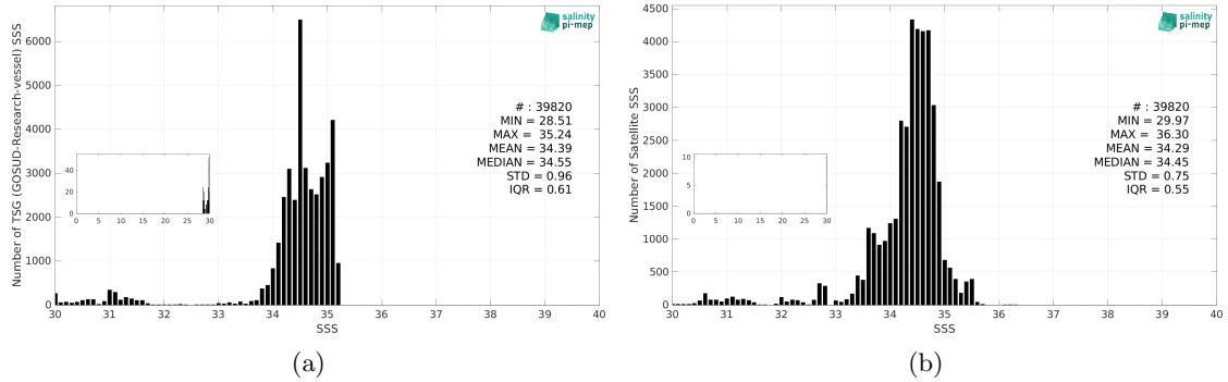
Figure 3: Histograms of SSS from TSG (GOSUD-Research-vessel) (a) and SMOS SSS L3 Arctic v2 - 18 Days (CATDS-CEC-LOCEAN) (b) considering all match-up pairs per bins of 0.1 over the Arctic Ocean Pi-MEP region and for the full satellite product period.
