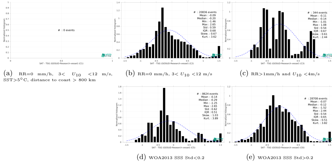
Figure 15: Normalized histogram of \Delta SSS (SMOS SSS L3 Arctic v2 - 18 Days (CATDS-CEC-LOCEAN) - TSG (GOSUD-Research-vessel)) for 5 different subdatasets corresponding to: RR=0 mm/h, 3 < U_{10} < 12 m/s, SST>5°C, distance to coast > 800 km (a), RR=0 mm/h, 3 < U_{10} < 12 m/s (b), RR>1mm/h and U_{10} < 4 m/s (c), WOA2013 SSS Std<0.2 (d), WOA2013 SSS Std>0.2 (e).
