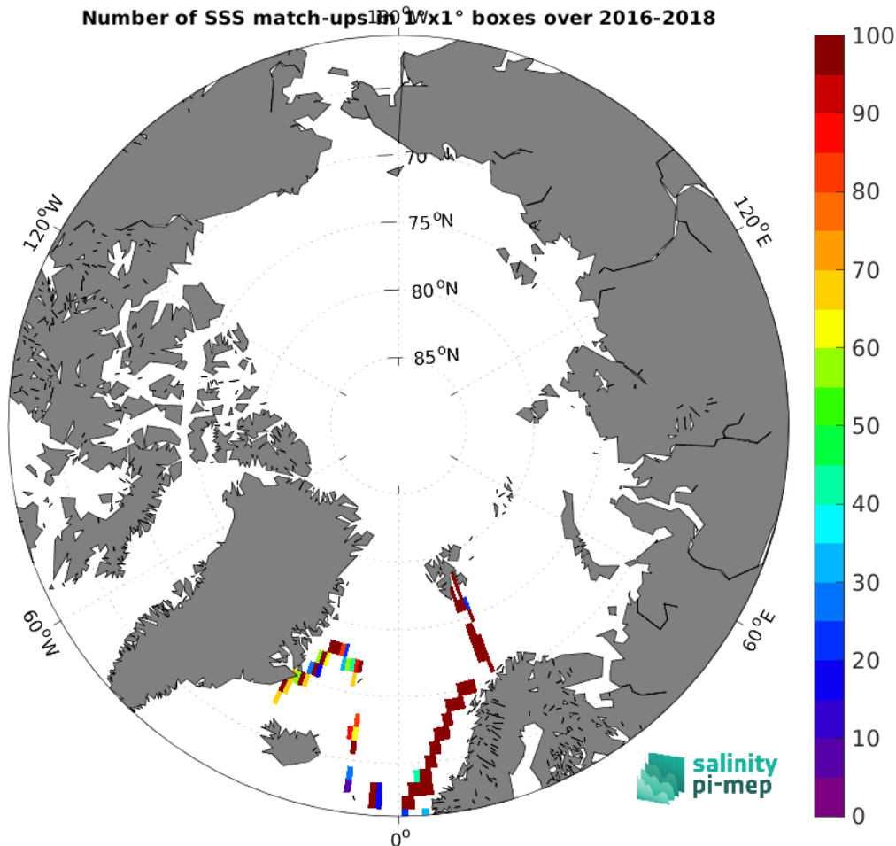
Figure 5: Number of SSS match-ups between TSG (GOSUD-Research-vessel) SSS and the SMOS SSS L3 Arctic v2 - 18 Days (CATDS-CEC-LOCEAN) SSS product for the Arctic Ocean Pi-MEP region over 1^\circ \times 1^\circ boxes and for the full satellite product period.
