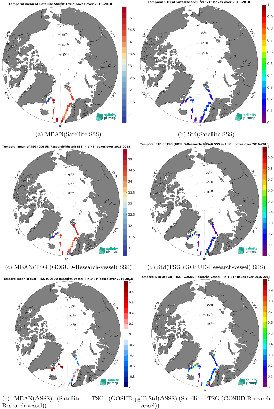
Figure 7: Temporal mean (left) and Std (right) of SSS from SMOS SSS L3 Arctic v2 - 18 Days (CATDS-CEC-LOCEAN) (top), TSG (GOSUD-Research-vessel) (middle), and of \Delta SSS (Satellite - TSG (GOSUD-Research-vessel)). Only match-up pairs are used to generate these maps.
