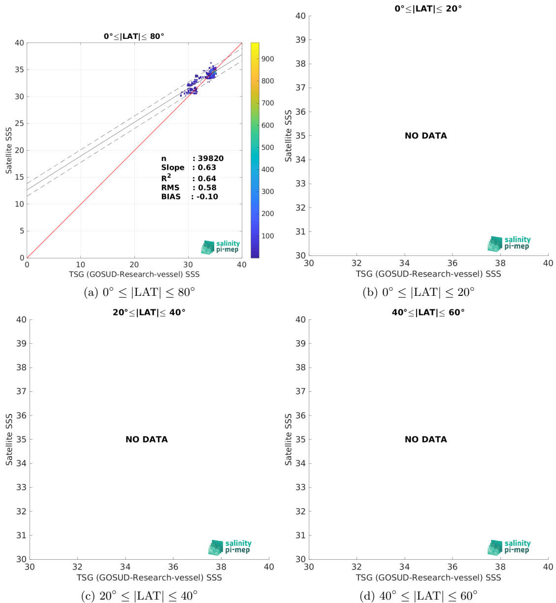
Figure 10: Contour maps of the concentration of SMOS SSS L3 Arctic v2 - 18 Days (CATDS-CEC-LOCEAN) SSS (y-axis) versus TSG (GOSUD-Research-vessel) SSS (x-axis) at match-up pairs for different latitude bands. For each plot, the red line shows x=y . The black thin and dashed lines indicate a linear fit through the data cloud and the \pm 95\% confidence levels, respectively. The number match-up pairs n , the slope and R^2 coefficient of the linear fit, the root mean square (RMS) and the mean bias between satellite and in situ data are indicated for each latitude band in each plots.
