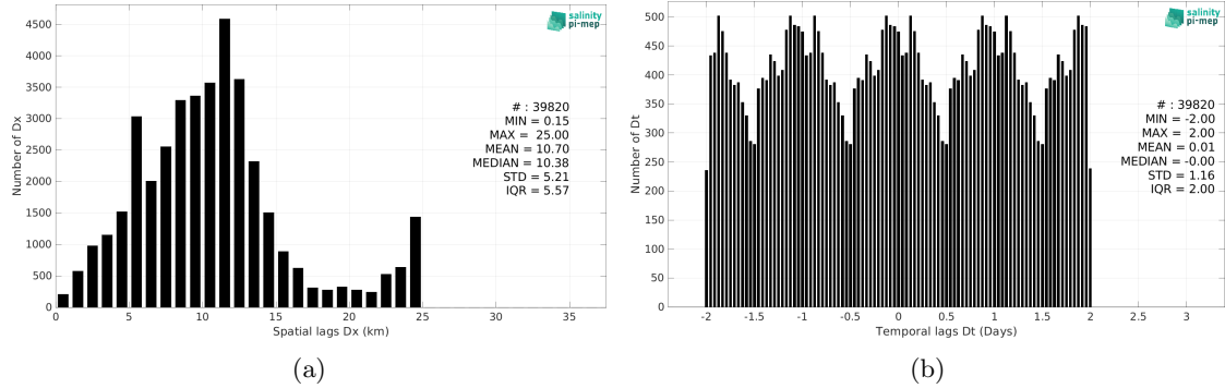
Figure 6: Histograms of the spatial (a) and temporal (b) lags between the location/time of the TSG (GOSUD-Research-vessel) measurement and the date of the corresponding SMOS SSS L3 Arctic v2 - 18 Days (CATDS-CEC-LOCEAN) SSS pixel.
