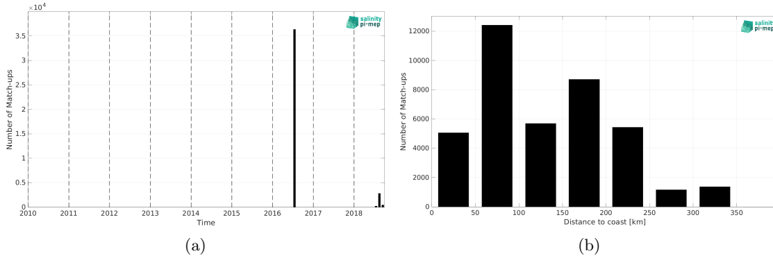
Figure 2: Number of match-ups between TSG (GOSUD-Research-vessel) and SMOS SSS L3 Arctic v2 - 18 Days (CATDS-CEC-LOCEAN) SSS as a function of time (a) and as function of the distance to coast (b) over the Arctic Ocean Pi-MEP region and for the full satellite product period.
