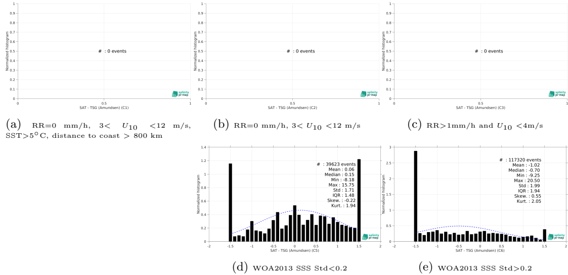
Figure 13: Normalized histogram of \Delta SSS (SMOS SSS L3 Arctic v2 - 18 Days (CATDS-CEC-LOCEAN) - TSG (Amundsen)) for 5 different subdatasets corresponding to: RR=0 mm/h, 3 < U_{10} < 12 m/s, SST>5°C, distance to coast > 800 km (a), RR=0 mm/h, 3 < U_{10} < 12 m/s (b), RR>1mm/h and U_{10} < 4 m/s (c), WOA2013 SSS Std<0.2 (d), WOA2013 SSS Std>0.2 (e).
