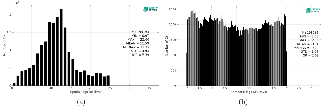
Figure 5: Histograms of the spatial (a) and temporal (b) lags between the location/time of the TSG (Amundsen) measurement and the date of the corresponding SMOS SSS L3 Arctic v2 - 18 Days (CATDS-CEC-LOCEAN) SSS pixel.
