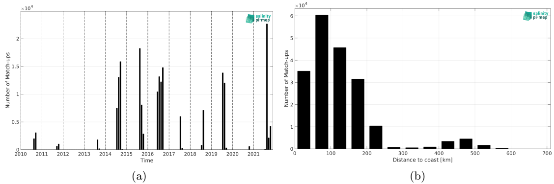
Figure 1: Number of match-ups between TSG (Amundsen) and SMOS SSS L3 Arctic v2 - 18 Days (CATDS-CEC-LOCEAN) SSS as a function of time (a) and as function of the distance to coast (b) over the Arctic Ocean Pi-MEP region and for the full satellite product period.
