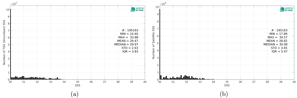
Figure 2: Histograms of SSS from TSG (Amundsen) (a) and SMOS SSS L3 Arctic v2 - 18 Days (CATDS-CEC-LOCEAN) (b) considering all match-up pairs per bins of 0.1 over the Arctic Ocean Pi-MEP region and for the full satellite product period.
