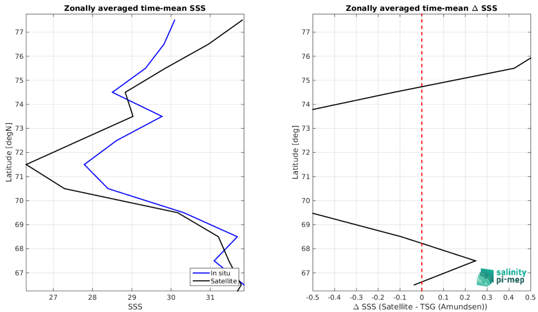
Figure 8: Left panel: Zonal mean SSS from SMOS SSS L3 Arctic v2 - 18 Days (CATDS-CEC-LOCEAN) satellite product (black) and from TSG (Amundsen) (blue). Right panel: Zonal mean of \Delta SSS (Satellite - TSG (Amundsen)) for all the collected Pi-MEP match-up pairs estimated over the full satellite product period.
