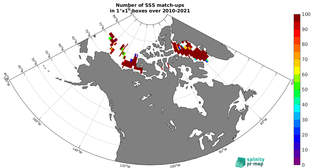
Figure 4: Number of SSS match-ups between TSG (Amundsen) SSS and the SMOS SSS L3 Arctic v2 - 18 Days (CATDS-CEC-LOCEAN) SSS product for the Arctic Ocean Pi-MEP region over 1^\circ \times 1^\circ boxes and for the full satellite product period.
