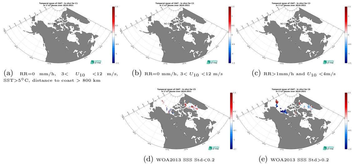
Figure 12: Temporal mean gridded over spatial boxes of size 1^{\circ}\times 1^{\circ} of \Delta\text{SSS} (SMOS SSS L3 Arctic v2 - 18 Days (CATDS-CEC-LOCEAN) - TSG (Amundsen)) for 5 different subdatasets corresponding to:RR=0 mm/h, 3 < U_{10} < 12 m/s, SST >5^{\circ}\text{C} , distance to coast > 800 km (a), RR=0 mm/h, 3 < U_{10} < 12 m/s (b), RR >1 mm/h and U_{10} < 4 m/s (c), WOA2013 SSS Std <0.2 (d), WOA2013 SSS Std >0.2 (e).
