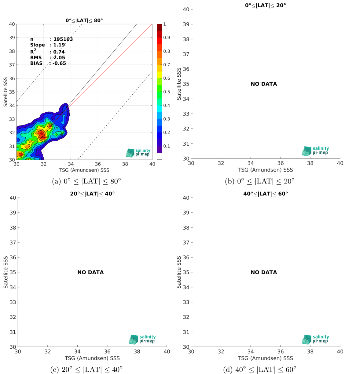
Figure 9: Contour maps of the concentration of SMOS SSS L3 Arctic v2 - 18 Days (CATDS-CEC-LOCEAN) SSS (y-axis) versus TSG (Amundsen) SSS (x-axis) at match-up pairs for different latitude bands. For each plot, the red line shows x=y . The black thin and dashed lines indicate a linear fit through the data cloud and the \pm 95\% confidence levels, respectively. The number match-up pairs n , the slope and R^2 coefficient of the linear fit, the root mean square (RMS) and the mean bias between satellite and in situ data are indicated for each latitude band in each plots.
