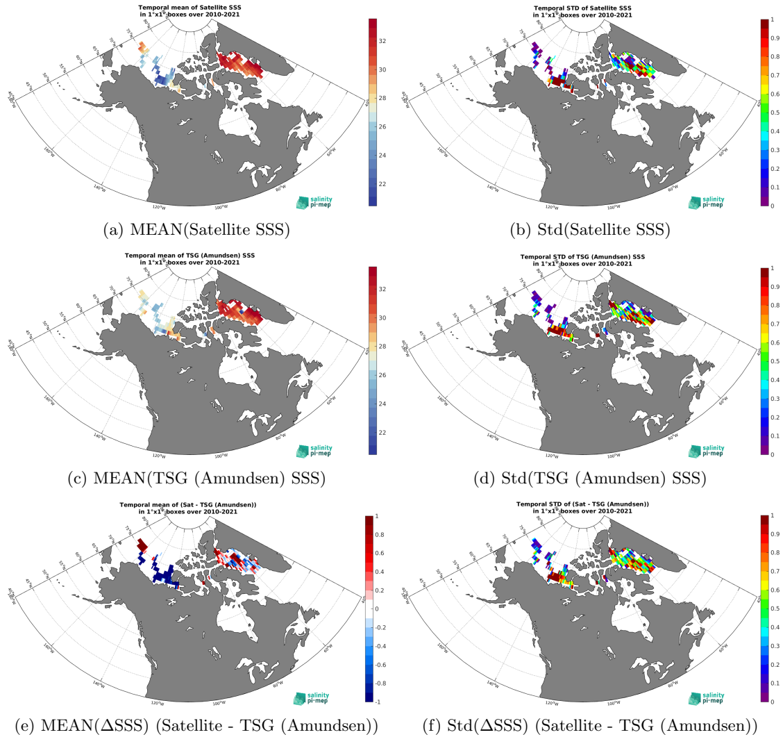
Figure 6: Temporal mean (left) and Std (right) of SSS from SMOS SSS L3 Arctic v2 - 18 Days (CATDS-CEC-LOCEAN) (top), TSG (Amundsen) (middle), and of \Delta SSS (Satellite - TSG (Amundsen)). Only match-up pairs are used to generate these maps.
