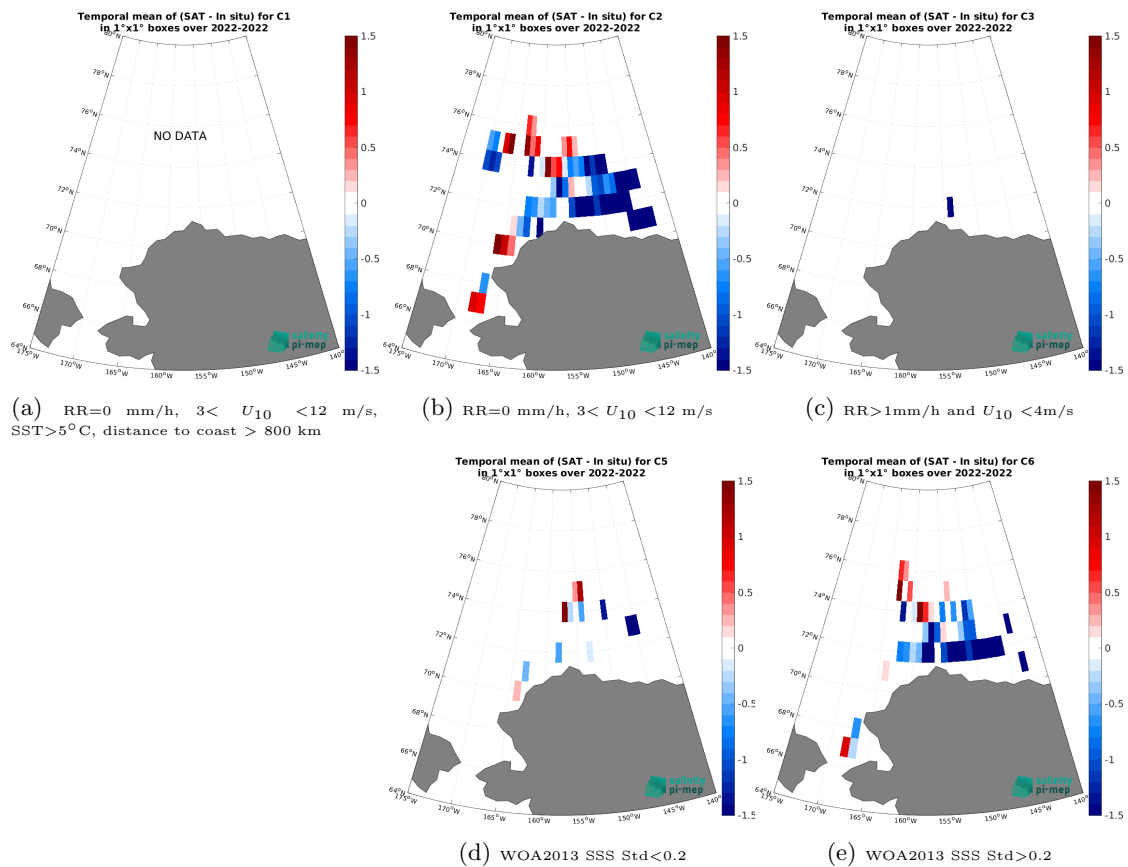
Figure 14: Temporal mean gridded over spatial boxes of size 1^\circ \times 1^\circ of \Delta SSS (SMOS SSS L3 Arctic v2 - 18 Days (CATDS-CEC-LOCEAN) - SASSIE) for 5 different subdatasets corresponding to:RR=0 mm/h, 3 < U_{10} < 12 m/s, SST>5°C, distance to coast > 800 km (a), RR=0 mm/h, 3 < U_{10} < 12 m/s (b), RR>1mm/h and U_{10} < 4 m/s (c), WOA2013 SSS Std<0.2 (d), WOA2013 SSS Std>0.2 (e).
