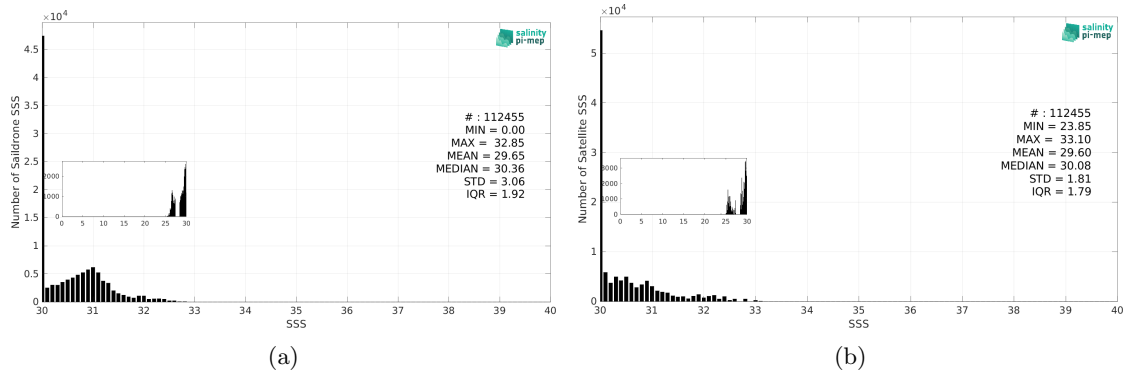
Figure 3: Histograms of SSS from Saildrone (a) and SMOS SSS L3 Arctic v2 - 18 Days (CATDS-CEC-LOCEAN) (b) considering all match-up pairs per bins of 0.1 over the Arctic Ocean Pi-MEP region and for the full satellite product period.
