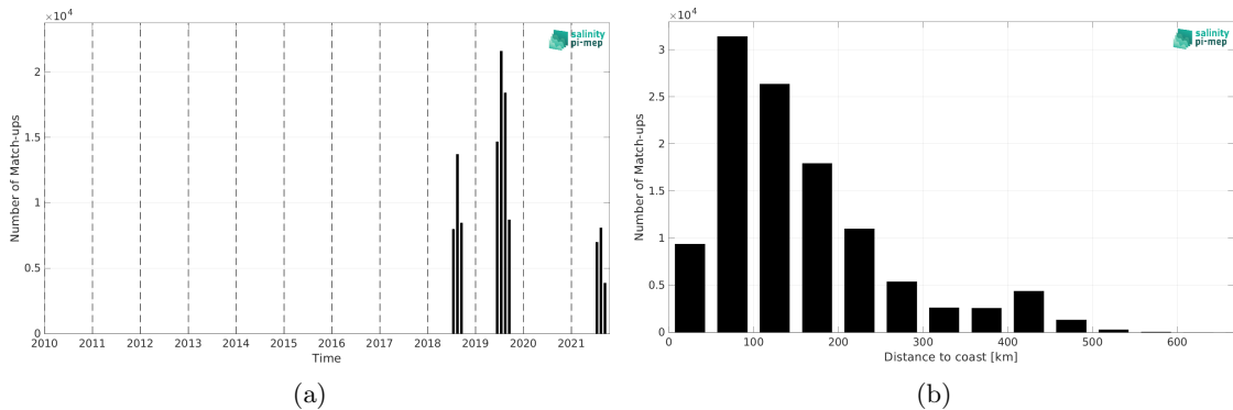
Figure 2: Number of match-ups between Saildrone and SMOS SSS L3 Arctic v2 - 18 Days (CATDS-CEC-LOCEAN) SSS as a function of time (a) and as function of the distance to coast (b) over the Arctic Ocean Pi-MEP region and for the full satellite product period.
