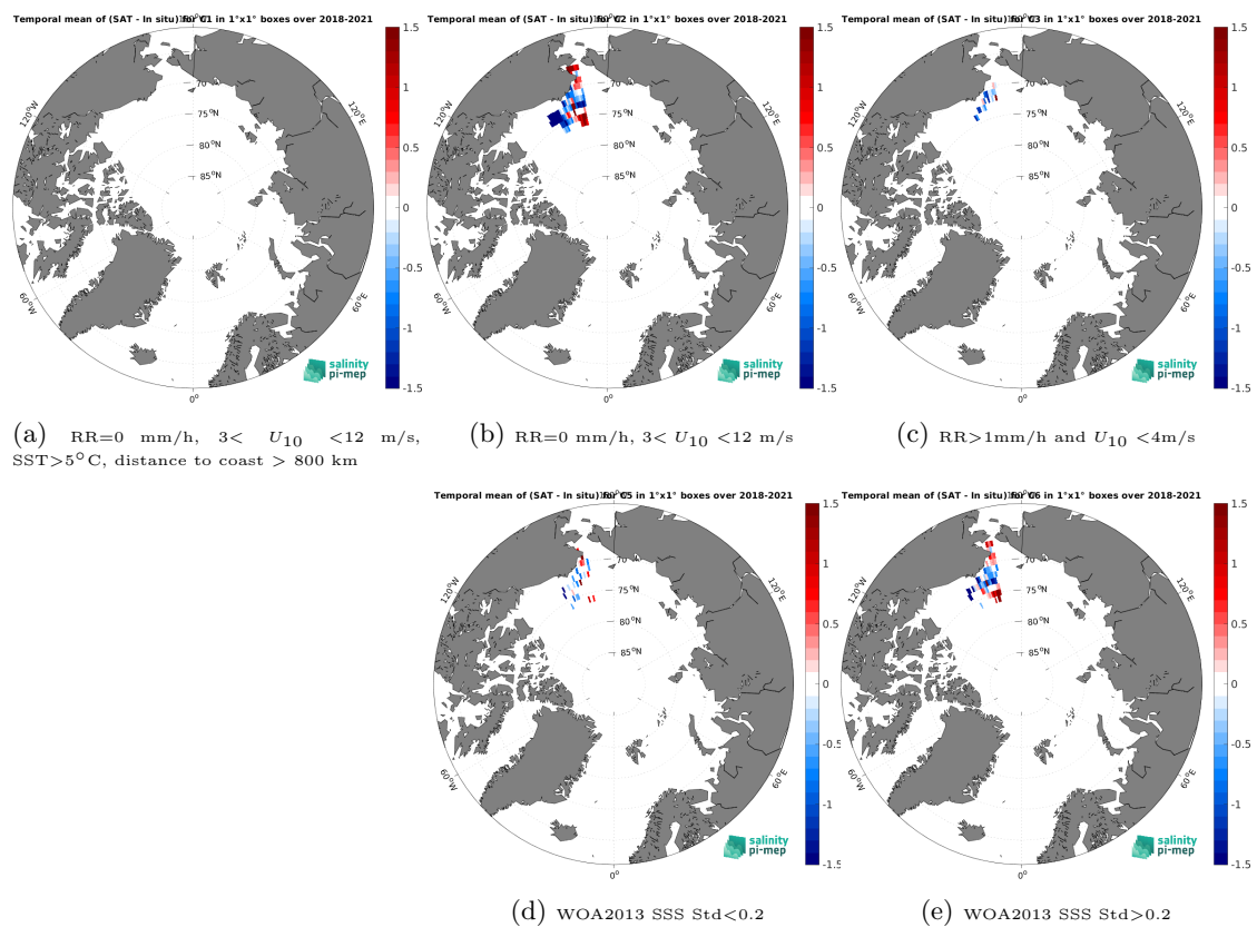
Figure 14: Temporal mean gridded over spatial boxes of size 1^\circ \times 1^\circ of \Delta SSS (SMOS SSS L3 Arctic v2 - 18 Days (CATDS-CEC-LOCEAN) - Sailydrone) for 5 different subdatasets corresponding to:RR=0 mm/h, 3 < U_{10} < 12 m/s, SST >5^\circ\text{C} , distance to coast > 800 km (a), RR=0 mm/h, 3 < U_{10} < 12 m/s (b), RR >1 mm/h and U_{10} < 4 m/s (c), WOA2013 SSS Std <0.2 (d), WOA2013 SSS Std >0.2 (e).
