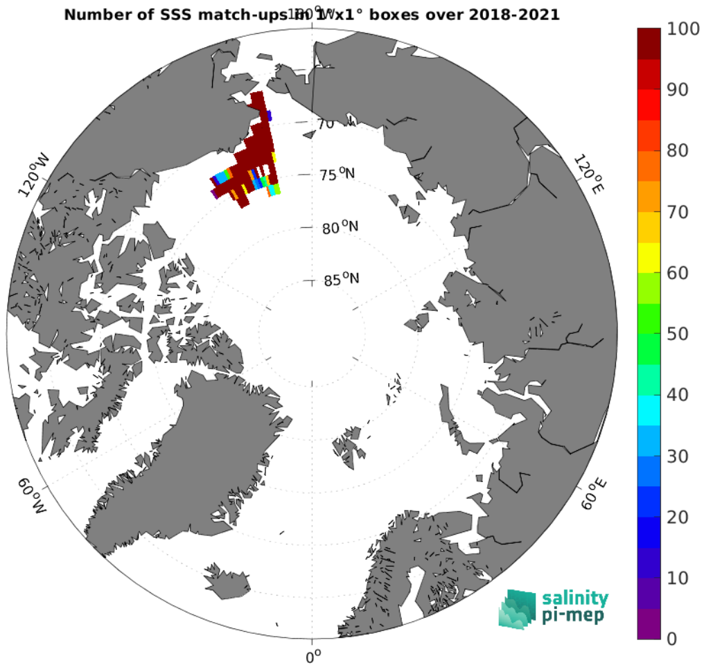
Figure 5: Number of SSS match-ups between Saildrone SSS and the SMOS SSS L3 Arctic v2 - 18 Days (CATDS-CEC-LOCEAN) SSS product for the Arctic Ocean Pi-MEP region over 1^\circ \times 1^\circ boxes and for the full satellite product period.
