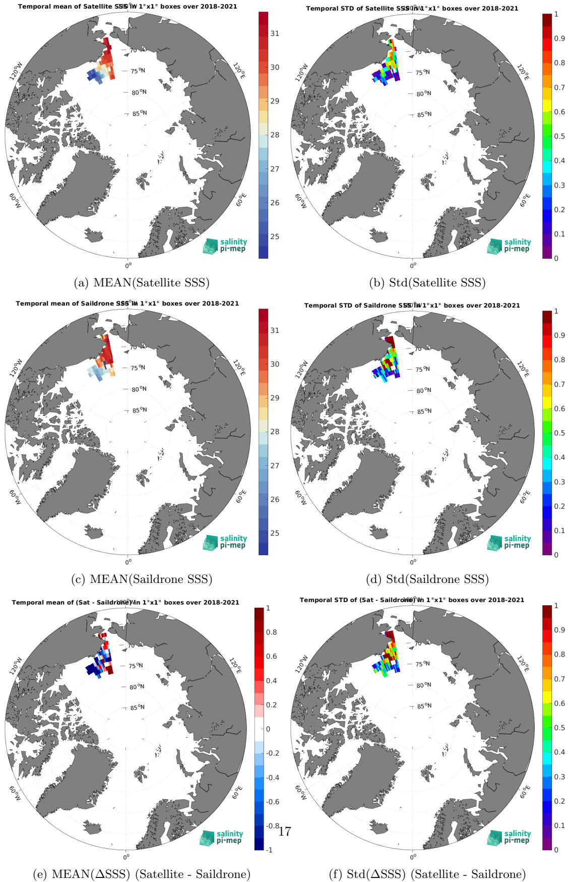
Figure 7: Temporal mean (left) and Std (right) of SSS from SMOS SSS L3 Arctic v2 - 18 Days (CATDS-CEC-LOCEAN) (top), Saildrone (middle), and of \Delta SSS (Satellite - Saildrone). Only match-up pairs are used to generate these maps.
