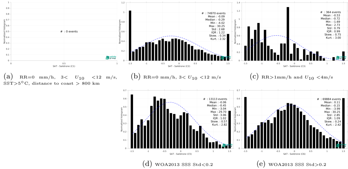
Figure 15: Normalized histogram of \Delta SSS (SMOS SSS L3 Arctic v2 - 18 Days (CATDS-CEC-LOCEAN) - Saldrone) for 5 different subdatasets corresponding to: RR=0 mm/h, 3 < U_{10} < 12 m/s, SST > 5°C, distance to coast > 800 km (a), RR=0 mm/h, 3 < U_{10} < 12 m/s (b), RR > 1mm/h and U_{10} < 4 m/s (c), WOA2013 SSS Std < 0.2 (d), WOA2013 SSS Std > 0.2 (e).
