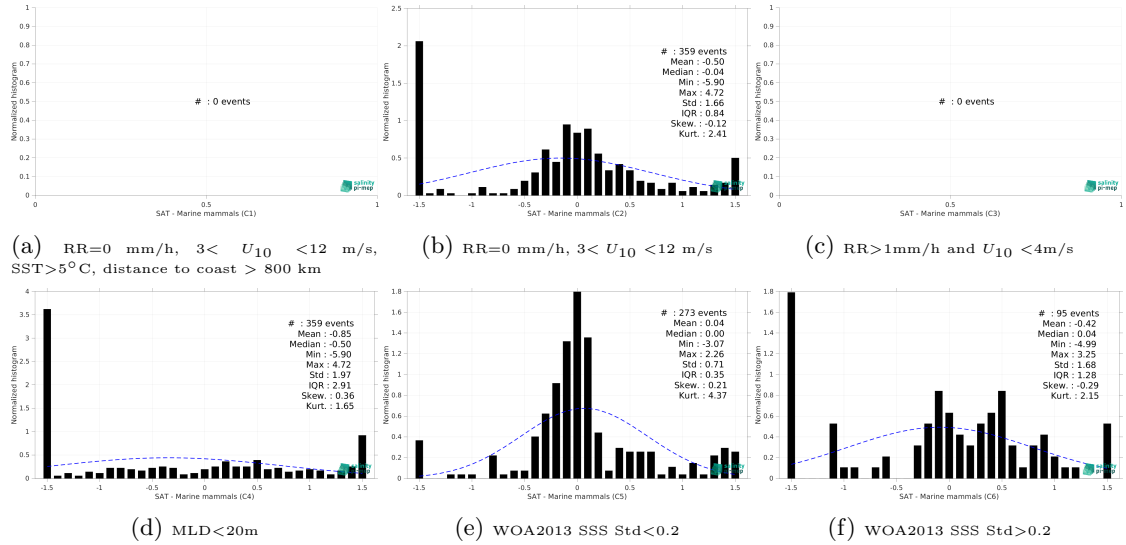
Figure 15: Normalized histogram of \Delta SSS (SMOS SSS L3 Arctic v2 - 18 Days (CATDS-CEC-LOCEAN) - Marine mammals) for 6 different subdatasets corresponding to: RR=0 mm/h, 3 < U_{10} < 12 m/s, SST>5°C, distance to coast > 800 km (a), RR=0 mm/h, 3 < U_{10} < 12 m/s (b), RR>1mm/h and U_{10} < 4 m/s (c), MLD<20m (d), WOA2013 SSS Std<0.2 (e), WOA2013 SSS Std>0.2 (f).
