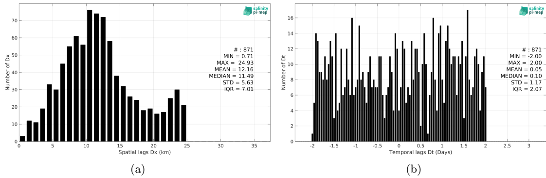
Figure 5: Histograms of the spatial (a) and temporal (b) lags between the location/time of the Marine mammals measurement and the date of the corresponding SMOS SSS L3 Arctic v2 - 18 Days (CATDS-CEC-LOCEAN) SSS pixel.
