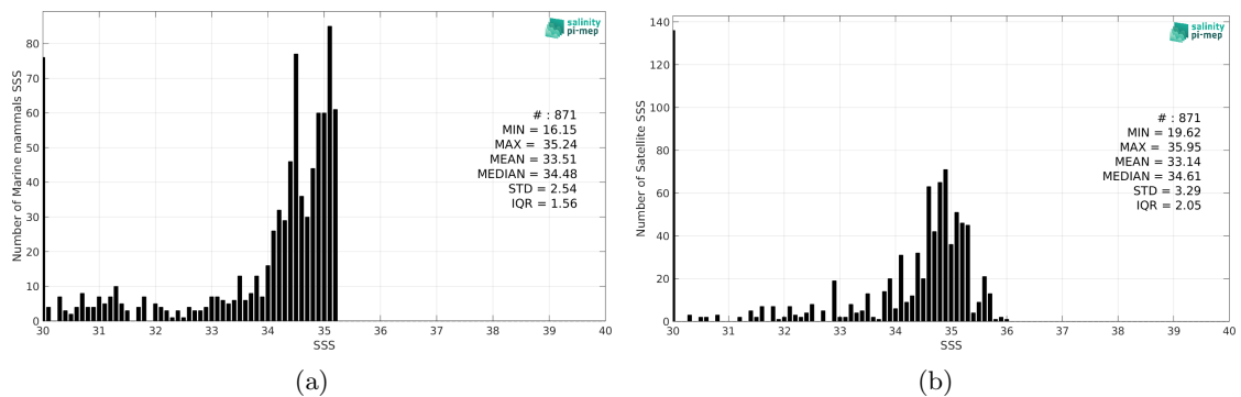
Figure 2: Histograms of SSS from Marine mammals (a) and SMOS SSS L3 Arctic v2 - 18 Days (CATDS-CEC-LOCEAN) (b) considering all match-up pairs per bins of 0.1 over the Arctic Ocean Pi-MEP region and for the full satellite product period.
