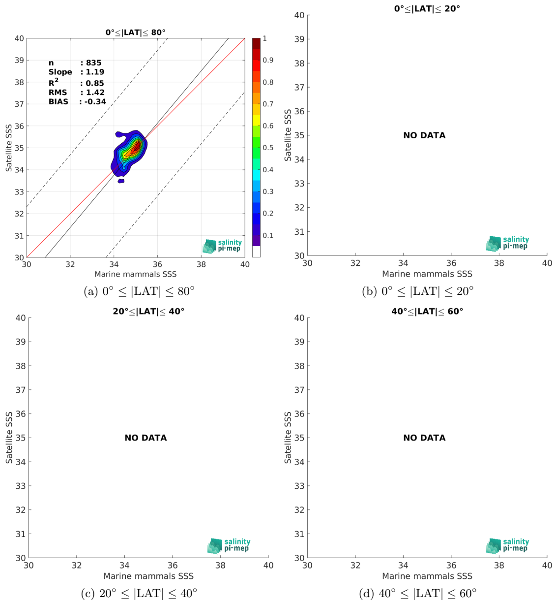
Figure 9: Contour maps of the concentration of SMOS SSS L3 Arctic v2 - 18 Days (CATDS-CEC-LOCEAN) SSS (y-axis) versus Marine mammals SSS (x-axis) at match-up pairs for different latitude bands. For each plot, the red line shows x=y . The black thin and dashed lines indicate a linear fit through the data cloud and the \pm 95\% confidence levels, respectively. The number match-up pairs n , the slope and R^2 coefficient of the linear fit, the root mean square (RMS) and the mean bias between satellite and in situ data are indicated for each latitude band in each plots.
