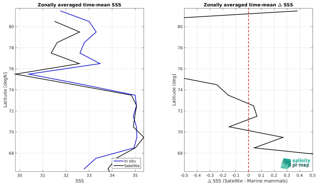
Figure 8: Left panel: Zonal mean SSS from SMOS SSS L3 Arctic v2 - 18 Days (CATDS-CEC-LOCEAN) satellite product (black) and from Marine mammals (blue). Right panel: Zonal mean of \Delta SSS (Satellite - Marine mammals) for all the collected Pi-MEP match-up pairs estimated over the full satellite product period.
