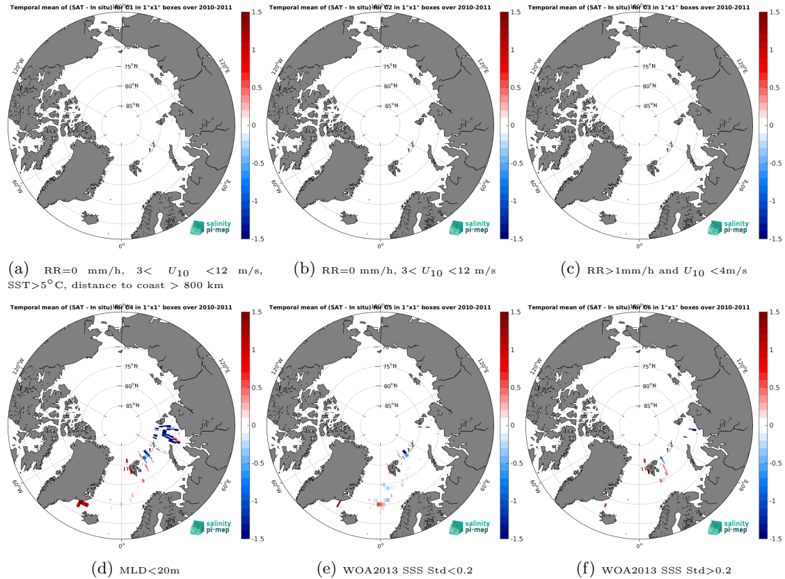
Figure 12: Temporal mean gridded over spatial boxes of size 1^{\circ}\times 1^{\circ} of \Delta\text{SSS} (SMOS SSS L3 Arctic v2 - 18 Days (CATDS-CEC-LOCEAN) - Marine mammals) for 6 different subdatasets corresponding to:RR=0 mm/h, 3 < U_{10} < 12 m/s, SST >5^{\circ}\text{C} , distance to coast > 800 km (a), RR=0 mm/h, 3 < U_{10} < 12 m/s (b), RR >1 mm/h and U_{10} < 4 m/s (c),MLD <20 m (d),WOA2013 SSS Std <0.2 (e),WOA2013 SSS Std >0.2 (f).
