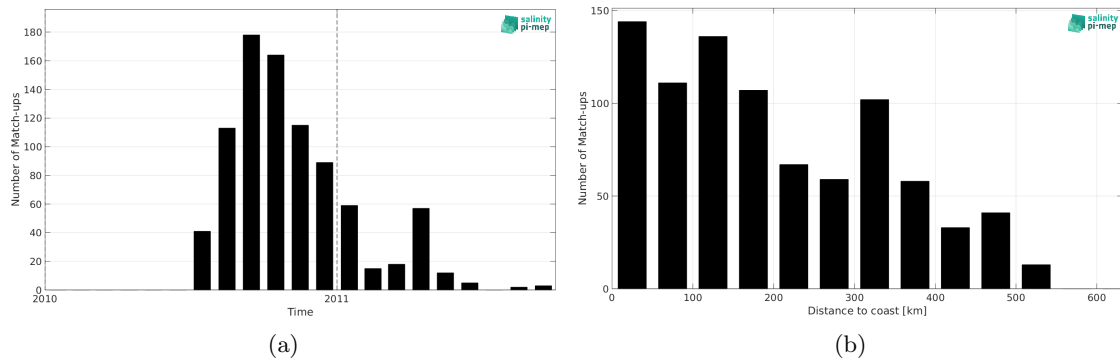
Figure 1: Number of match-ups between Marine mammals and SMOS SSS L3 Arctic v2 - 18 Days (CATDS-CEC-LOCEAN) SSS as a function of time (a) and as function of the distance to coast (b) over the Arctic Ocean Pi-MEP region and for the full satellite product period.
