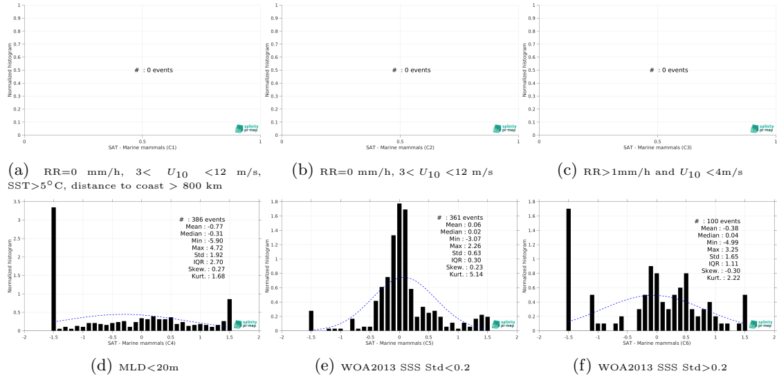
Figure 13: Normalized histogram of \Delta SSS (SMOS SSS L3 Arctic v2 - 18 Days (CATDS-CEC-LOCEAN) - Marine mammals) for 6 different subdatasets corresponding to: RR=0 mm/h, 3 < U_{10} < 12 m/s, SST>5°C, distance to coast > 800 km (a), RR=0 mm/h, 3 < U_{10} < 12 m/s (b), RR>1mm/h and U_{10} < 4 m/s (c), MLD<20m (d), WOA2013 SSS Std<0.2 (e), WOA2013 SSS Std>0.2 (f).
