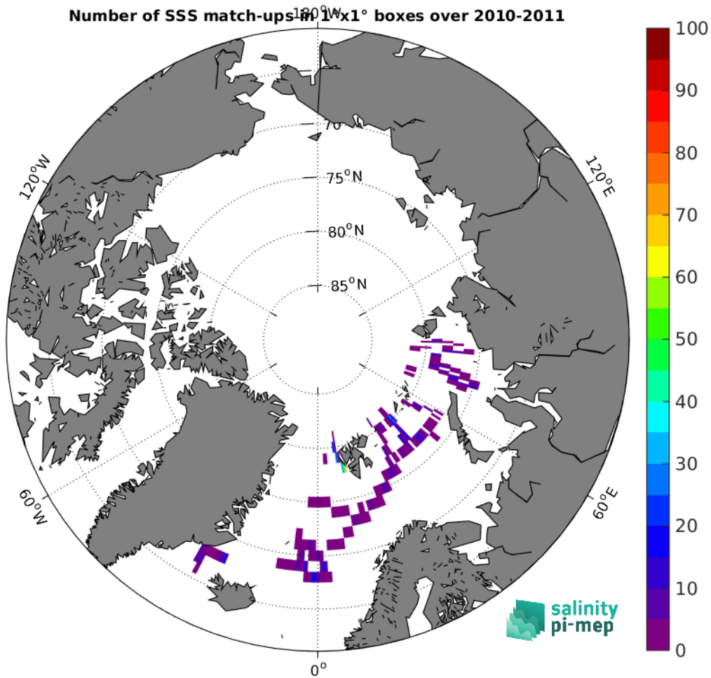
Figure 4: Number of SSS match-ups between Marine mammals SSS and the SMOS SSS L3 Arctic v2 - 18 Days (CATDS-CEC-LOCEAN) SSS product for the Arctic Ocean Pi-MEP region over 1^\circ \times 1^\circ boxes and for the full satellite product period.
