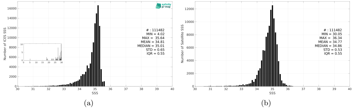
Figure 3: Histograms of SSS from ICES (a) and SMOS SSS L3 Arctic v2 - 18 Days (CATDS-CEC-LOCEAN) (b) considering all match-up pairs per bins of 0.1 over the Arctic Ocean Pi-MEP region and for the full satellite product period.
