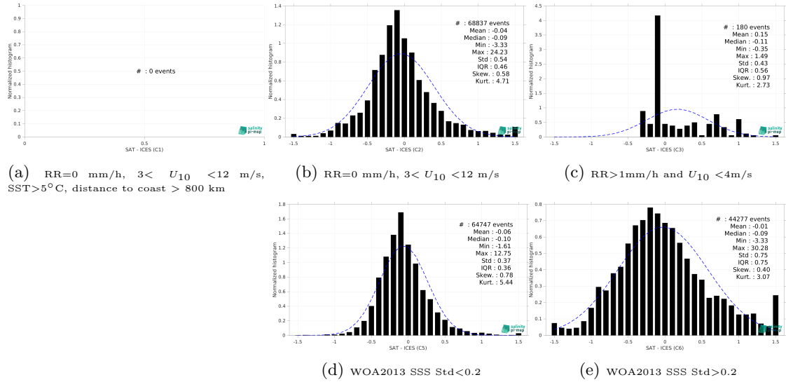
Figure 15: Normalized histogram of \Delta SSS (SMOS SSS L3 Arctic v2 - 18 Days (CATDS-CEC-LOCEAN) - ICES) for 5 different subdatasets corresponding to: RR=0 mm/h, 3 < U_{10} < 12 m/s, SST > 5°C, distance to coast > 800 km (a), RR=0 mm/h, 3 < U_{10} < 12 m/s (b), RR > 1mm/h and U_{10} < 4 m/s (c), WOA2013 SSS Std < 0.2 (d), WOA2013 SSS Std > 0.2 (e).
