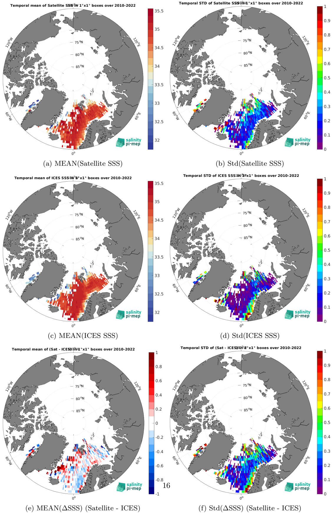
Figure 7: Temporal mean (left) and Std (right) of SSS from SMOS SSS L3 Arctic v2 - 18 Days (CATDS-CEC-LOCEAN) (top), ICES (middle), and of \Delta SSS (Satellite - ICES). Only match-up pairs are used to generate these maps.
