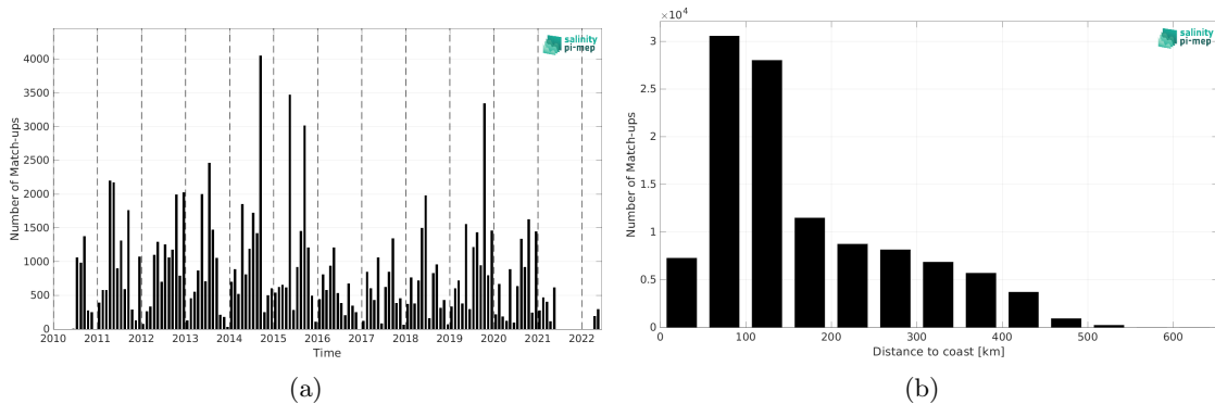
Figure 2: Number of match-ups between ICES and SMOS SSS L3 Arctic v2 - 18 Days (CATDS-CEC-LOCEAN) SSS as a function of time (a) and as function of the distance to coast (b) over the Arctic Ocean Pi-MEP region and for the full satellite product period.
