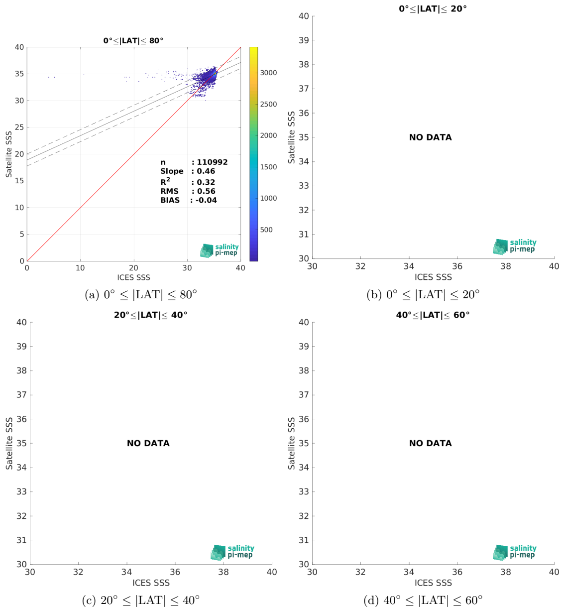
Figure 10: Contour maps of the concentration of SMOS SSS L3 Arctic v2 - 18 Days (CATDS-CEC-LOCEAN) SSS (y-axis) versus ICES SSS (x-axis) at match-up pairs for different latitude bands. For each plot, the red line shows x=y . The black thin and dashed lines indicate a linear fit through the data cloud and the \pm 95\% confidence levels, respectively. The number match-up pairs n , the slope and R^2 coefficient of the linear fit, the root mean square (RMS) and the mean bias between satellite and in situ data are indicated for each latitude band in each plots.
