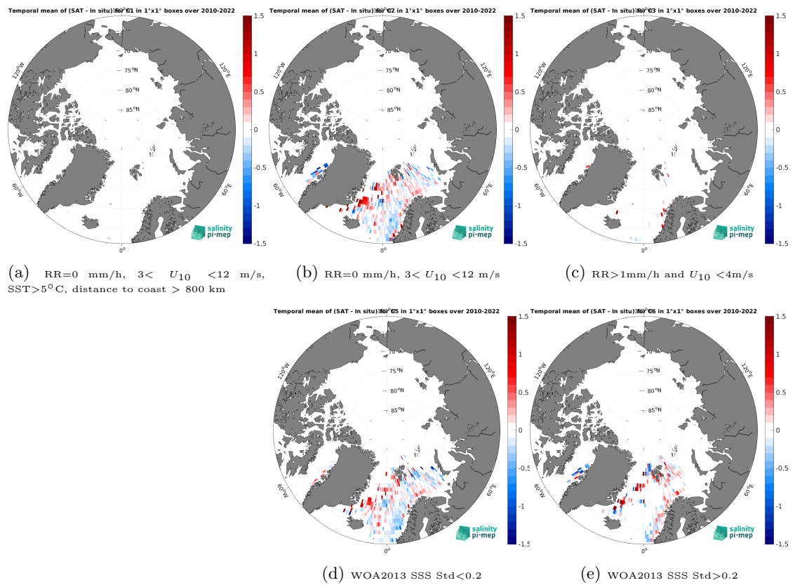
Figure 14: Temporal mean gridded over spatial boxes of size 1^\circ \times 1^\circ of \Delta SSS (SMOS SSS L3 Arctic v2 - 18 Days (CATDS-CEC-LOCEAN) - ICES) for 5 different subdatasets corresponding to:RR=0 mm/h, 3 < U_{10} < 12 m/s, SST >5^\circ C, distance to coast > 800 km (a), RR=0 mm/h, 3 < U_{10} < 12 m/s (b), RR >1 mm/h and U_{10} < 4 m/s (c), WOA2013 SSS Std <0.2 (d), WOA2013 SSS Std >0.2 (e).
