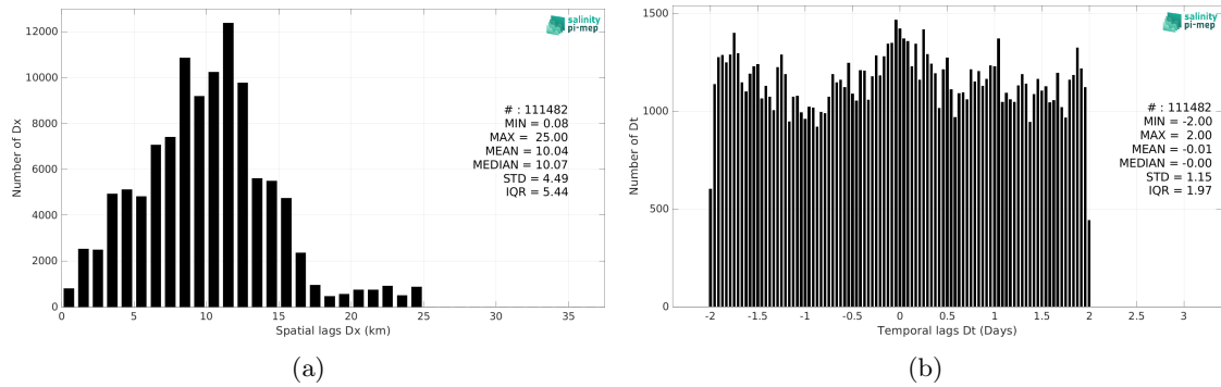
Figure 6: Histograms of the spatial (a) and temporal (b) lags between the location/time of the ICES measurement and the date of the corresponding SMOS SSS L3 Arctic v2 - 18 Days (CATDS-CEC-LOCEAN) SSS pixel.
