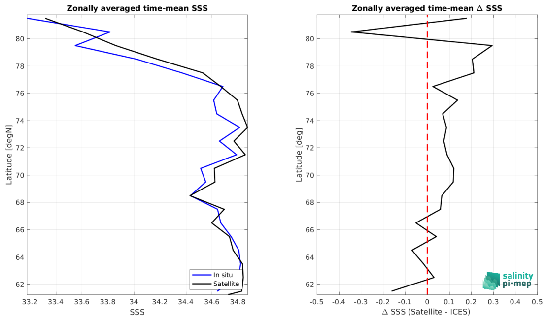
Figure 9: Left panel: Zonal mean SSS from SMOS SSS L3 Arctic v2 - 18 Days (CATDS-CEC-LOCEAN) satellite product (black) and from ICES (blue). Right panel: Zonal mean of \Delta SSS (Satellite - ICES) for all the collected Pi-MEP match-up pairs estimated over the full satellite product period.
