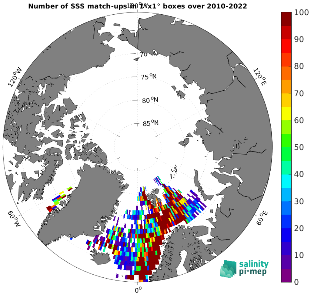
Figure 5: Number of SSS match-ups between ICES SSS and the SMOS SSS L3 Arctic v2 - 18 Days (CATDS-CEC-LOCEAN) SSS product for the Arctic Ocean Pi-MEP region over 1^\circ \times 1^\circ boxes and for the full satellite product period.
