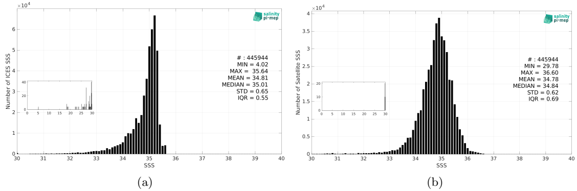
Figure 3: Histograms of SSS from ICES (a) and SMOS SSS L3 Arctic v2 - 18 Days (CATDS-CEC-LOCEAN) (b) considering all match-up pairs per bins of 0.1 over the Arctic Ocean Pi-MEP region and for the full satellite product period.
