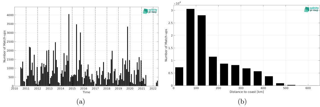
Figure 1: Number of match-ups between ICES and SMOS SSS L3 Arctic v2 - 18 Days (CATDS-CEC-LOCEAN) SSS as a function of time (a) and as function of the distance to coast (b) over the Arctic Ocean Pi-MEP region and for the full satellite product period.
