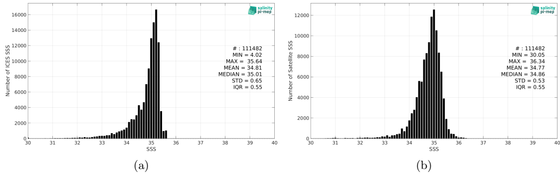
Figure 2: Histograms of SSS from ICES (a) and SMOS SSS L3 Arctic v2 - 18 Days (CATDS-CEC-LOCEAN) (b) considering all match-up pairs per bins of 0.1 over the Arctic Ocean Pi-MEP region and for the full satellite product period.
