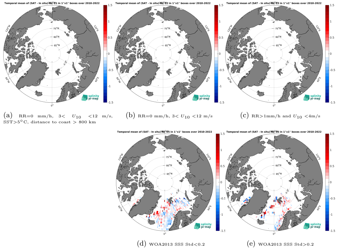
Figure 12: Temporal mean gridded over spatial boxes of size 1^{\circ}\times 1^{\circ} of \Delta\text{SSS} (SMOS SSS L3 Arctic v2 - 18 Days (CATDS-CEC-LOCEAN) - ICES) for 5 different subdatasets corresponding to: RR=0 mm/h, 3 < U_{10} < 12 m/s, SST > 5^{\circ}\text{C} , distance to coast > 800 km (a), RR=0 mm/h, 3 < U_{10} < 12 m/s (b), RR > 1 mm/h and U_{10} < 4 m/s (c), WOA2013 SSS Std < 0.2 (d), WOA2013 SSS Std > 0.2 (e).
