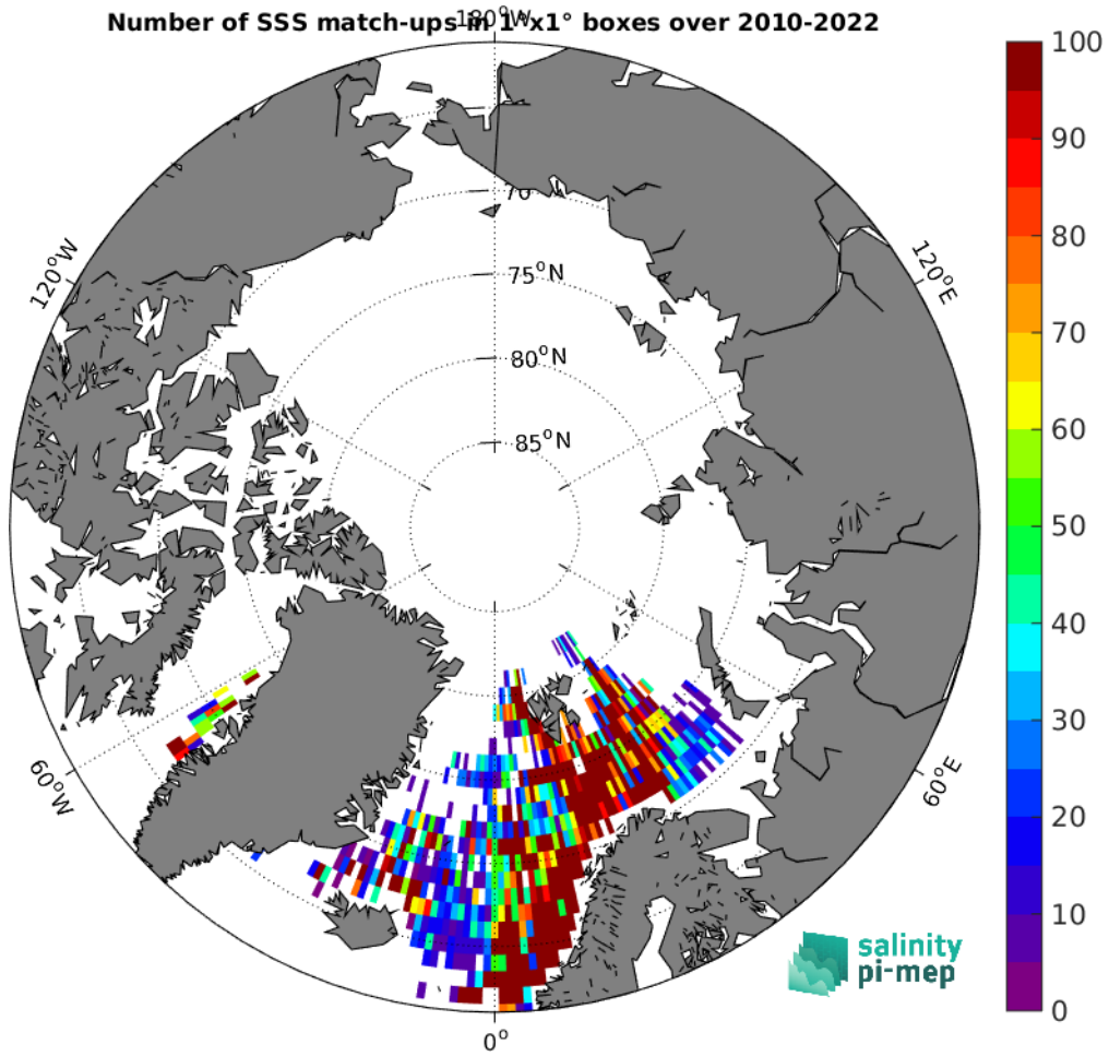
Figure 4: Number of SSS match-ups between ICES SSS and the SMOS SSS L3 Arctic v2 - 18 Days (CATDS-CEC-LOCEAN) SSS product for the Arctic Ocean Pi-MEP region over 1^\circ \times 1^\circ boxes and for the full satellite product period.
