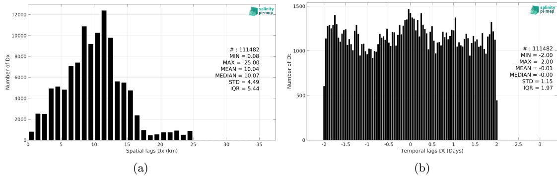
Figure 5: Histograms of the spatial (a) and temporal (b) lags between the location/time of the ICES measurement and the date of the corresponding SMOS SSS L3 Arctic v2 - 18 Days (CATDS-CEC-LOCEAN) SSS pixel.
