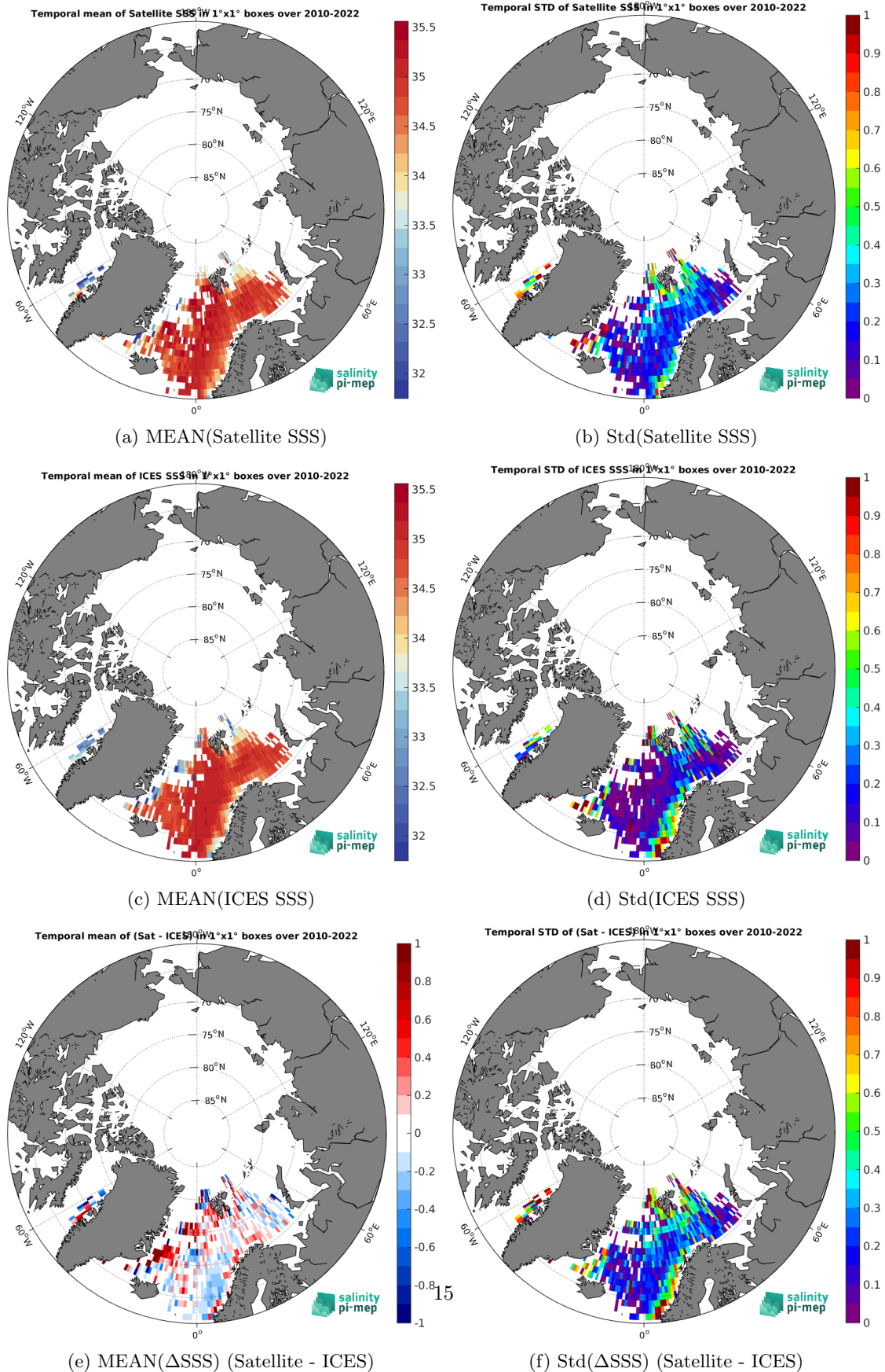
Figure 6: Temporal mean (left) and Std (right) of SSS from SMOS SSS L3 Arctic v2 - 18 Days (CATDS-CEC-LOCEAN) (top), ICES (middle), and of \Delta SSS (Satellite - ICES). Only match-up pairs are used to generate these maps.
