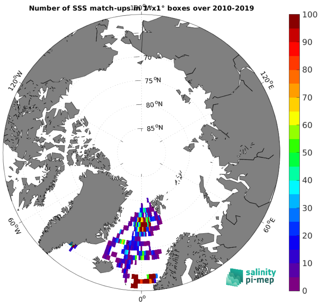
Figure 4: Number of SSS match-ups between Surface drifters SSS and the SMOS SSS L3 Arctic v2 - 18 Days (CATDS-CEC-LOCEAN) SSS product for the Arctic Ocean Pi-MEP region over 1^{\circ} \times 1^{\circ} boxes and for the full satellite product period.
