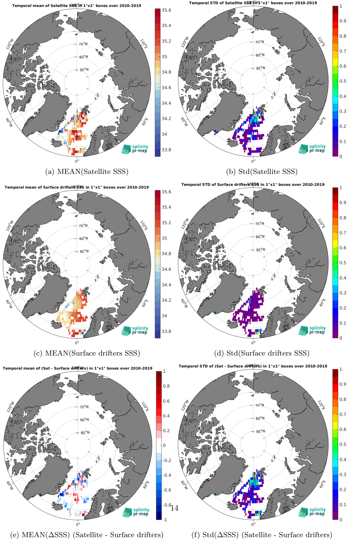
Figure 5: Temporal mean (left) and Std (right) of SSS from SMOS SSS L3 Arctic v2 - 18 Days (CATDS-CEC-LOCEAN) (top), Surface drifters (middle), and of \Delta SSS (Satellite - Surface drifters). Only match-up pairs are used to generate these maps.
