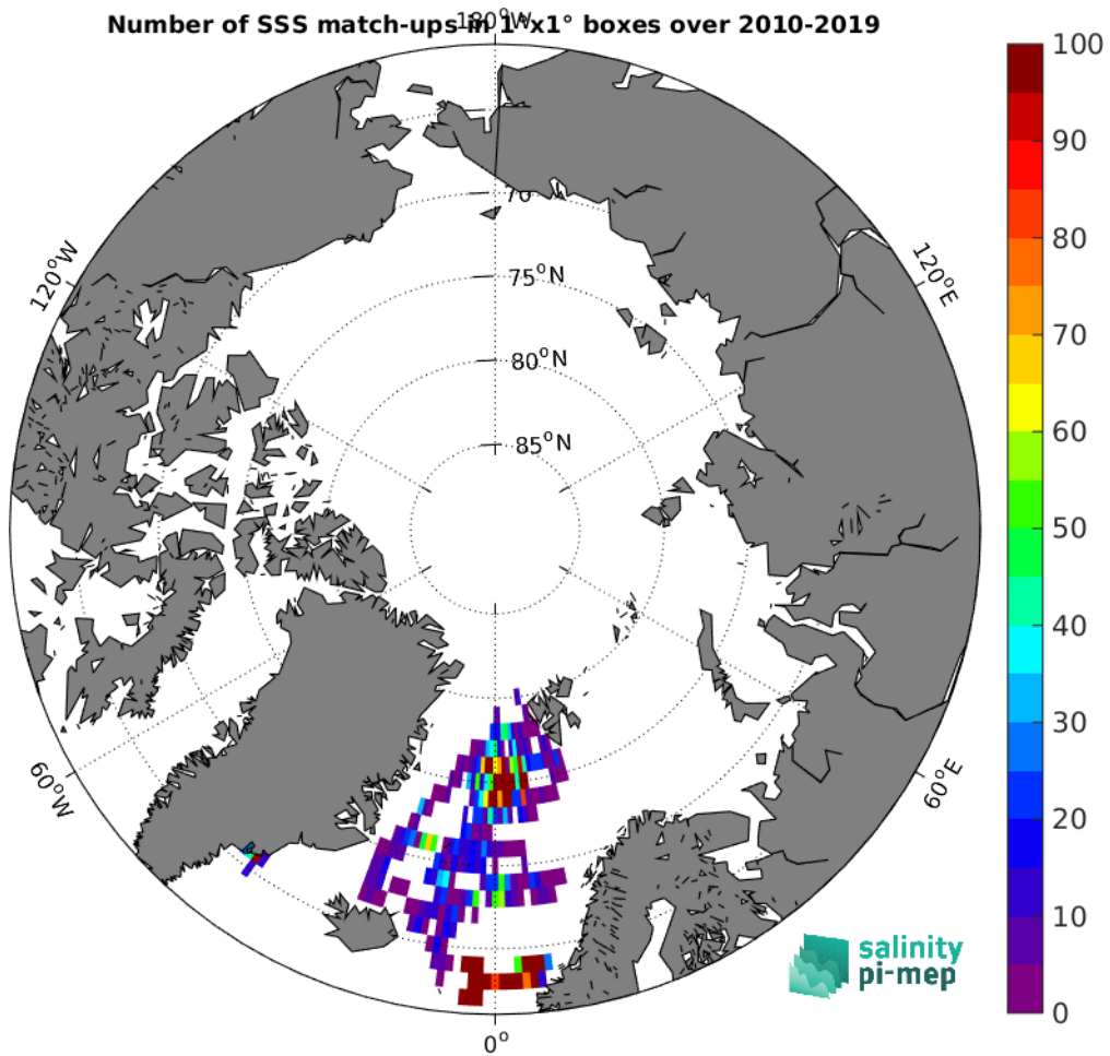
Figure 3: Number of SSS match-ups between Surface drifters SSS and the SMOS SSS L3 Arctic v2 - 18 Days (CATDS-CEC-LOCEAN) SSS product for the Arctic Ocean Pi-MEP region over 1^\circ \times 1^\circ boxes and for the full satellite product period.
