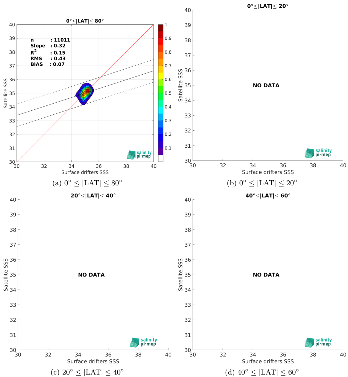
Figure 8: Contour maps of the concentration of SMOS SSS L3 Arctic v2 - 18 Days (CATDS-CEC-LOCEAN) SSS (y-axis) versus Surface drifters SSS (x-axis) at match-up pairs for different latitude bands. For each plot, the red line shows x=y . The black thin and dashed lines indicate a linear fit through the data cloud and the \pm 95\% confidence levels, respectively. The number match-up pairs n , the slope and R^2 coefficient of the linear fit, the root mean square (RMS) and the mean bias between satellite and in situ data are indicated for each latitude band in each plots.
