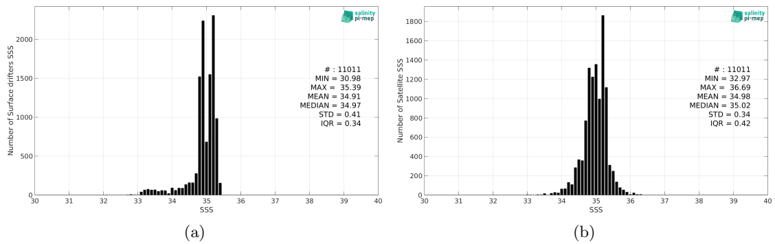
Figure 2: Histograms of SSS from Surface drifters (a) and SMOS SSS L3 Arctic v2 - 18 Days (CATDS-CEC-LOCEAN) (b) considering all match-up pairs per bins of 0.1 over the Arctic Ocean Pi-MEP region and for the full satellite product period.
