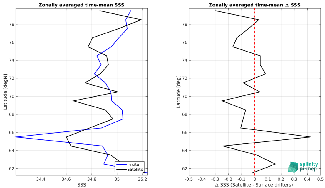
Figure 7: Left panel: Zonal mean SSS from SMOS SSS L3 Arctic v2 - 18 Days (CATDS-CEC-LOCEAN) satellite product (black) and from Surface drifters (blue). Right panel: Zonal mean of \Delta SSS (Satellite - Surface drifters) for all the collected Pi-MEP match-up pairs estimated over the full satellite product period.
