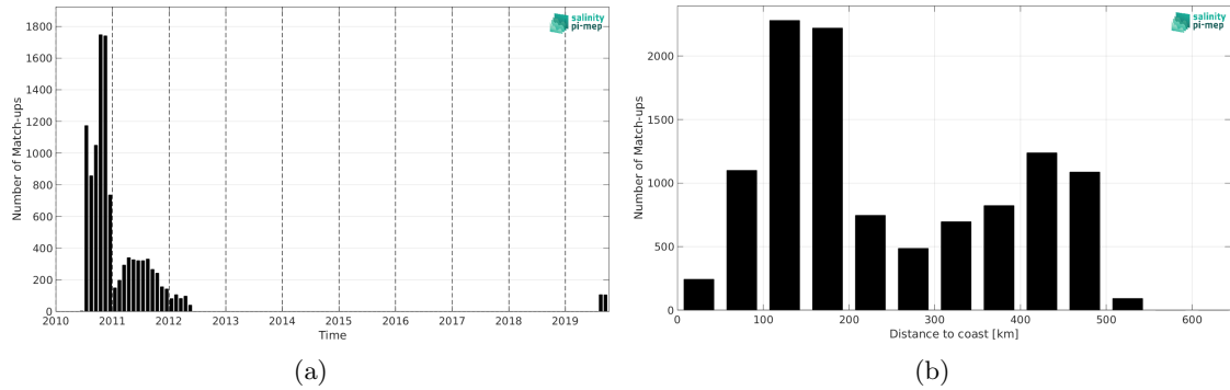
Figure 1: Number of match-ups between Surface drifters and SMOS SSS L3 Arctic v2 - 18 Days (CATDS-CEC-LOCEAN) SSS as a function of time (a) and as function of the distance to coast (b) over the Arctic Ocean Pi-MEP region and for the full satellite product period.
