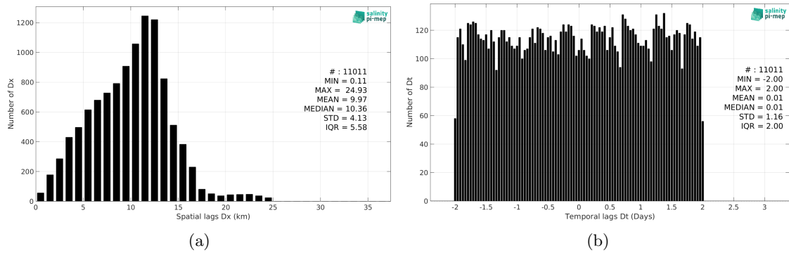
Figure 4: Histograms of the spatial (a) and temporal (b) lags between the location/time of the Surface drifters measurement and the date of the corresponding SMOS SSS L3 Arctic v2 - 18 Days (CATDS-CEC-LOCEAN) SSS pixel.
