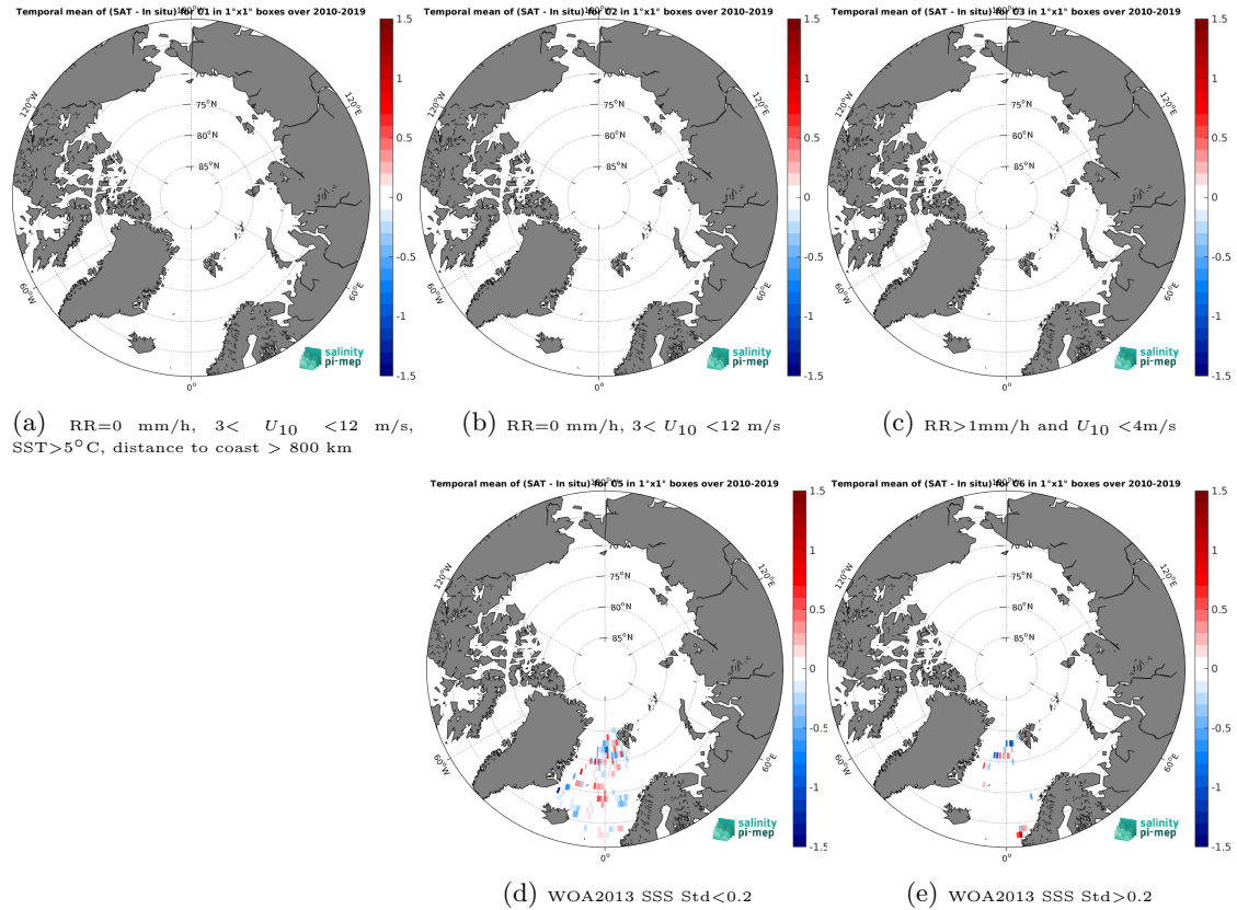
Figure 11: Temporal mean gridded over spatial boxes of size 1^{\circ}\times 1^{\circ} of \Delta\text{SSS} (SMOS SSS L3 Arctic v2 - 18 Days (CATDS-CEC-LOCEAN) - Surface drifters) for 5 different subdatasets corresponding to:RR=0 mm/h, 3 < U_{10} < 12 m/s, SST > 5^{\circ}\text{C} , distance to coast > 800 km (a), RR=0 mm/h, 3 < U_{10} < 12 m/s (b), RR > 1 mm/h and U_{10} < 4 m/s (c), WOA2013 SSS Std < 0.2 (d), WOA2013 SSS Std > 0.2 (e).
