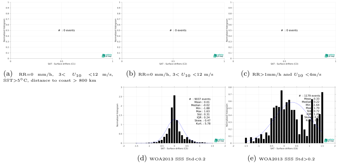
Figure 12: Normalized histogram of \Delta SSS (SMOS SSS L3 Arctic v2 - 18 Days (CATDS-CEC-LOCEAN) - Surface drifters) for 5 different subdatasets corresponding to: RR=0 mm/h, 3 < U_{10} < 12 m/s, SST > 5°C, distance to coast > 800 km (a), RR=0 mm/h, 3 < U_{10} < 12 m/s (b), RR > 1mm/h and U_{10} < 4 m/s (c), WOA2013 SSS Std < 0.2 (d), WOA2013 SSS Std > 0.2 (e).
