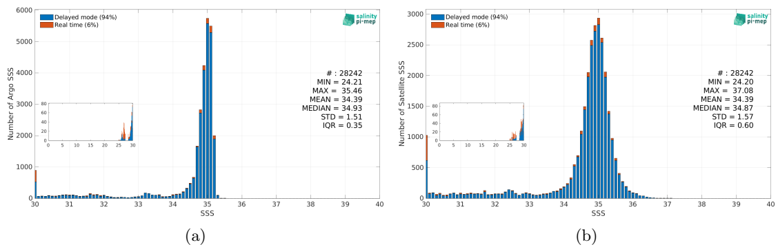
Figure 3: Histograms of SSS from Argo (a) and SMOS SSS L3 Arctic v2 - 18 Days (CATDS-CEC-LOCEAN) (b) considering all match-up pairs per bins of 0.1 over the Arctic Ocean Pi-MEP region and for the full satellite product period.
