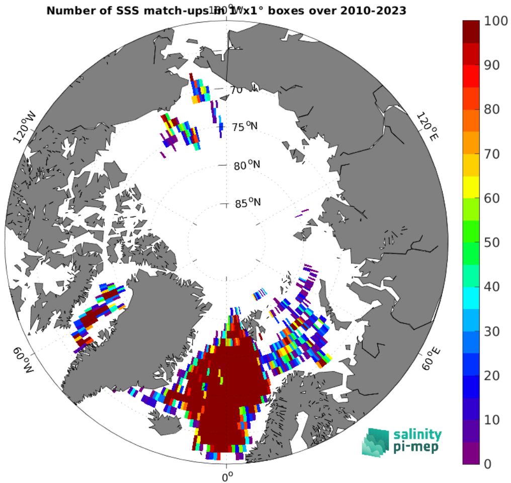
Figure 5: Number of SSS match-ups between Argo SSS and the SMOS SSS L3 Arctic v2 - 18 Days (CATDS-CEC-LOCEAN) SSS product for the Arctic Ocean Pi-MEP region over 1^\circ \times 1^\circ boxes and for the full satellite product period.
