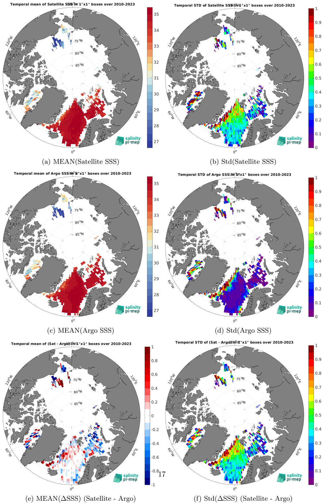
Figure 7: Temporal mean (left) and Std (right) of SSS from SMOS SSS L3 Arctic v2 - 18 Days (CATDS-CEC-LOCEAN) (top), Argo (middle), and of \Delta SSS (Satellite - Argo). Only match-up pairs are used to generate these maps.
