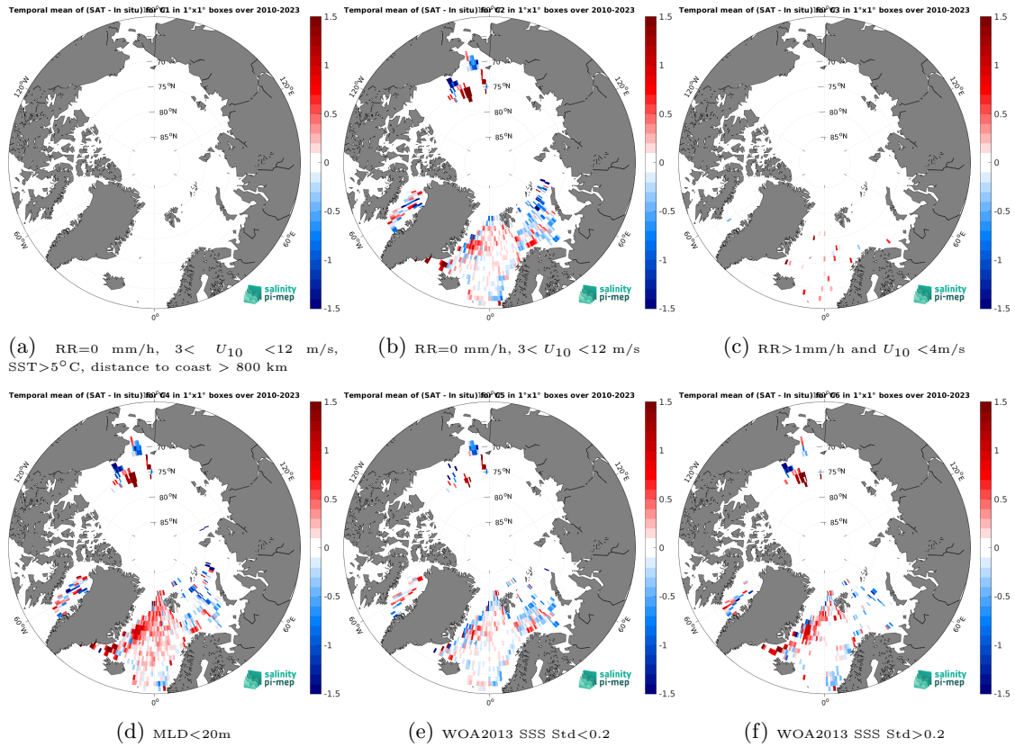
Figure 14: Temporal mean gridded over spatial boxes of size 1^\circ \times 1^\circ of \Delta SSS (SMOS SSS L3 Arctic v2 - 18 Days (CATDS-CEC-LOCEAN) - Argo) for 6 different subdatasets corresponding to:RR=0 mm/h, 3 < U_{10} < 12 m/s, SST>5°C, distance to coast > 800 km (a), RR=0 mm/h, 3 < U_{10} < 12 m/s (b), RR>1mm/h and U_{10} < 4 m/s (c),MLD<20m (d),WOA2013 SSS Std<0.2 (e),WOA2013 SSS Std>0.2 (f).
