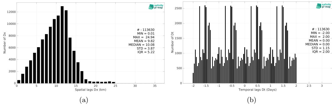
Figure 6: Histograms of the spatial (a) and temporal (b) lags between the location/time of the Argo measurement and the date of the corresponding SMOS SSS L3 Arctic v2 - 18 Days (CATDS-CEC-LOCEAN) SSS pixel.
