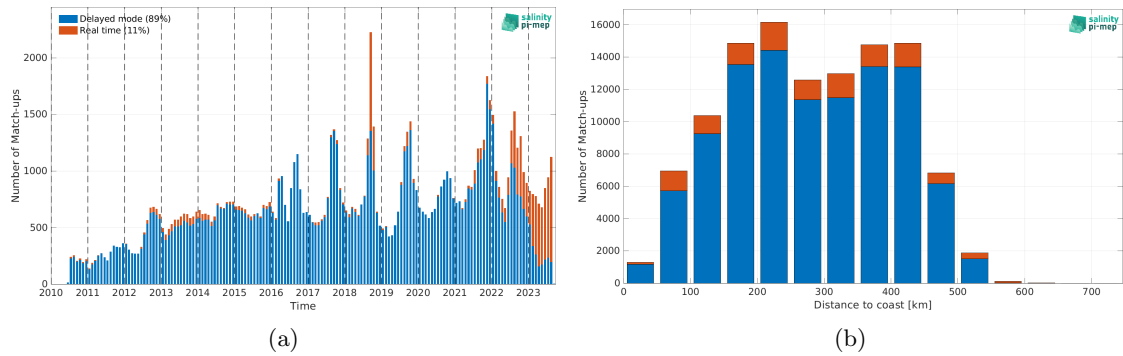
Figure 2: Number of match-ups between Argo and SMOS SSS L3 Arctic v2 - 18 Days (CATDS-CEC-LOCEAN) SSS as a function of time (a) and as function of the distance to coast (b) over the Arctic Ocean Pi-MEP region and for the full satellite product period.
