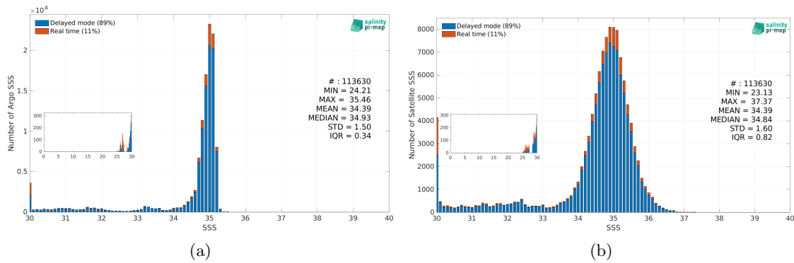
Figure 3: Histograms of SSS from Argo (a) and SMOS SSS L3 Arctic v2 - 18 Days (CATDS-CEC-LOCEAN) (b) considering all match-up pairs per bins of 0.1 over the Arctic Ocean Pi-MEP region and for the full satellite product period.
