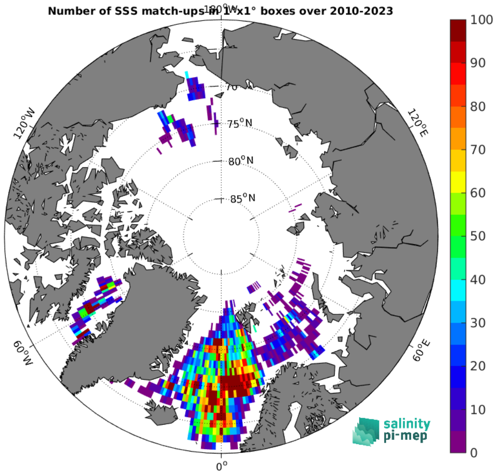
Figure 4: Number of SSS match-ups between Argo SSS and the SMOS SSS L3 Arctic v2 - 18 Days (CATDS-CEC-LOCEAN) SSS product for the Arctic Ocean Pi-MEP region over 1^\circ \times 1^\circ boxes and for the full satellite product period.
