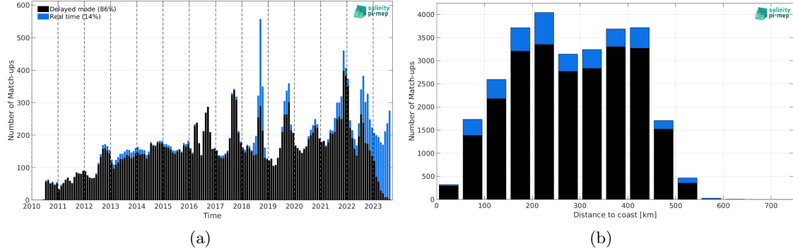
Figure 1: Number of match-ups between Argo and SMOS SSS L3 Arctic v2 - 18 Days (CATDS-CEC-LOCEAN) SSS as a function of time (a) and as function of the distance to coast (b) over the Arctic Ocean Pi-MEP region and for the full satellite product period.
