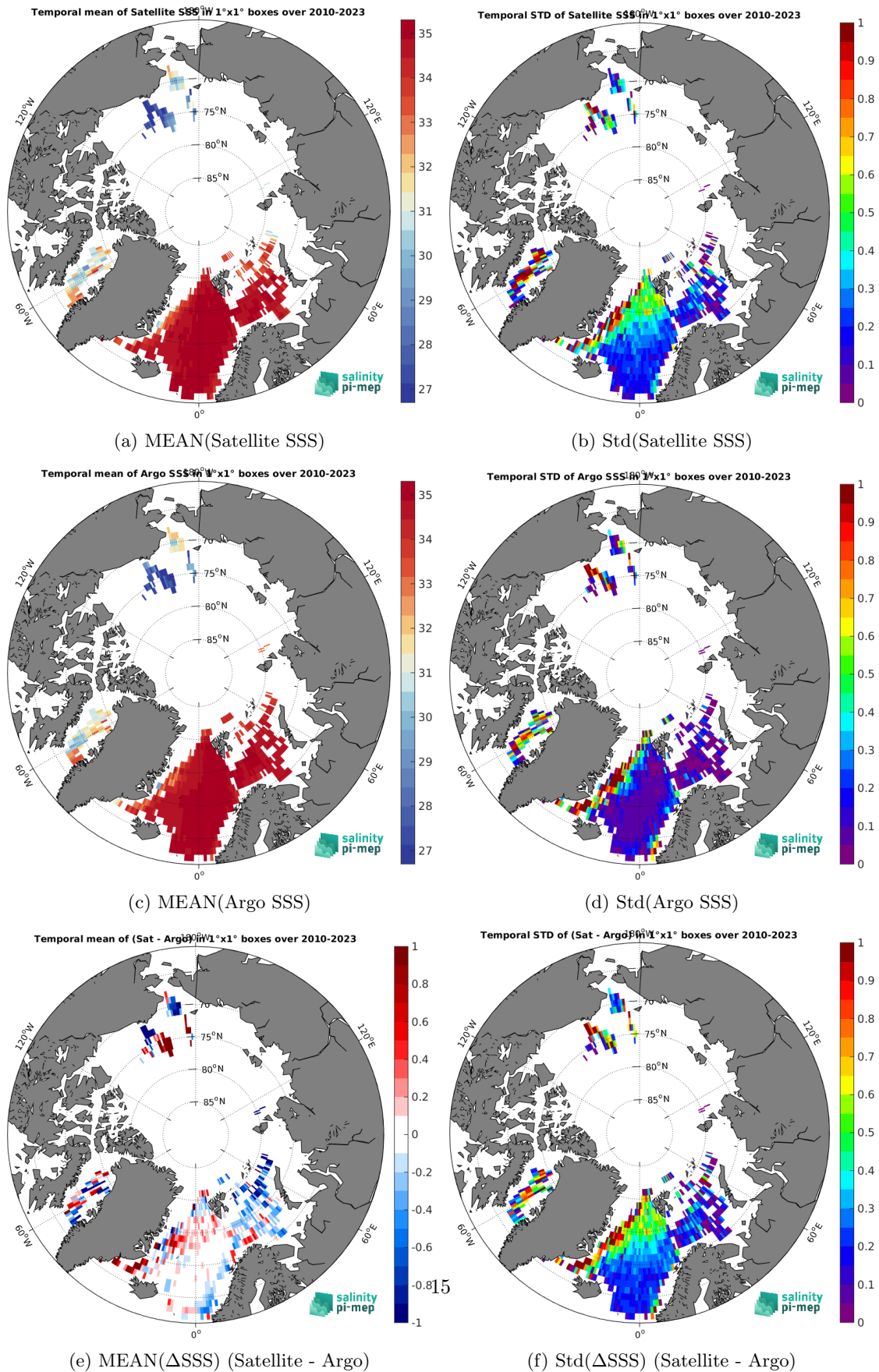
Figure 6: Temporal mean (left) and Std (right) of SSS from SMOS SSS L3 Arctic v2 - 18 Days (CATDS-CEC-LOCEAN) (top), Argo (middle), and of \Delta SSS (Satellite - Argo). Only match-up pairs are used to generate these maps.
