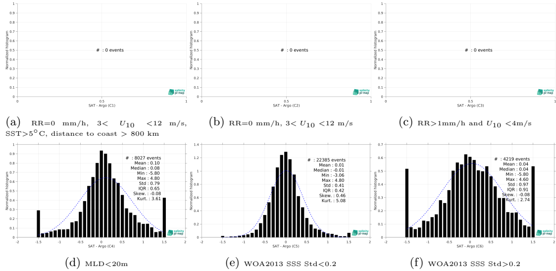
Figure 13: Normalized histogram of \Delta SSS (SMOS SSS L3 Arctic v2 - 18 Days (CATDS-CEC-LOCEAN) - Argo) for 6 different subdatasets corresponding to: RR=0 mm/h, 3 < U_{10} < 12 m/s, SST > 5°C, distance to coast > 800 km (a), RR=0 mm/h, 3 < U_{10} < 12 m/s (b), RR > 1mm/h and U_{10} < 4 m/s (c), MLD < 20m (d), WOA2013 SSS Std < 0.2 (e), WOA2013 SSS Std > 0.2 (f).
