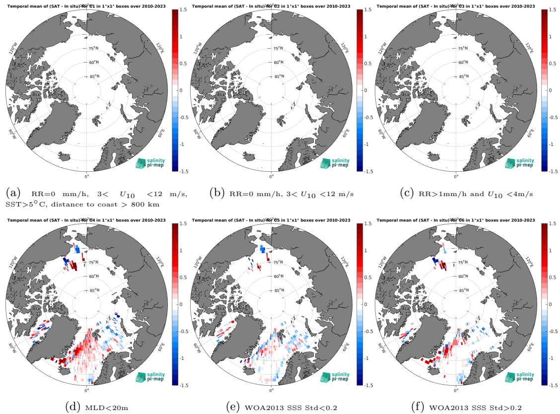
Figure 12: Temporal mean gridded over spatial boxes of size 1^{\circ}\times 1^{\circ} of \Delta\text{SSS} (SMOS SSS L3 Arctic v2 - 18 Days (CATDS-CEC-LOCEAN) - Argo) for 6 different subdatasets corresponding to:RR=0 mm/h, 3 < U_{10} < 12 m/s, SST >5^{\circ}\text{C} , distance to coast > 800 km (a), RR=0 mm/h, 3 < U_{10} < 12 m/s (b), RR >1 mm/h and U_{10} < 4 m/s (c),MLD <20 m (d),WOA2013 SSS Std <0.2 (e),WOA2013 SSS Std >0.2 (f).
