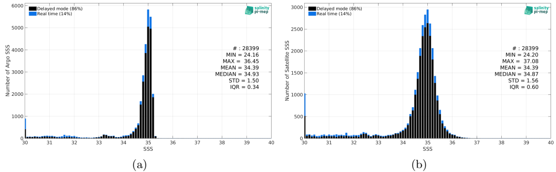
Figure 2: Histograms of SSS from Argo (a) and SMOS SSS L3 Arctic v2 - 18 Days (CATDS-CEC-LOCEAN) (b) considering all match-up pairs per bins of 0.1 over the Arctic Ocean Pi-MEP region and for the full satellite product period.
